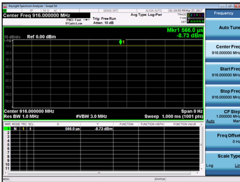
Frequency 916MHz
