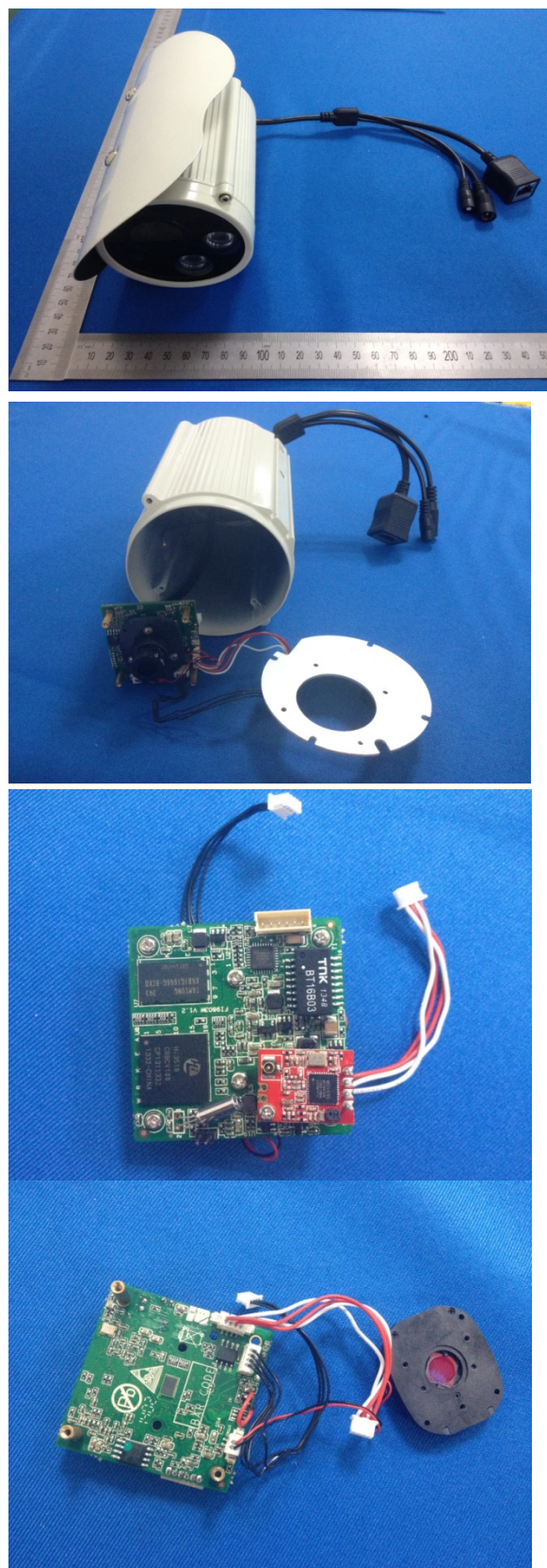
Model 2:FC5413P
