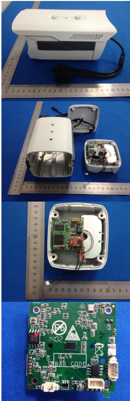
Model 1:FC5412P
