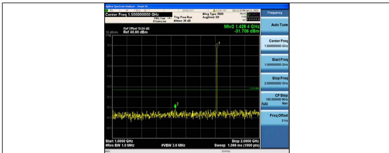
Band4-1.4MHz-16QAM-19957-1RB#0-Range5:2000~20000MHz
