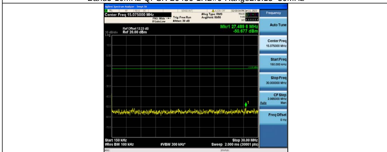
Band5-10MHz-QPSK-20450-1RB#0-Range3:30~1000MHz
