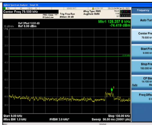
Band5-4132-2-0.009~0.15MHz
