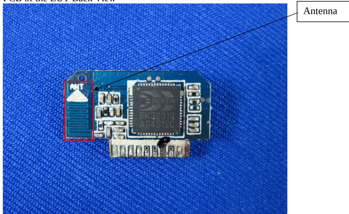
Figure 14 PCB of the EUT-Back View
