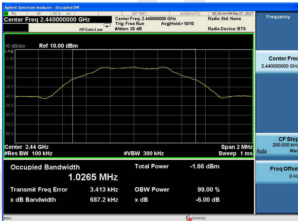
CH: Middle
