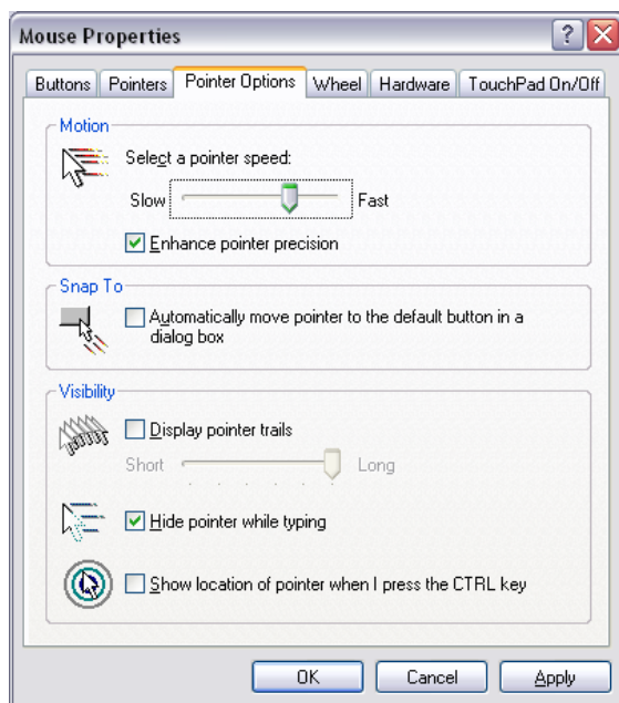
Windows®
