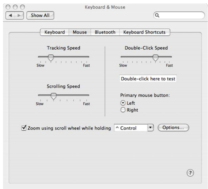
Mac®
