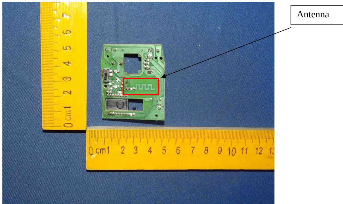
Figure 11 PCB of the EUT-Back View
