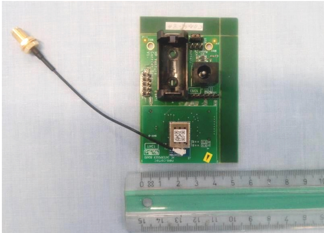
EUT on support board, front
