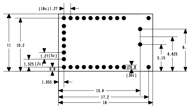
Figure 4: Module footprint (top-view)
