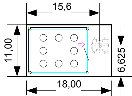
Figure 2: Module drawing
