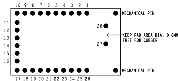
Figure 3: Module pin-out (top-view)
