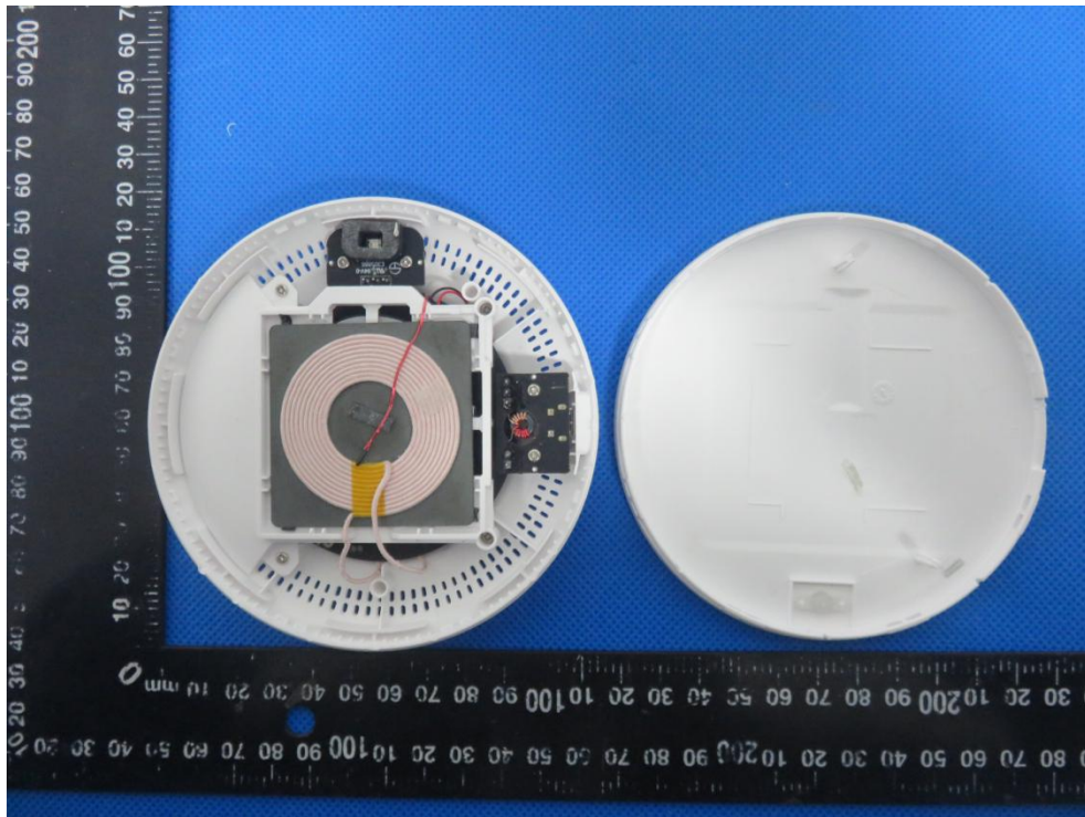
Loop Antenna
