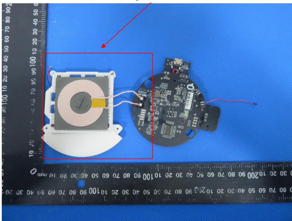
Loop Antenna
