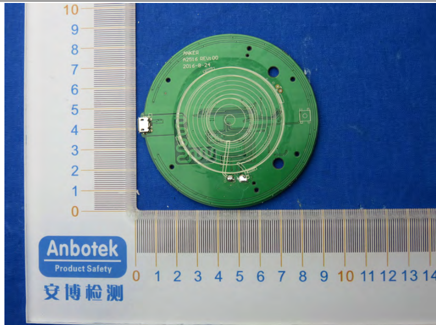
PCB of the EUT-Back View (2)
