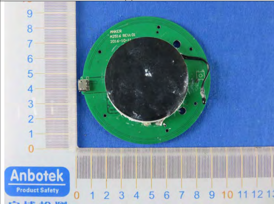
3. Figure PCB of the EUT-Back View (1)
