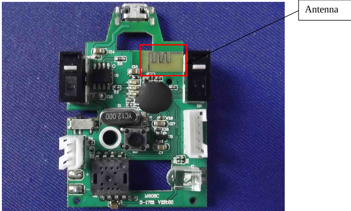
Figure 12 PCB of the EUT-Module View
