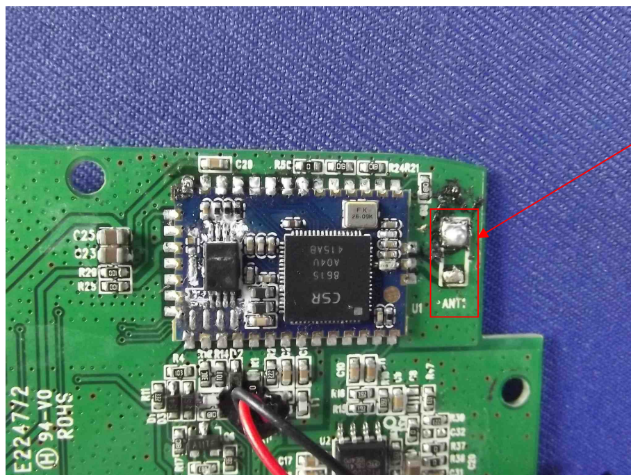
PCB of the EUT-Module View
