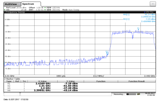
CH03-Bandedge
