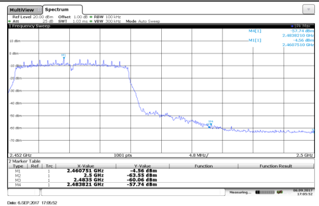
CH11-Bandedge
