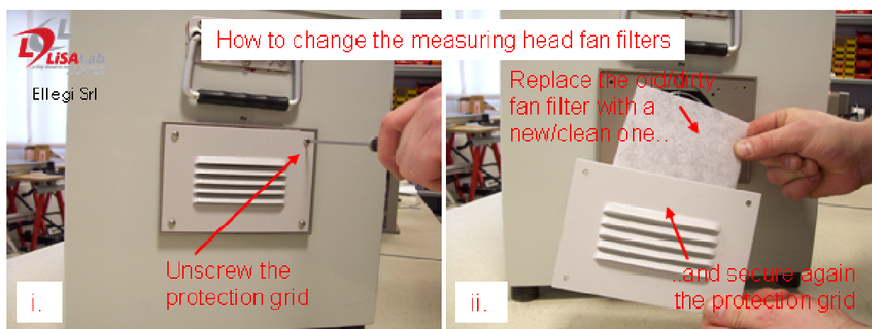
Figure 17: Changing the fan filter of the power base.
