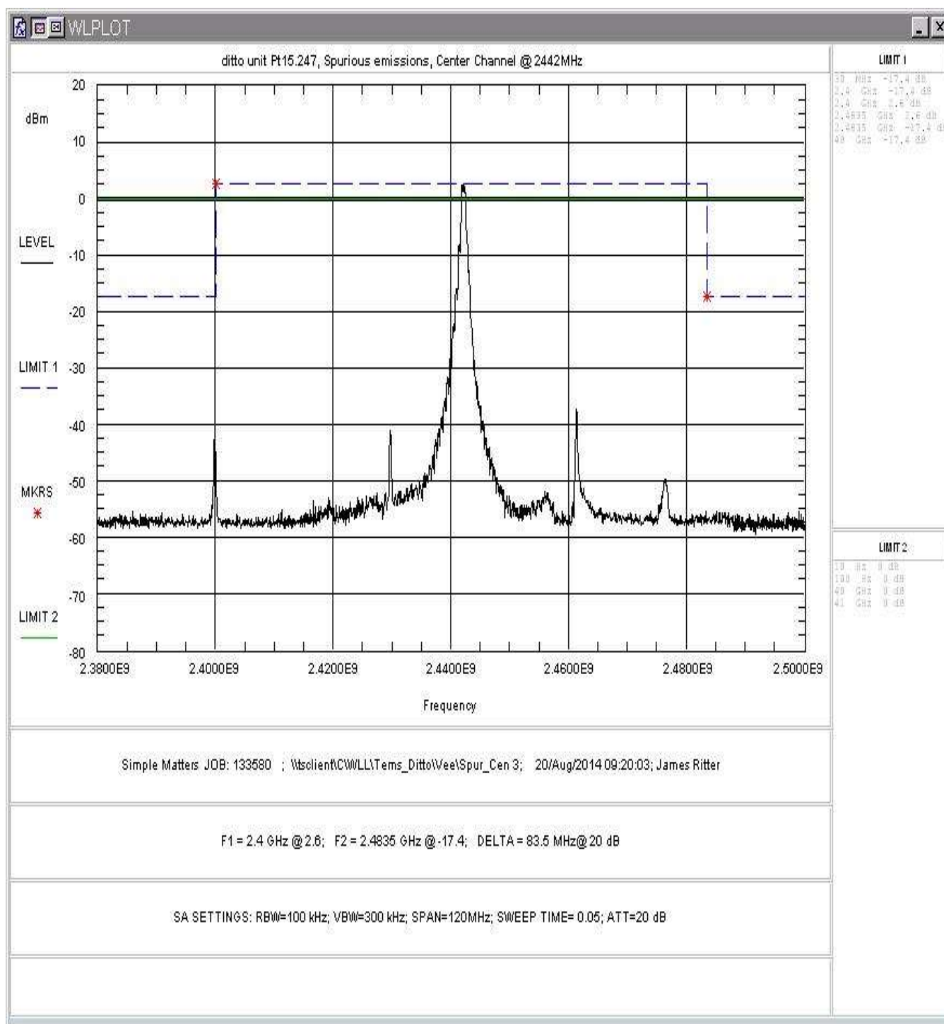
Figure 20: Conducted Spurious Emissions, Center Channel 2.38 – 2.5GHz
