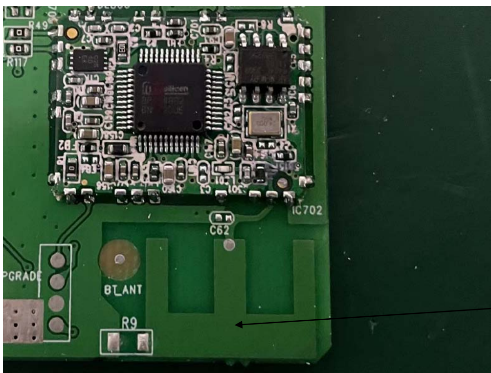
Bluetooth antenna
