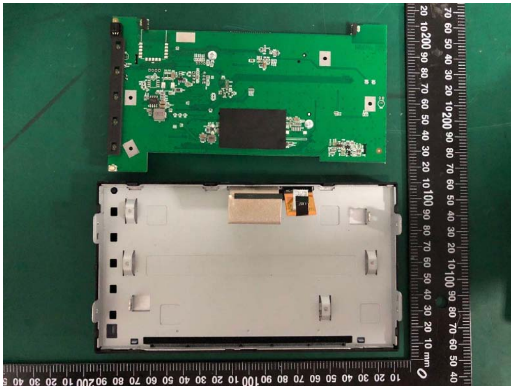
Internal photos M/N: DDX5707S
