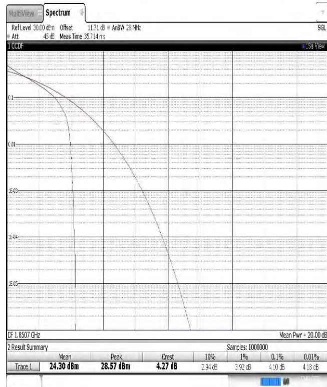
Band2-1.4MHz-QPSK-18607-1RB#0
