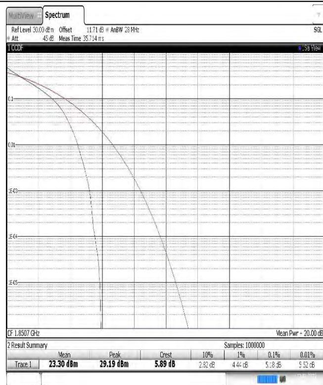
Band2-1.4MHz-QPSK-18607-6RB#0
