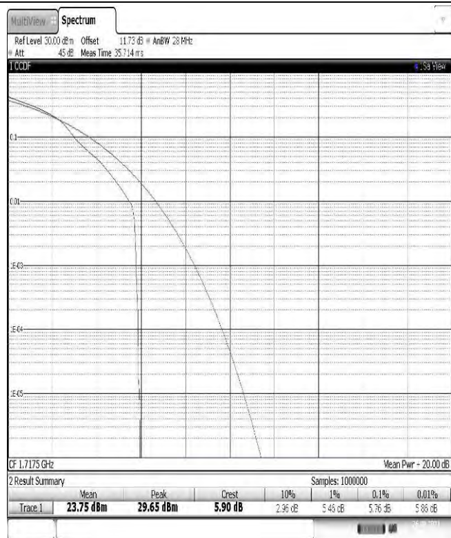
Band66-15MHz-16QAM-132047-75RB#0
