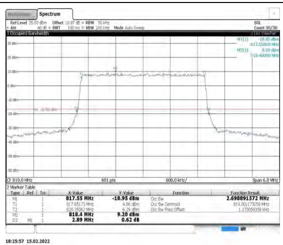
Band26-3MHz-16QAM-26740-15RB#0
