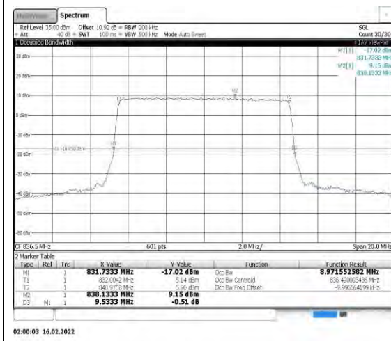
Band26-10MHz-QPSK-26915-50RB#0
