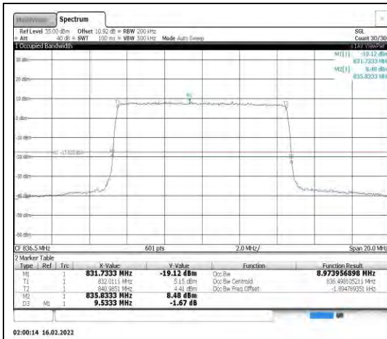
Band26-10MHz-16QAM-26915-50RB#0
