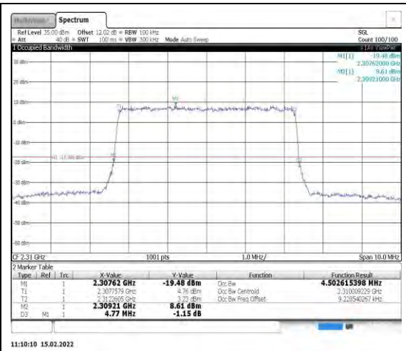
Band40-5MHz-16QAM-38750-25RB#0
