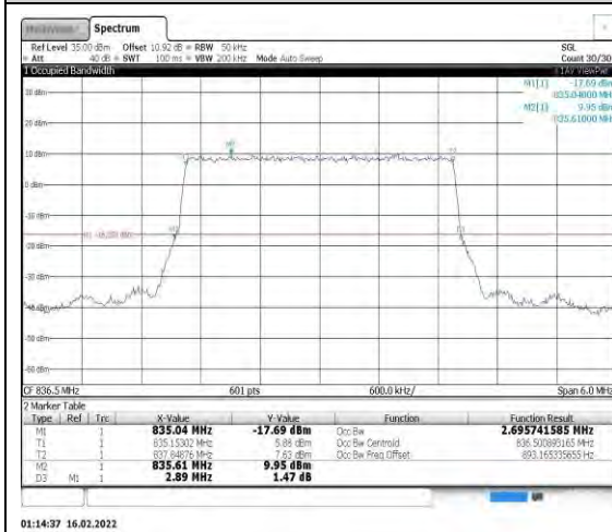
Band26-3MHz-QPSK-26915-15RB#0
