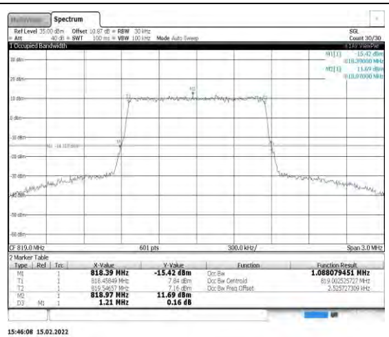
Band26-1.4MHz-16QAM-26740-6RB#0
