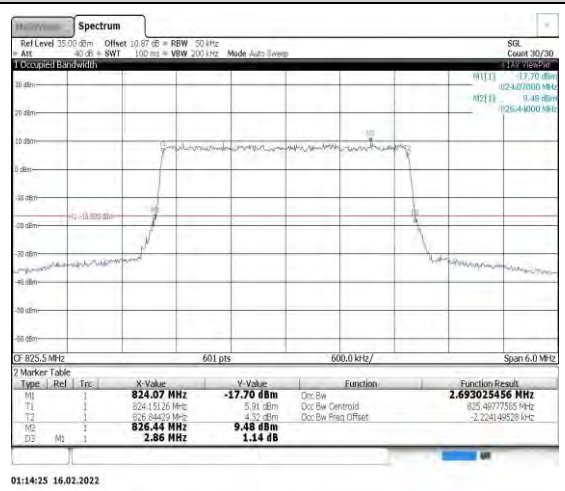
Band26-3MHz-16QAM-26805-15RB#0
