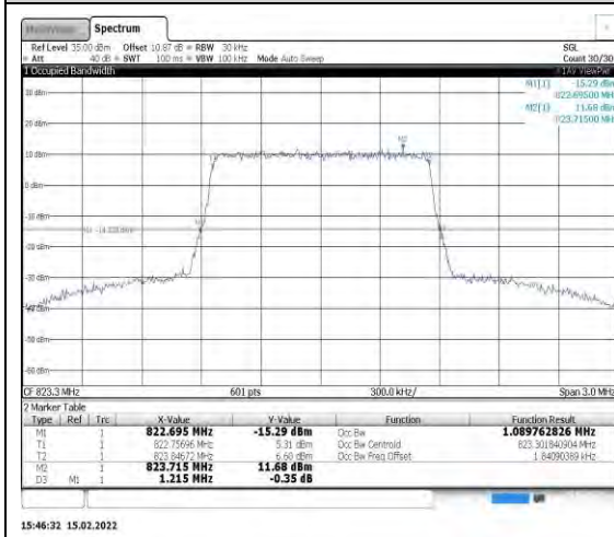
Band26-1.4MHz-16QAM-26783-6RB#0
