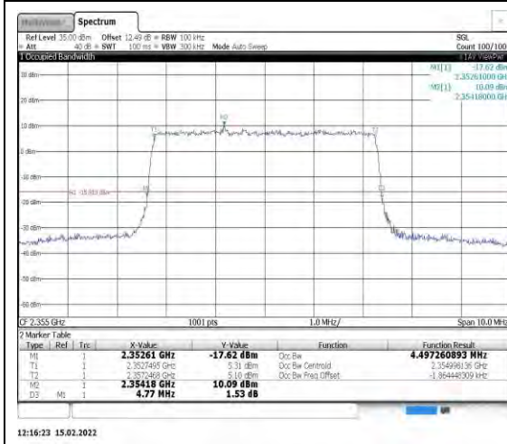
Band40-5MHz-16QAM-39200-25RB#0
