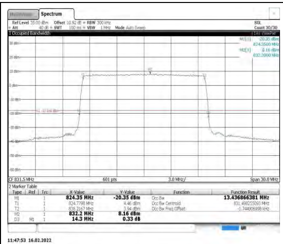
Band26-15MHz-16QAM-26865-75RB#0
