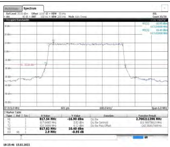
Band26-3MHz-QPSK-26740-15RB#0
