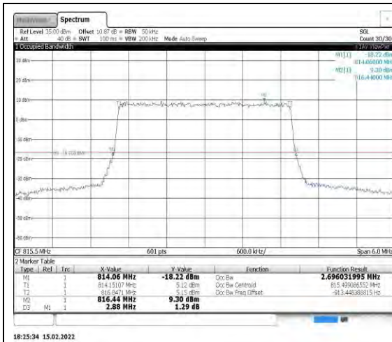
Band26-3MHz-16QAM-26705-15RB#0
