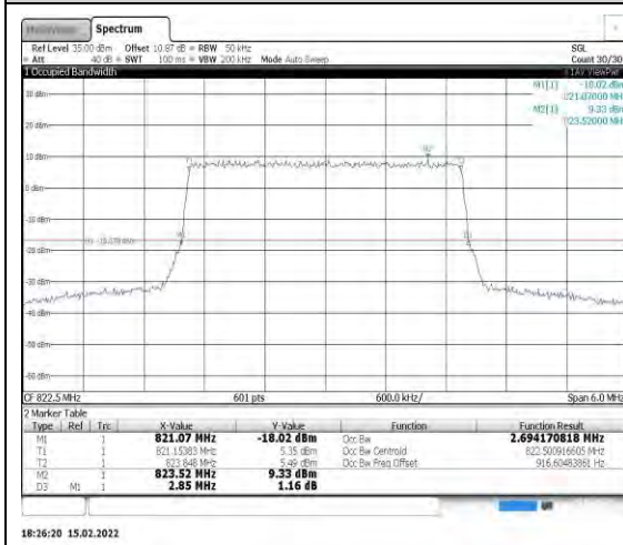
Band26-3MHz-16QAM-26775-15RB#0
