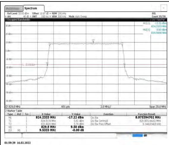
Band26-10MHz-QPSK-26840-50RB#0
