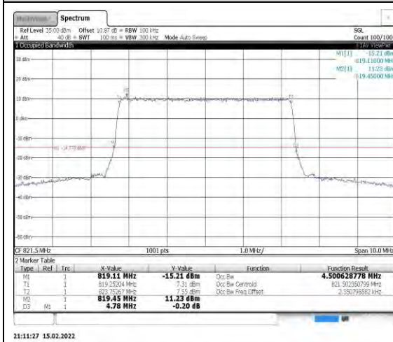
Band26-5MHz-QPSK-26765-25RB#0
