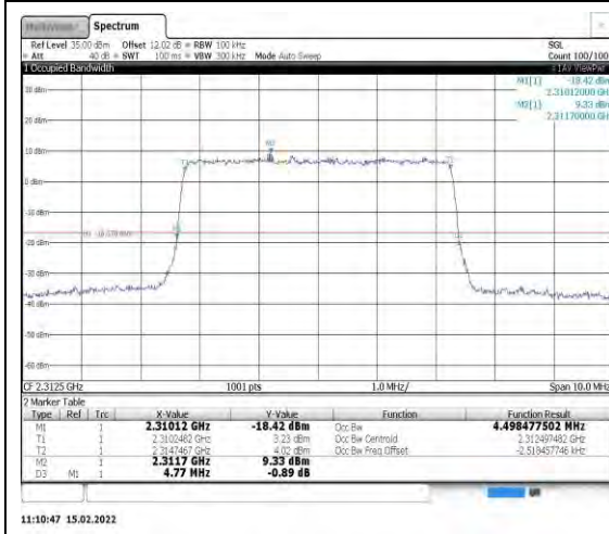
Band40-5MHz-16QAM-38775-25RB#0
