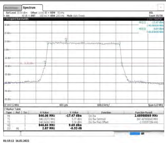
Band26-3MHz-16QAM-27025-15RB#0
