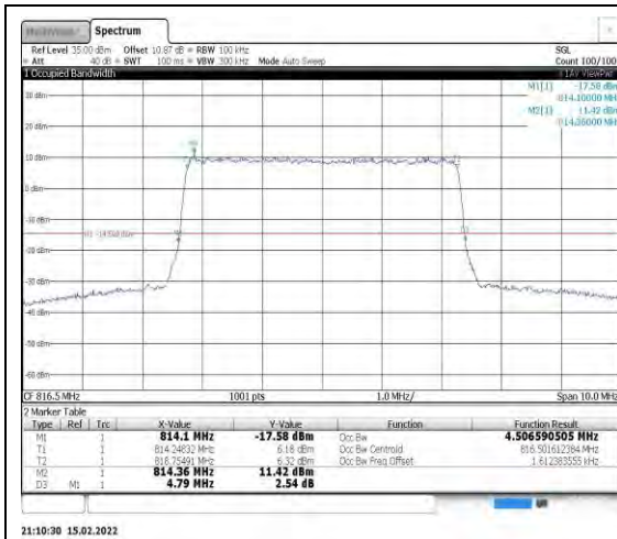
Band26-5MHz-16QAM-26715-25RB#0
