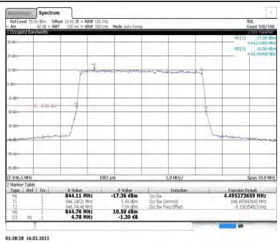
Band26-5MHz-16QAM-27015-25RB#0
