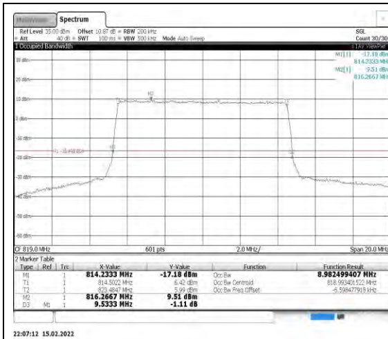
Band26-10MHz-QPSK-26740-50RB#0
