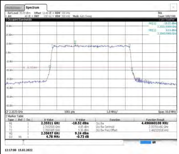
Band40-5MHz-16QAM-39225-25RB#0
