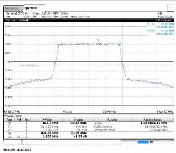
Band26-1.4MHz-16QAM-26797-6RB#0
