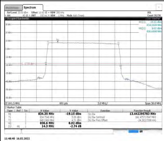
Band26-15MHz-16QAM-26965-75RB#0
