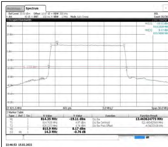
Band26-15MHz-16QAM-26765-75RB#0
