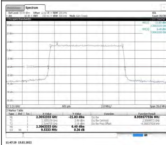
Band40-10MHz-16QAM-38750-50RB#0
