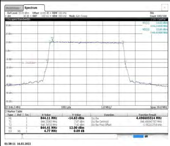
Band26-5MHz-QPSK-27015-25RB#0
