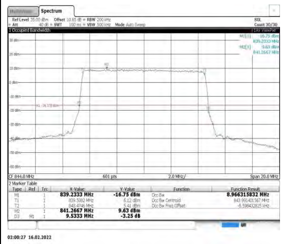
Band26-10MHz-QPSK-26990-50RB#0
