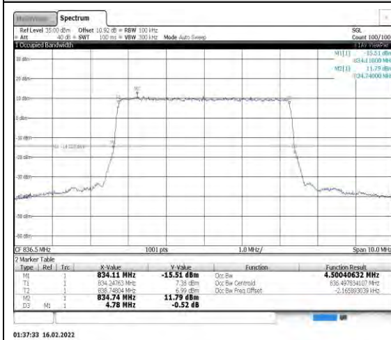
Band26-5MHz-QPSK-26915-25RB#0
