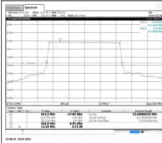
Band26-15MHz-QPSK-26765-75RB#0
