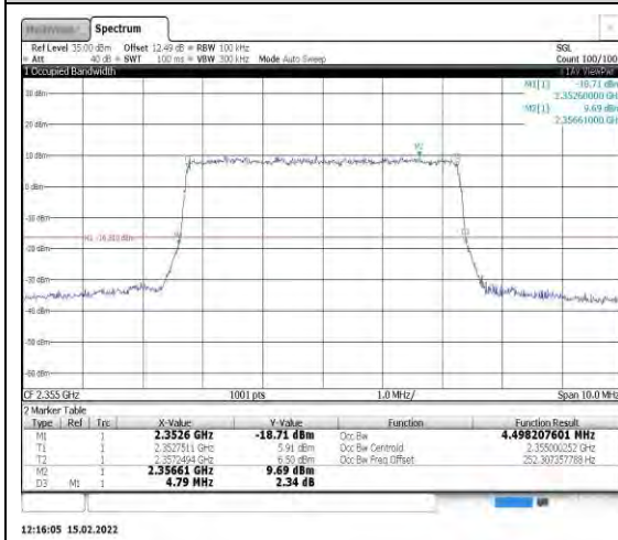
Band40-5MHz-QPSK-39200-25RB#0
