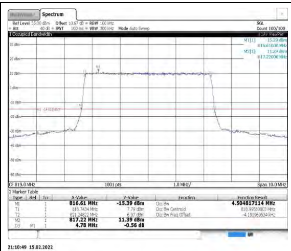
Band26-5MHz-QPSK-26740-25RB#0
