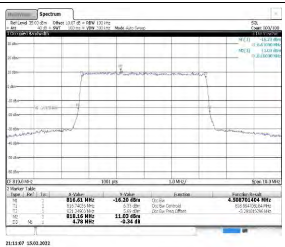
Band26-5MHz-16QAM-26740-25RB#0
