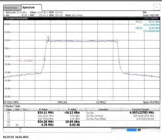
Band26-5MHz-16QAM-26815-25RB#0
