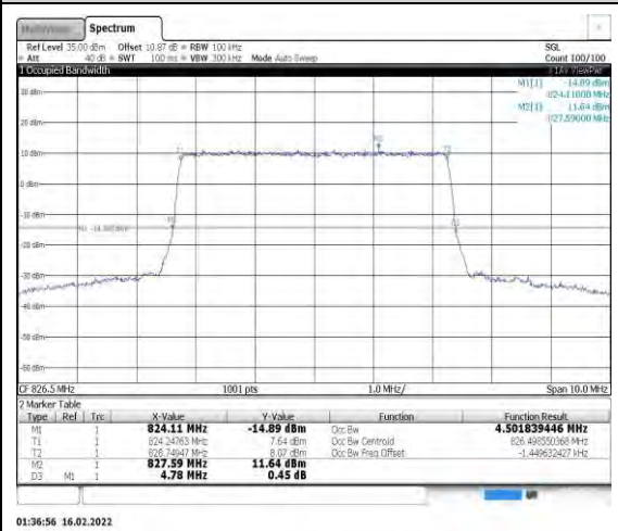
Band26-5MHz-QPSK-26815-25RB#0
