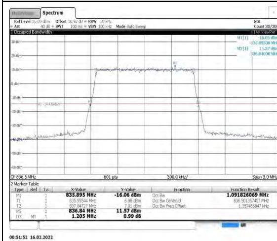
Band26-1.4MHz-16QAM-26915-6RB#0
