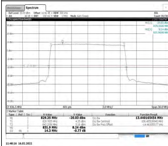
Band26-15MHz-16QAM-26915-75RB#0
