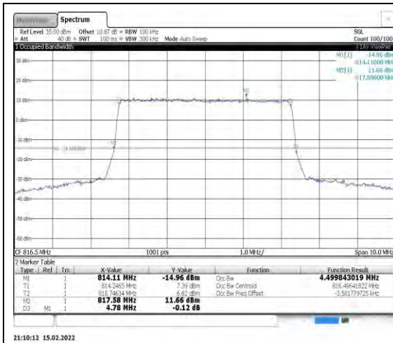
Band26-5MHz-QPSK-26715-25RB#0
