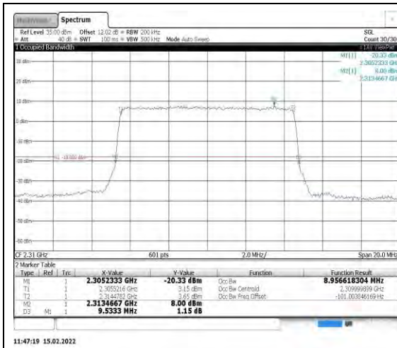
Band40-10MHz-QPSK-38750-50RB#0
