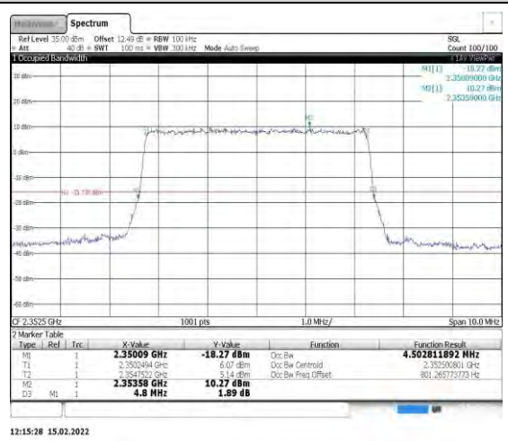
Band40-5MHz-QPSK-39175-25RB#0
