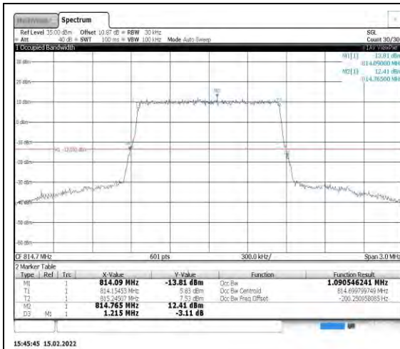
Band26-1.4MHz-16QAM-26697-6RB#0
