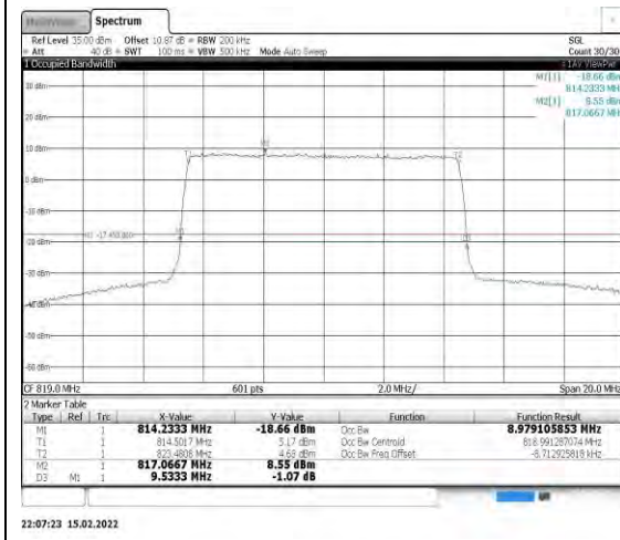
Band26-10MHz-16QAM-26740-50RB#0
