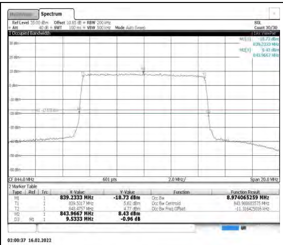
Band26-10MHz-16QAM-26990-50RB#0
