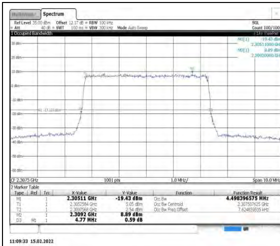
Band40-5MHz-16QAM-38725-25RB#0
