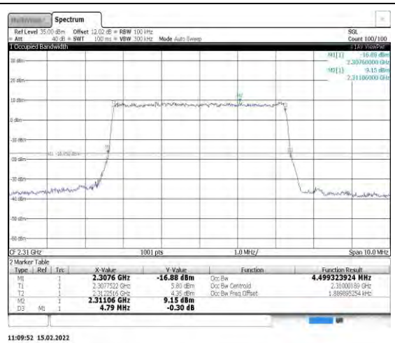
Band40-5MHz-QPSK-38750-25RB#0
