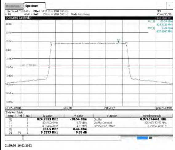
Band26-10MHz-16QAM-26840-50RB#0
