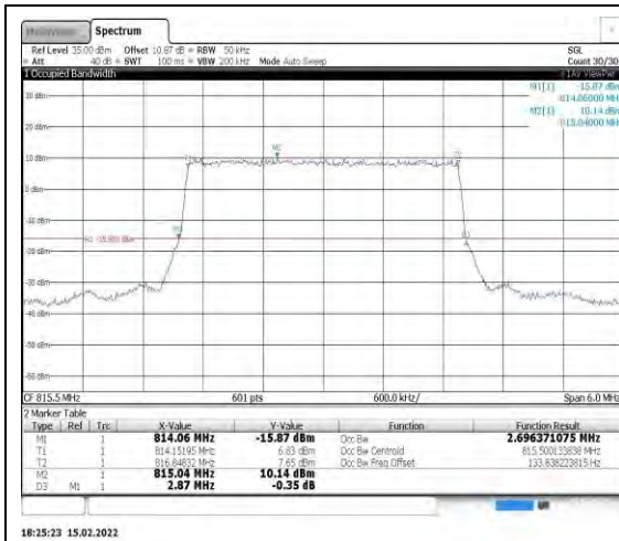
Band26-3MHz-QPSK-26705-15RB#0
