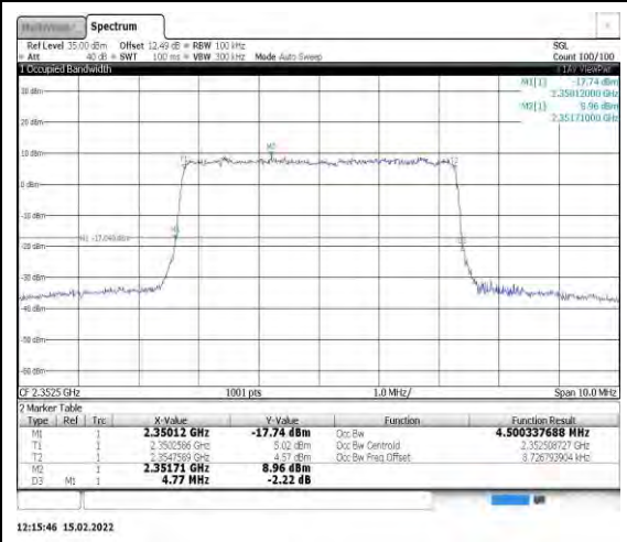
Band40-5MHz-16QAM-39175-25RB#0
