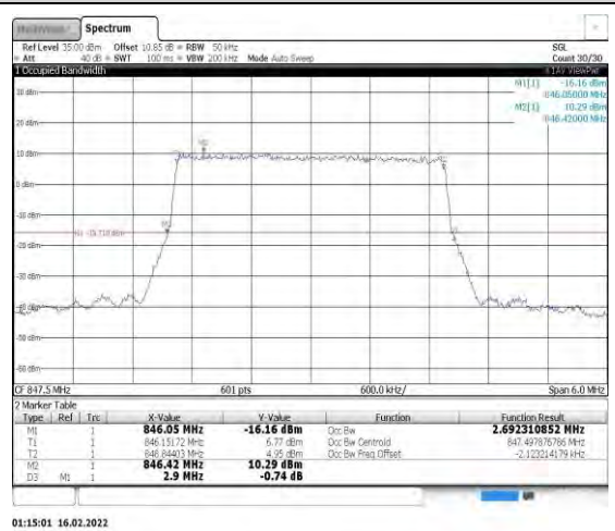
Band26-3MHz-QPSK-27025-15RB#0
