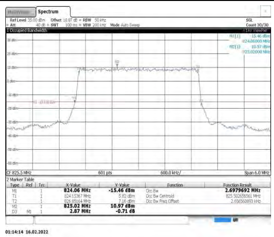
Band26-3MHz-QPSK-26805-15RB#0
