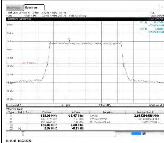
Band26-3MHz-16QAM-26915-15RB#0
