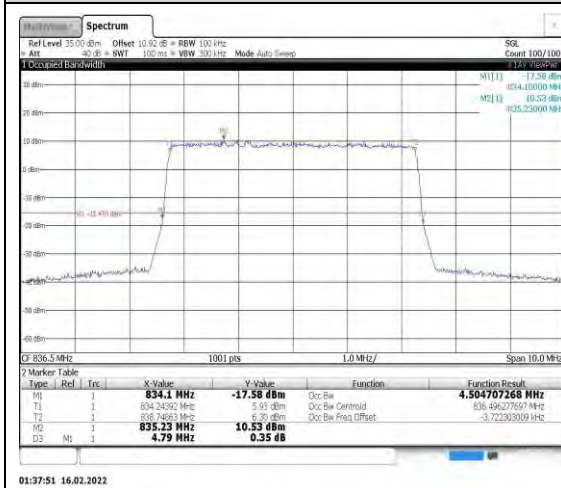
Band26-5MHz-16QAM-26915-25RB#0
