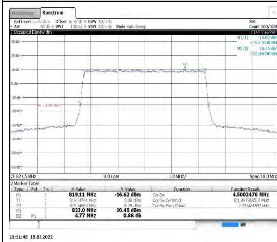
Band26-5MHz-16QAM-26765-25RB#0
