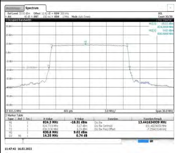
Band26-15MHz-QPSK-26865-75RB#0
