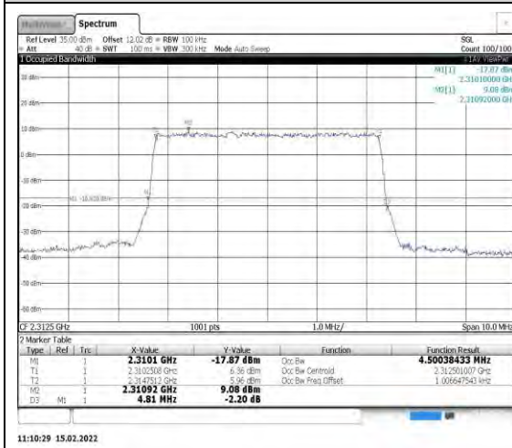
Band40-5MHz-QPSK-38775-25RB#0
