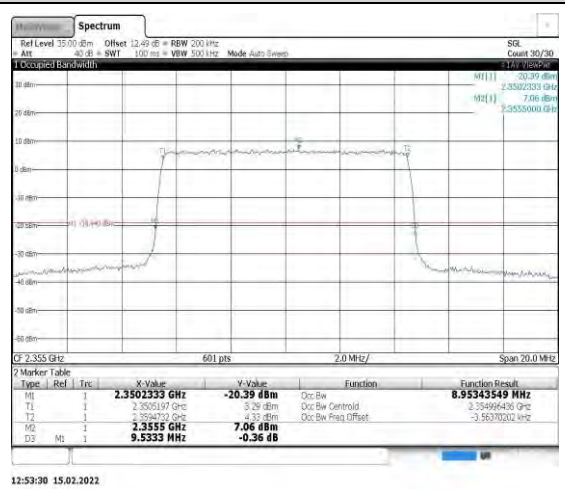
Band40-10MHz-16QAM-39200-50RB#0
