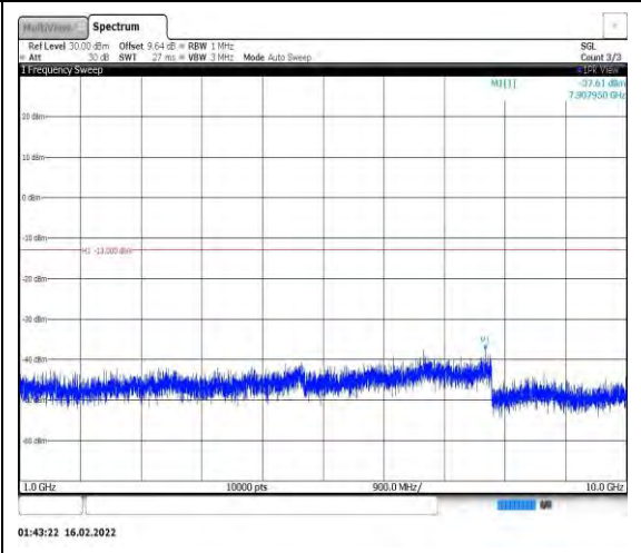
Band26-5MHz-16QAM-26915-1RB#0- Range2:1000~10000MHz
