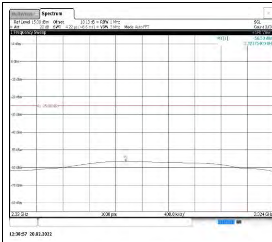
Band40-5MHz-QPSK-38725-1RB#0- Range7:2320~2324MHz
