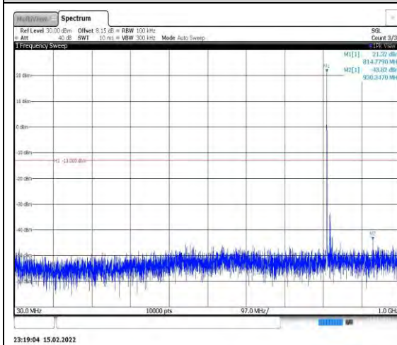
Band26-15MHz-QPSK-26765-1RB#0- Range1:30~1000MHz
