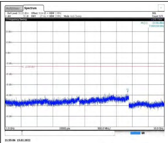
Band26-5MHz-16QAM-26715-1RB#0- Range2:1000~10000MHz
