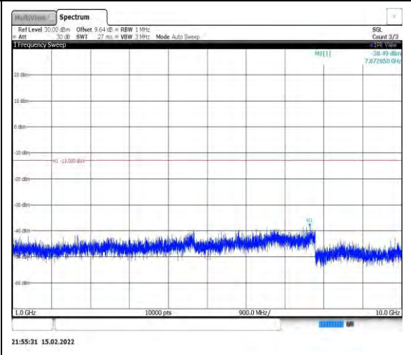
Band26-5MHz-QPSK-26740-1RB#0- Range2:1000~10000MHz
