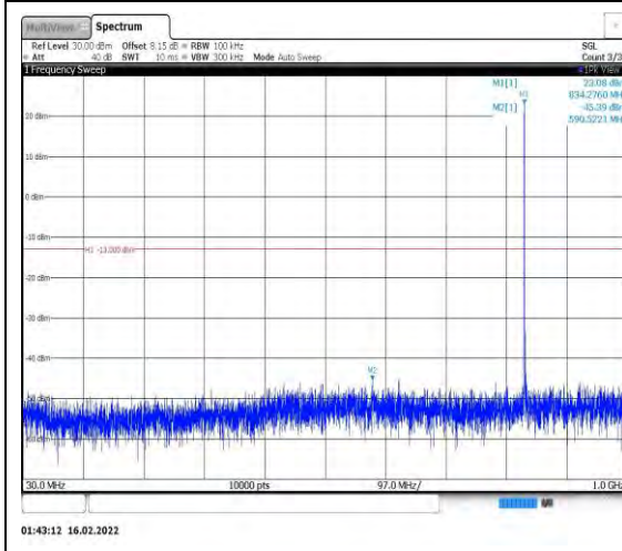
Band26-5MHz-16QAM-26915-1RB#0- Range1:30~1000MHz
