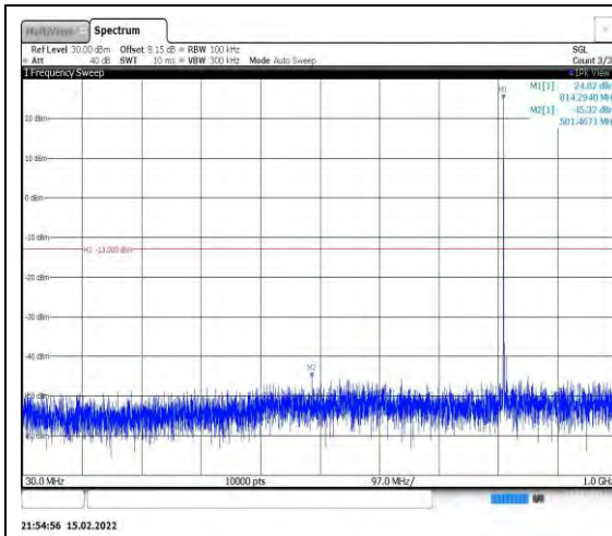
Band26-5MHz-16QAM-26715-1RB#0- Range1:30~1000MHz
