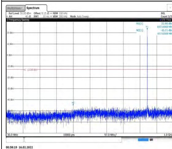
Band26-1.4MHz-QPSK-27033-1RB#0- Range1:30~1000MHz
