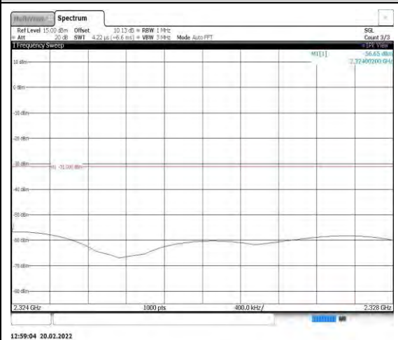
Band40-5MHz-QPSK-39200-1RB#0- Range8:2324~2328MHz
