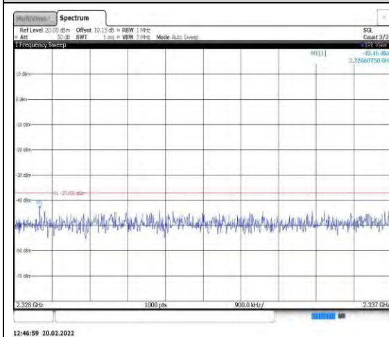
Band40-5MHz-QPSK-38775-1RB#0- Range9:2328~2337MHz
