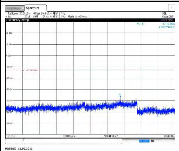
Band26-1.4MHz-16QAM-27033-1RB#0- Range2:1000~10000MHz
