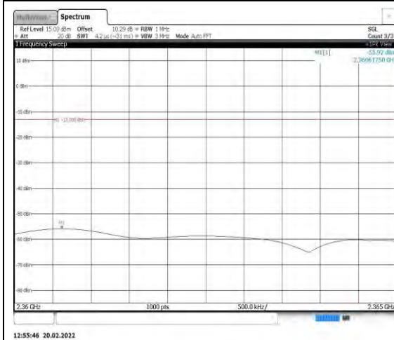
Band40-5MHz-QPSK-39175-1RB#0- Range12:2360~2365MHz
