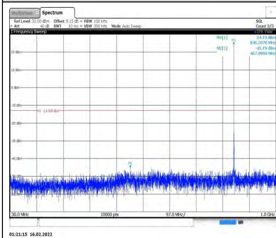
Band26-3MHz-16QAM-27025-1RB#0- Range1:30~1000MHz
