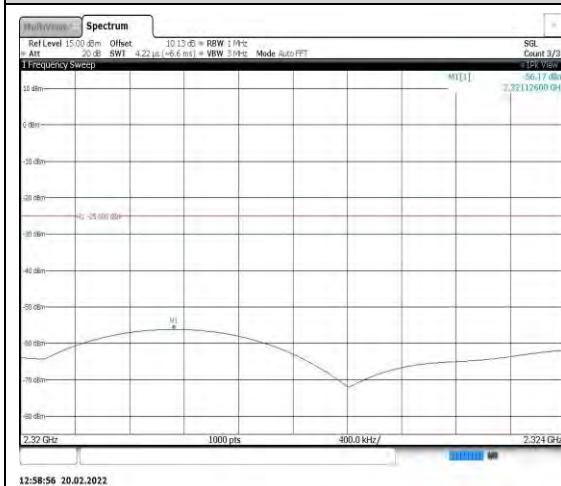
Band40-5MHz-QPSK-39200-1RB#0- Range7:2320~2324MHz
