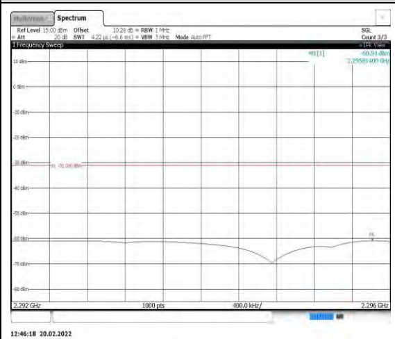
Band40-5MHz-QPSK-38775-1RB#0- Range4:2292~2296MHz
