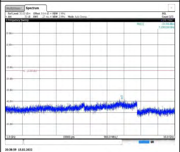
Band26-3MHz-16QAM-26775-1RB#0- Range2:1000~10000MHz
