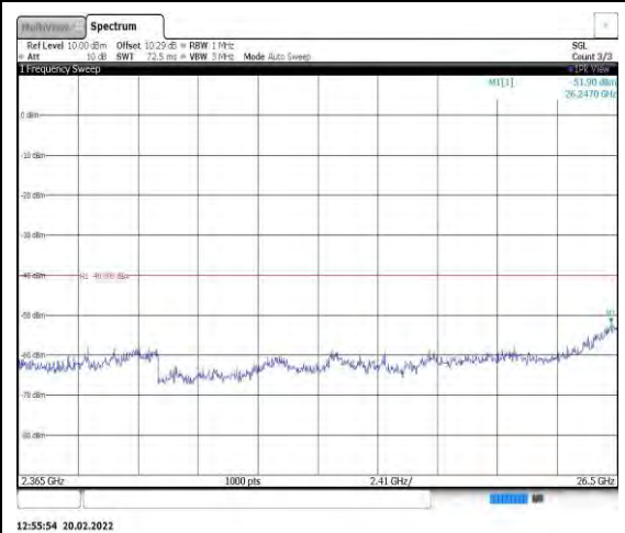
Band40-5MHz-QPSK-39175-1RB#0- Range13:2365~26500MHz
