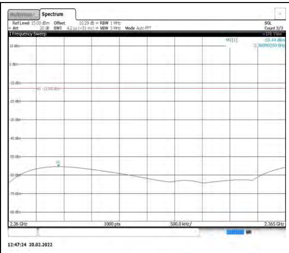
Band40-5MHz-QPSK-38775-1RB#0- Range12:2360~2365MHz
