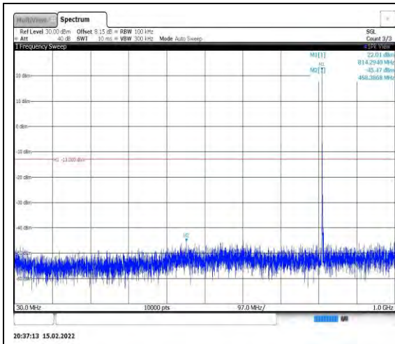
Band26-3MHz-16QAM-26705-1RB#0- Range1:30~1000MHz
