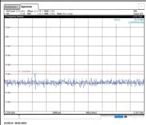
Band40-5MHz-QPSK-39175-1RB#0- Range9:2328~2337MHz
