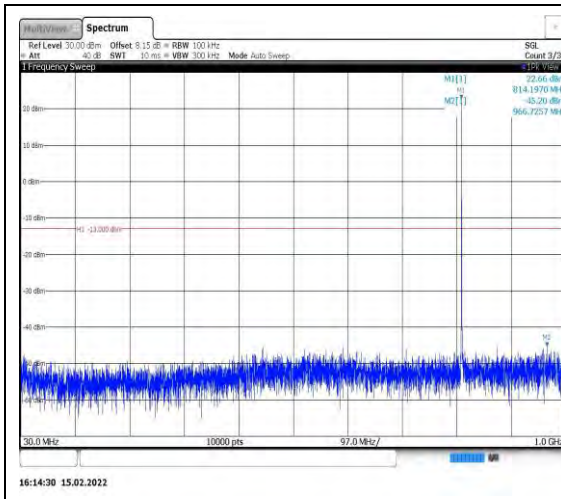
Band26-1.4MHz-16QAM-26697-1RB#0- Range1:30~1000MHz
