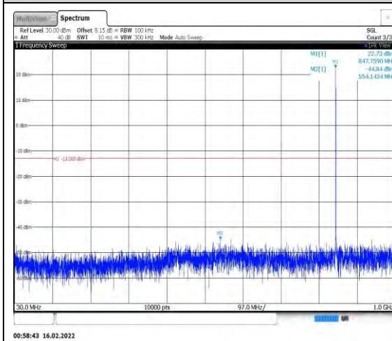
Band26-1.4MHz-16QAM-27033-1RB#0- Range1:30~1000MHz
