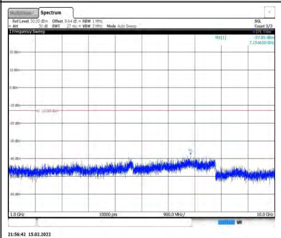
Band26-5MHz-16QAM-26765-1RB#0- Range2:1000~10000MHz
