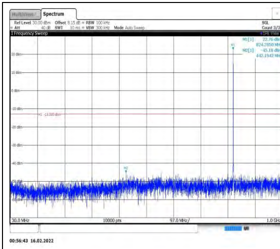
Band26-1.4MHz-QPSK-26797-1RB#0- Range1:30~1000MHz
