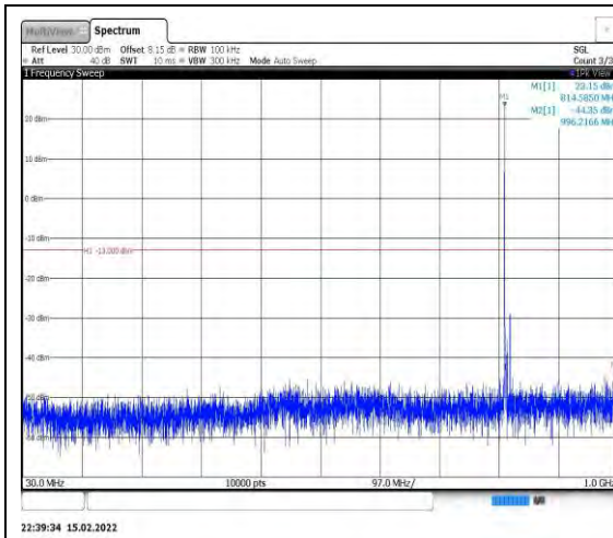
Band26-10MHz-QPSK-26740-1RB#0- Range1:30~1000MHz
