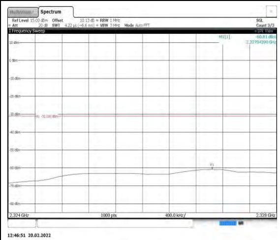
Band40-5MHz-QPSK-38775-1RB#0- Range8:2324~2328MHz
