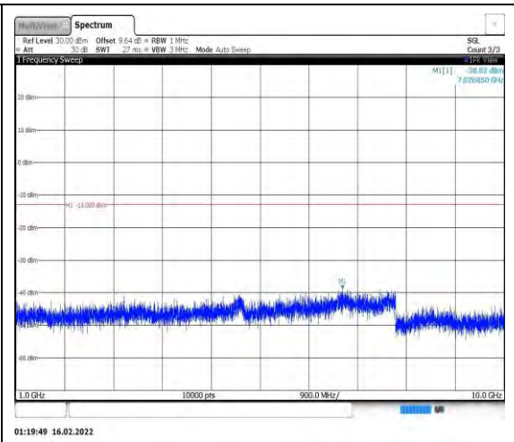
Band26-3MHz-16QAM-26805-1RB#0- Range2:1000~10000MHz
