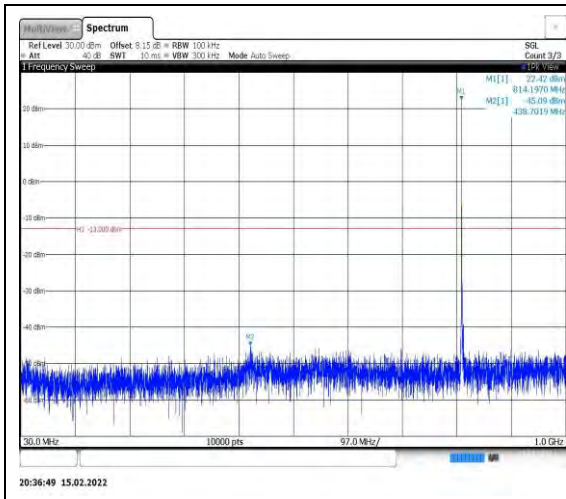
Band26-3MHz-QPSK-26705-1RB#0- Range1:30~1000MHz
