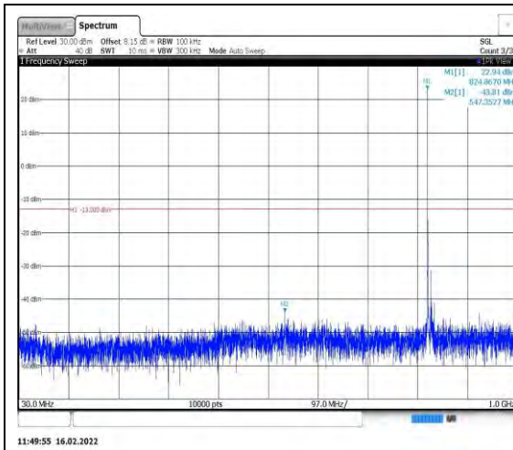
Band26-15MHz-QPSK-26865-1RB#0- Range1:30~1000MHz
