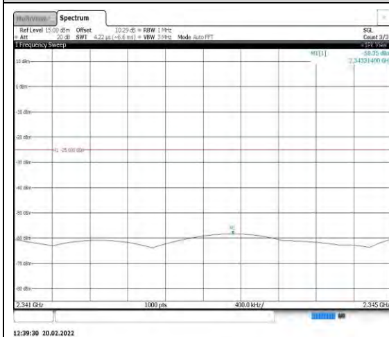
Band40-5MHz-QPSK-38725-1RB#0- Range11:2341~2345MHz
