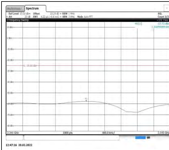
Band40-5MHz-QPSK-38775-1RB#0- Range11:2341~2345MHz
