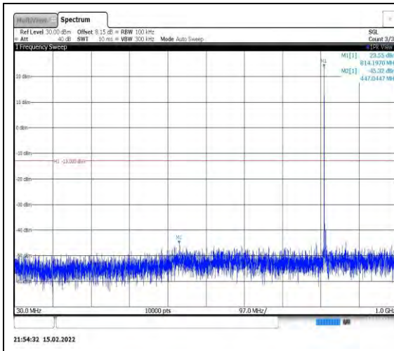
Band26-5MHz-QPSK-26715-1RB#0- Range1:30~1000MHz
