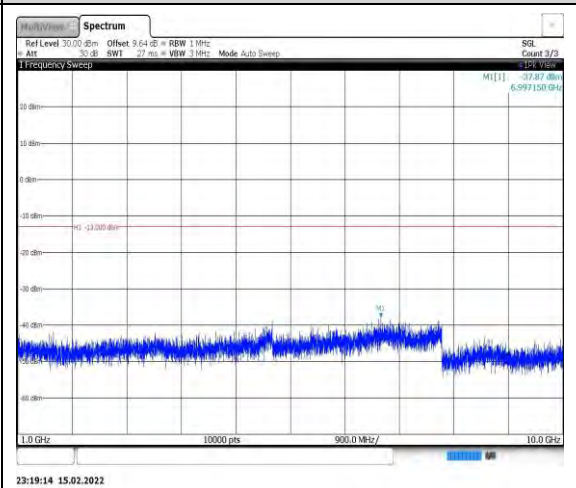
Band26-15MHz-QPSK-26765-1RB#0- Range2:1000~10000MHz
