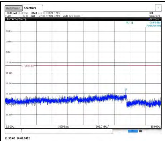
Band26-15MHz-QPSK-26865-1RB#0- Range2:1000~10000MHz
