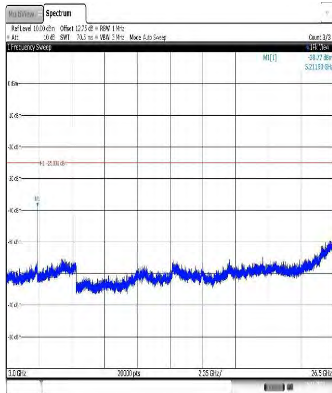
Band38-15MHz-16QAM-38175-1RB#0-Range3:3000~26500MHz
