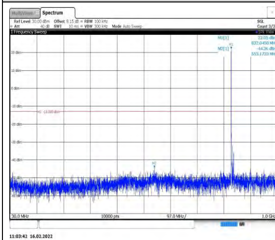
Band26-10MHz-QPSK-26915-1RB#0- Range1:30~1000MHz
