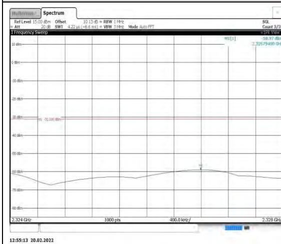
Band40-5MHz-QPSK-39175-1RB#0- Range8:2324~2328MHz
