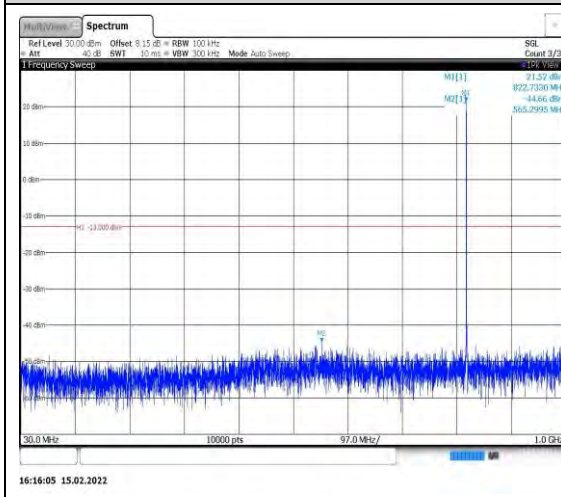
Band26-1.4MHz-16QAM-26783-1RB#0- Range1:30~1000MHz
