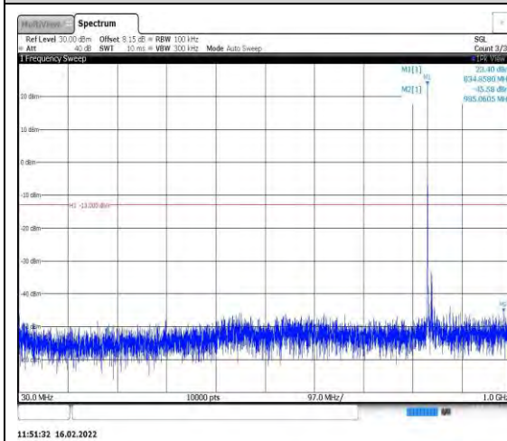
Band26-15MHz-QPSK-26965-1RB#0- Range1:30~1000MHz
