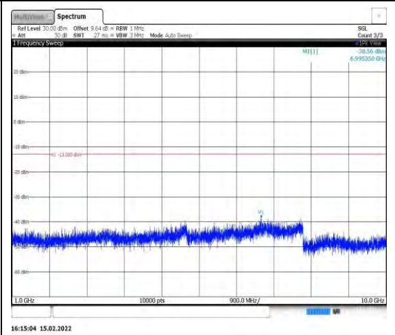
Band26-1.4MHz-QPSK-26740-1RB#0- Range2:1000~10000MHz
