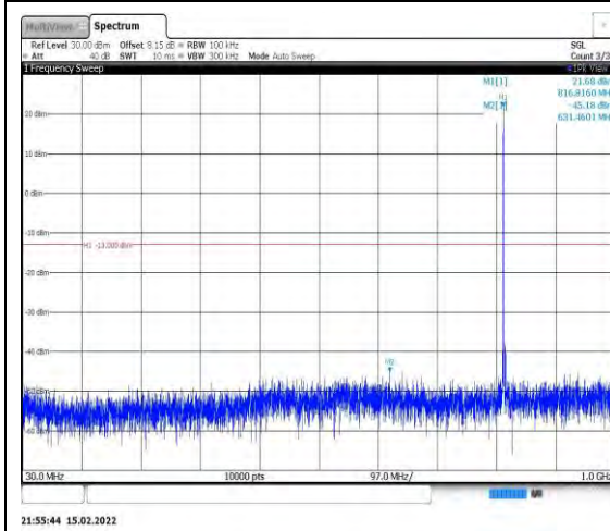
Band26-5MHz-16QAM-26740-1RB#0- Range1:30~1000MHz
