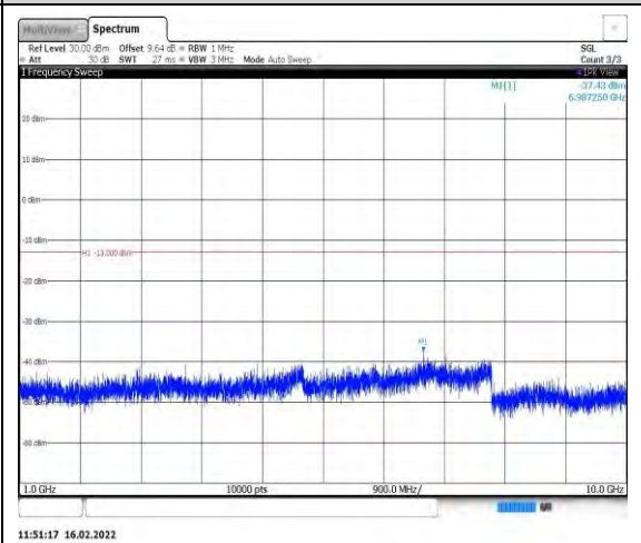
Band26-15MHz-16QAM-26915-1RB#0- Range2:1000~10000MHz
