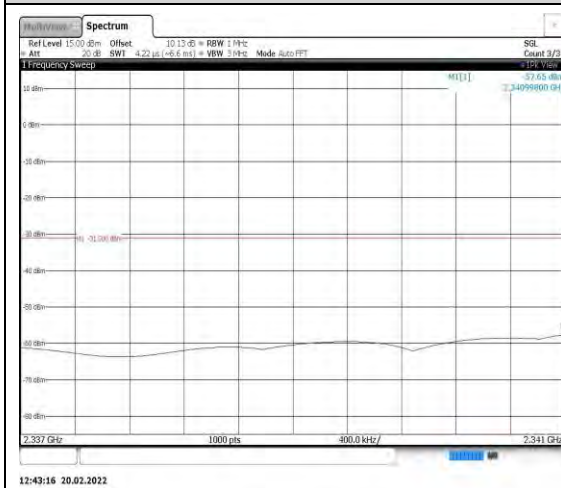
Band40-5MHz-QPSK-38750-1RB#0- Range10:2337~2341MHz
