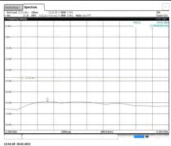
Band40-5MHz-QPSK-38750-1RB#0- Range3:2288~2292MHz
