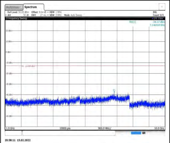
Band26-3MHz-16QAM-26740-1RB#0- Range2:1000~10000MHz
