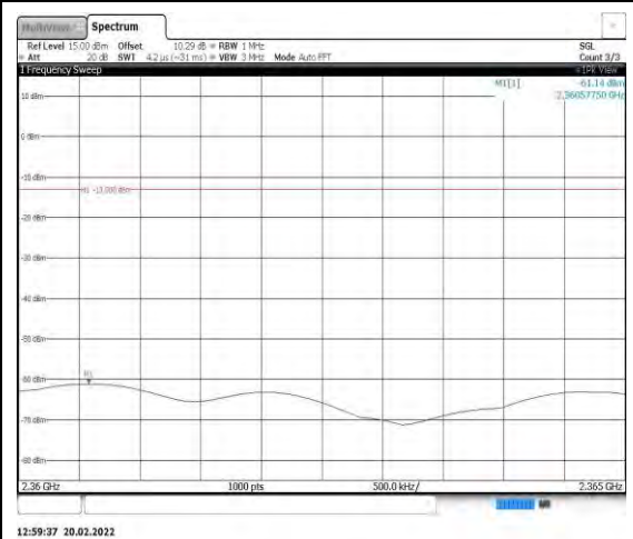
Band40-5MHz-QPSK-39200-1RB#0- Range12:2360~2365MHz
