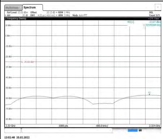
Band40-5MHz-QPSK-39225-1RB#0- Range7:2320~2324MHz
