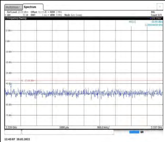
Band40-5MHz-QPSK-38750-1RB#0- Range9:2328~2337MHz
