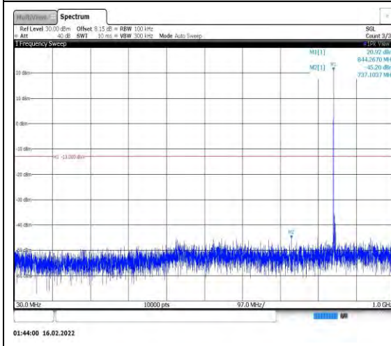
Band26-5MHz-16QAM-27015-1RB#0- Range1:30~1000MHz
