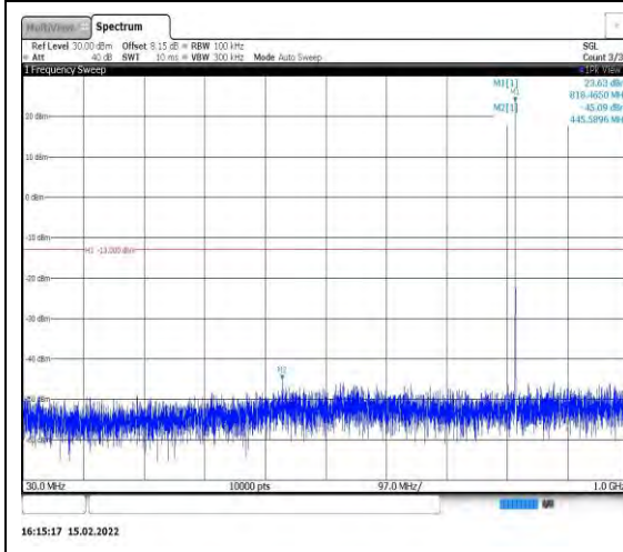
Band26-1.4MHz-16QAM-26740-1RB#0- Range1:30~1000MHz
