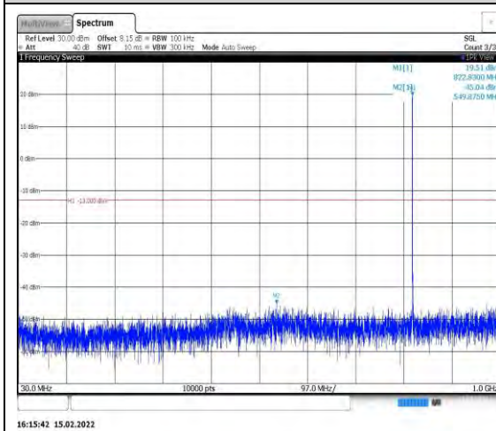
Band26-1.4MHz-QPSK-26783-1RB#0- Range1:30~1000MHz
