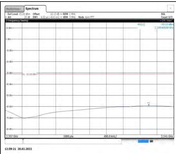
Band40-5MHz-QPSK-39200-1RB#0- Range10:2337~2341MHz
