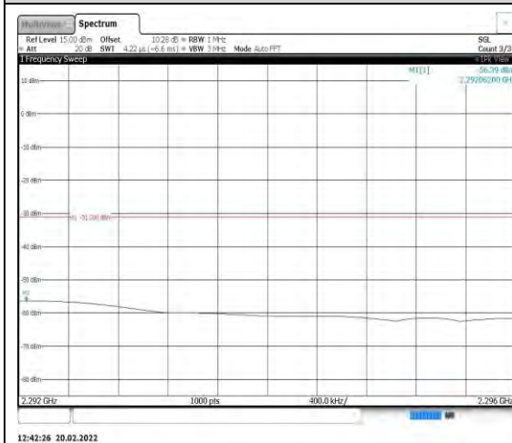
Band40-5MHz-QPSK-38750-1RB#0- Range4:2292~2296MHz
