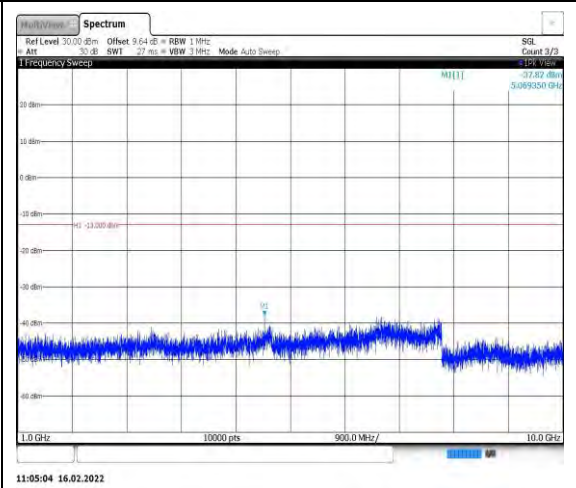
Band26-10MHz-16QAM-26990-1RB#0- Range2:1000~10000MHz
