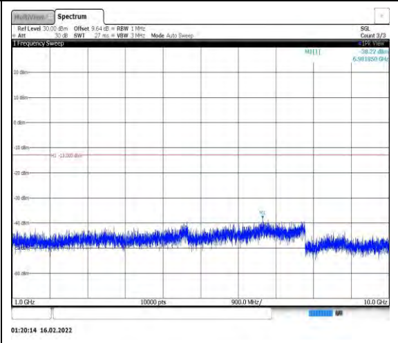
Band26-3MHz-QPSK-26915-1RB#0- Range2:1000~10000MHz
