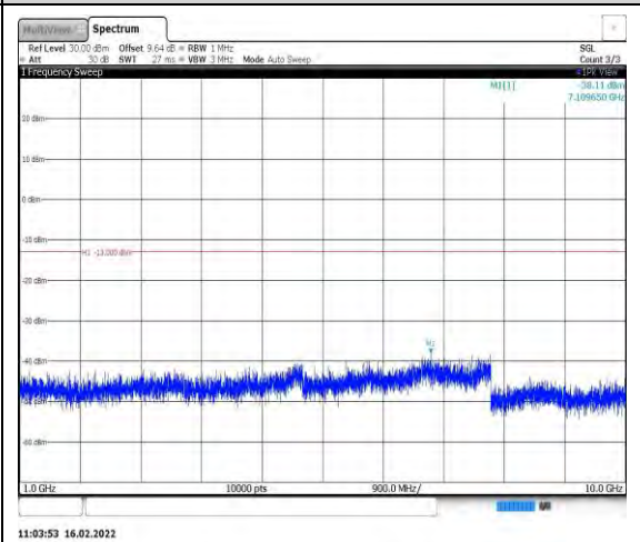
Band26-10MHz-QPSK-26915-1RB#0- Range2:1000~10000MHz
