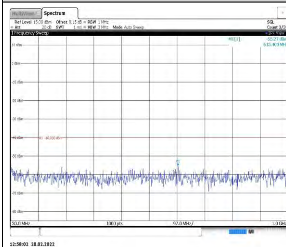
Band40-5MHz-QPSK-39200-1RB#0- Range1:30~1000MHz
