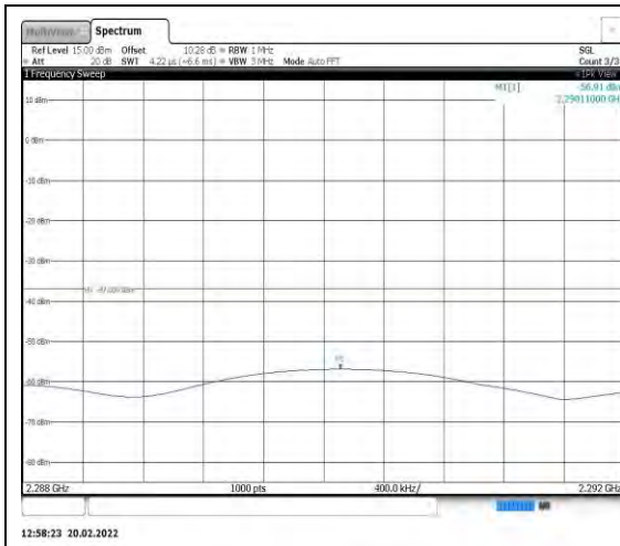
Band40-5MHz-QPSK-39200-1RB#0- Range3:2288~2292MHz
