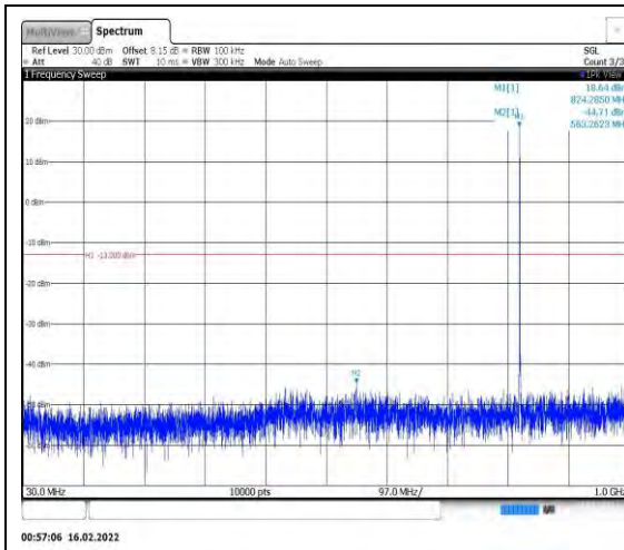
Band26-1.4MHz-16QAM-26797-1RB#0- Range1:30~1000MHz
