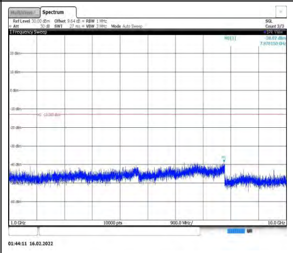
Band26-5MHz-16QAM-27015-1RB#0- Range2:1000~10000MHz
