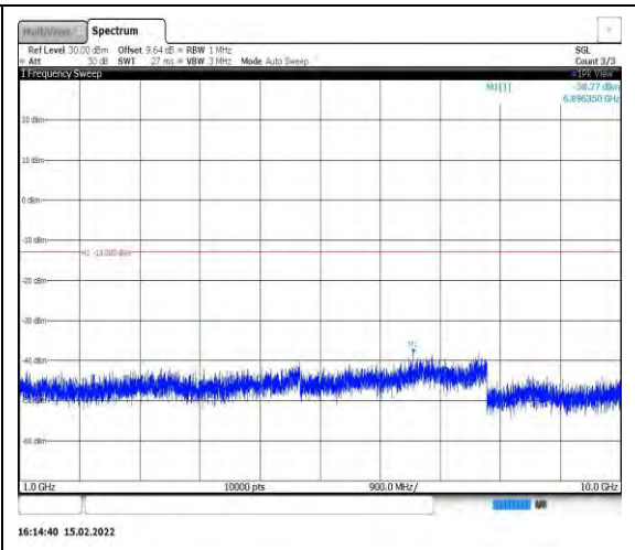
Band26-1.4MHz-16QAM-26697-1RB#0- Range2:1000~10000MHz
