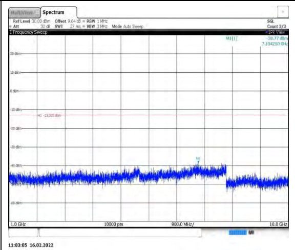
Band26-10MHz-QPSK-26840-1RB#0- Range2:1000~10000MHz
