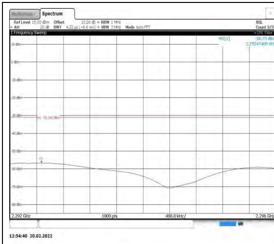
Band40-5MHz-QPSK-39175-1RB#0- Range4:2292~2296MHz
