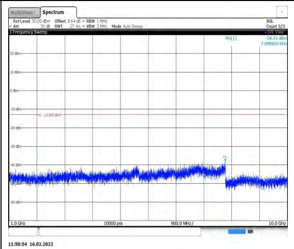
Band26-15MHz-QPSK-26915-1RB#0- Range2:1000~10000MHz
