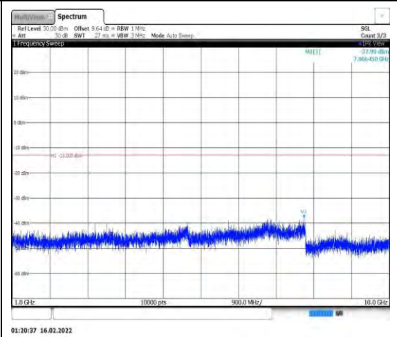
Band26-3MHz-16QAM-26915-1RB#0- Range2:1000~10000MHz
