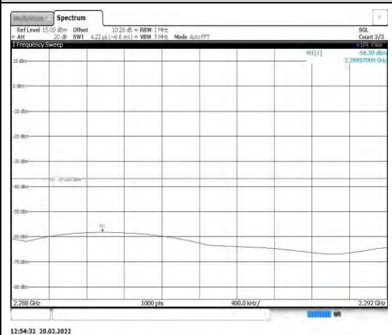
Band40-5MHz-QPSK-39175-1RB#0- Range3:2288~2292MHz
