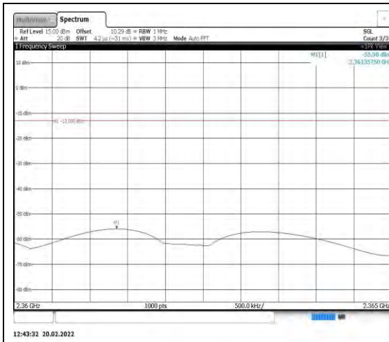
Band40-5MHz-QPSK-38750-1RB#0- Range12:2360~2365MHz
