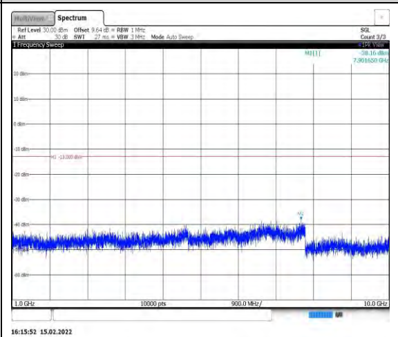
Band26-1.4MHz-QPSK-26783-1RB#0- Range2:1000~10000MHz
