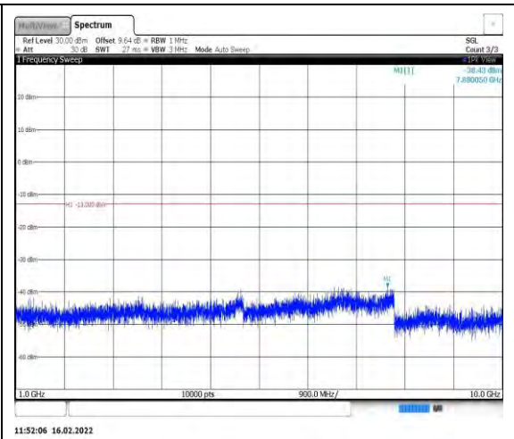
Band26-15MHz-16QAM-26965-1RB#0- Range2:1000~10000MHz
