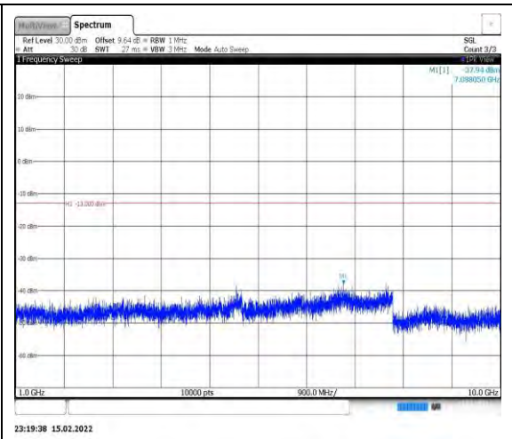
Band26-15MHz-16QAM-26765-1RB#0- Range2:1000~10000MHz
