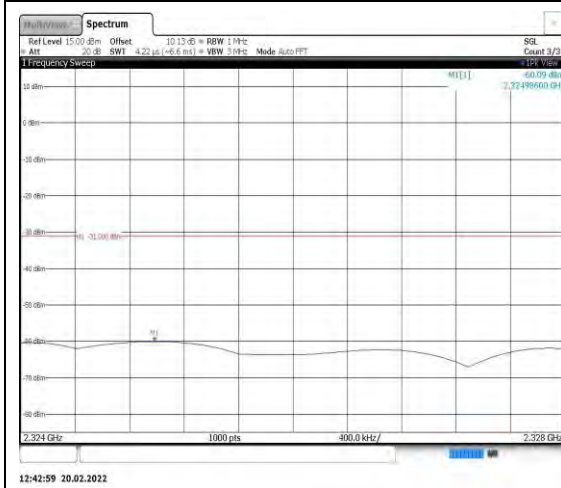
Band40-5MHz-QPSK-38750-1RB#0- Range8:2324~2328MHz
