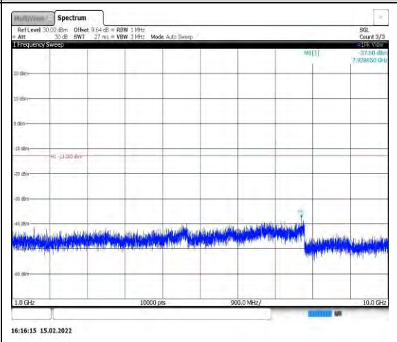
Band26-1.4MHz-16QAM-26783-1RB#0- Range2:1000~10000MHz
