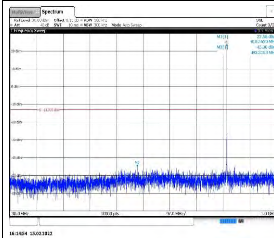
Band26-1.4MHz-QPSK-26740-1RB#0- Range1:30~1000MHz
