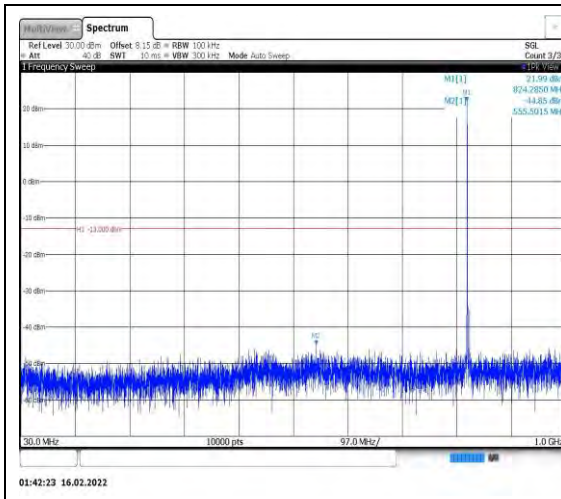
Band26-5MHz-16QAM-26815-1RB#0- Range1:30~1000MHz
