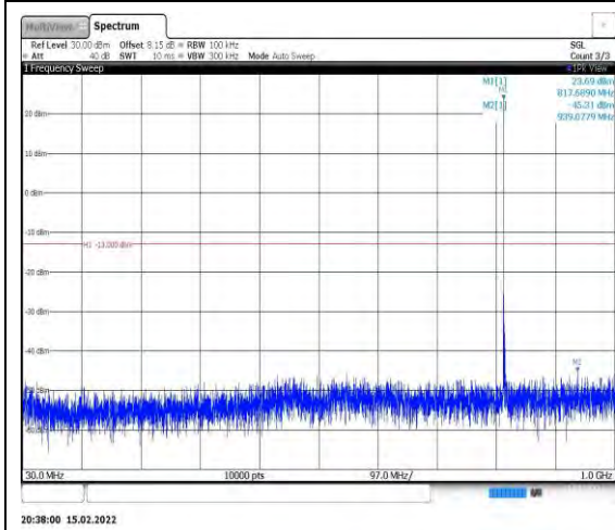
Band26-3MHz-16QAM-26740-1RB#0- Range1:30~1000MHz
