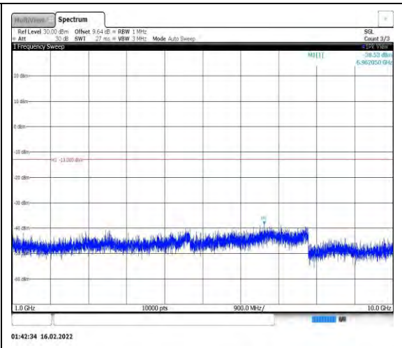
Band26-5MHz-16QAM-26815-1RB#0- Range2:1000~10000MHz
