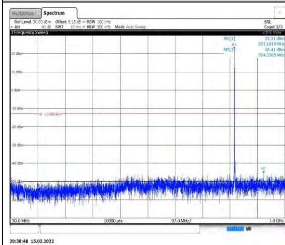
Band26-3MHz-16QAM-26775-1RB#0- Range1:30~1000MHz
