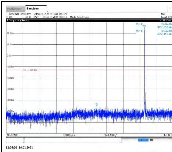
Band26-10MHz-16QAM-26915-1RB#0- Range1:30~1000MHz
