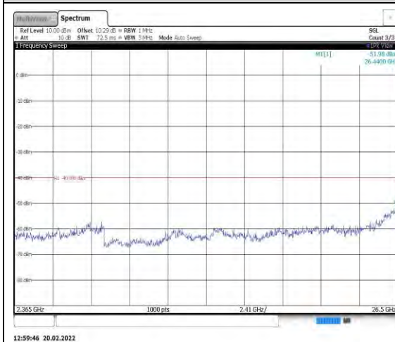
Band40-5MHz-QPSK-39200-1RB#0- Range13:2365~26500MHz
