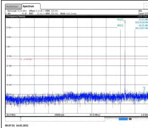
Band26-1.4MHz-QPSK-26915-1RB#0- Range1:30~1000MHz
