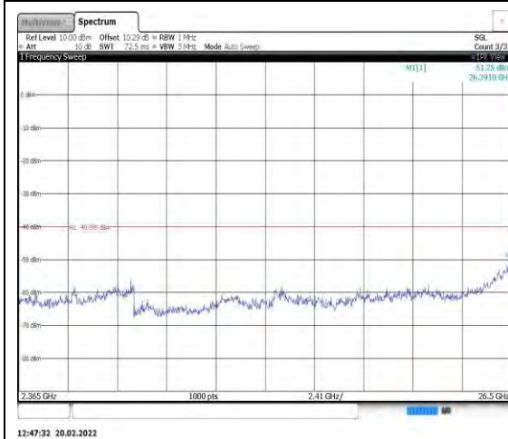
Band40-5MHz-QPSK-38775-1RB#0- Range13:2365~26500MHz
