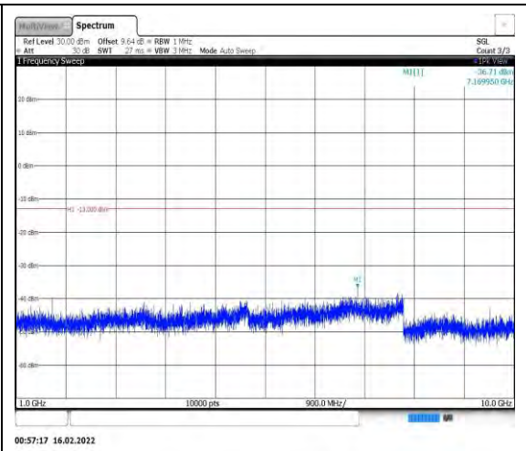
Band26-1.4MHz-16QAM-26797-1RB#0- Range2:1000~10000MHz
