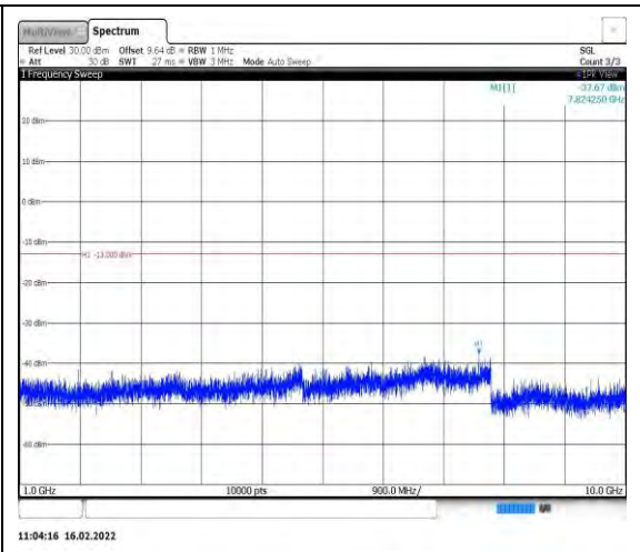
Band26-10MHz-16QAM-26915-1RB#0- Range2:1000~10000MHz
