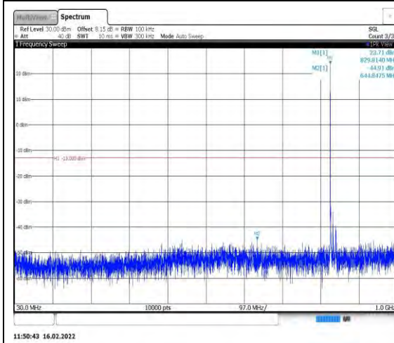
Band26-15MHz-QPSK-26915-1RB#0- Range1:30~1000MHz
