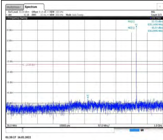
Band26-3MHz-16QAM-26915-1RB#0- Range1:30~1000MHz
