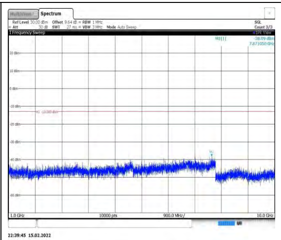
Band26-10MHz-QPSK-26740-1RB#0- Range2:1000~10000MHz
