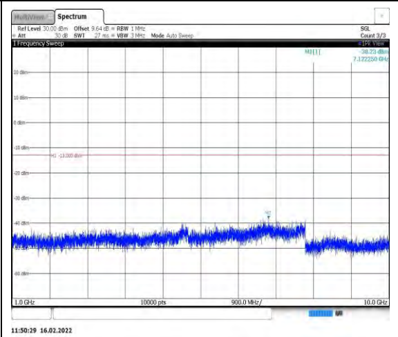
Band26-15MHz-16QAM-26865-1RB#0- Range2:1000~10000MHz
