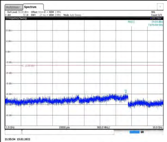
Band26-5MHz-16QAM-26740-1RB#0- Range2:1000~10000MHz
