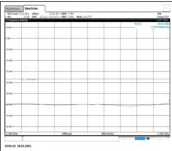
Band40-5MHz-QPSK-39225-1RB#0- Range3:2288~2292MHz
