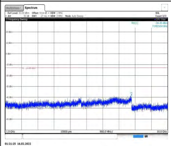
Band26-3MHz-16QAM-27025-1RB#0- Range2:1000~10000MHz
