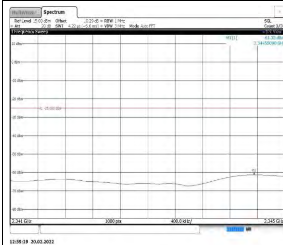
Band40-5MHz-QPSK-39200-1RB#0- Range11:2341~2345MHz
