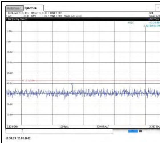
Band40-5MHz-QPSK-39200-1RB#0- Range9:2328~2337MHz
