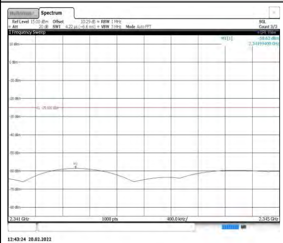
Band40-5MHz-QPSK-38750-1RB#0- Range11:2341~2345MHz
