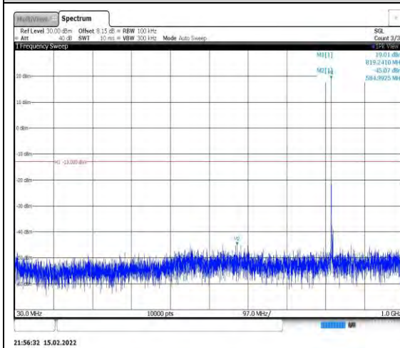
Band26-5MHz-16QAM-26765-1RB#0- Range1:30~1000MHz
