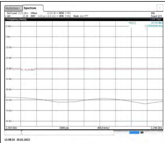
Band40-5MHz-QPSK-39200-1RB#0- Range4:2292~2296MHz
