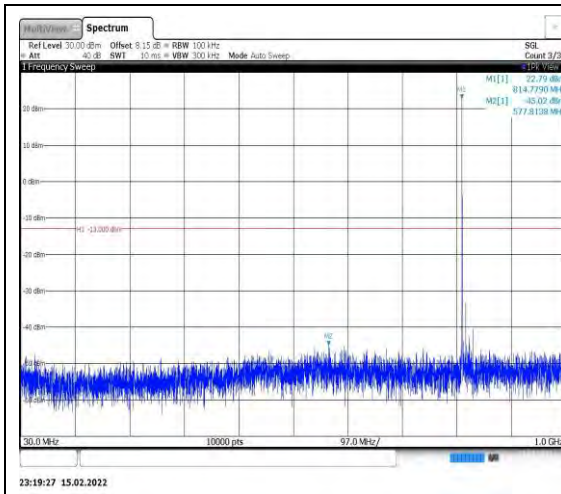
Band26-15MHz-16QAM-26765-1RB#0- Range1:30~1000MHz
