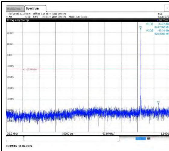
Band26-3MHz-QPSK-26805-1RB#0- Range1:30~1000MHz
