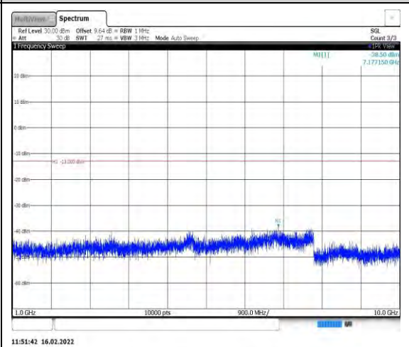
Band26-15MHz-QPSK-26965-1RB#0- Range2:1000~10000MHz
