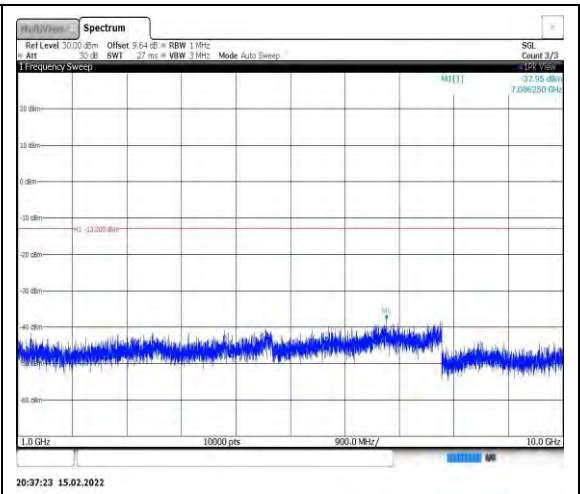
Band26-3MHz-16QAM-26705-1RB#0- Range2:1000~10000MHz
