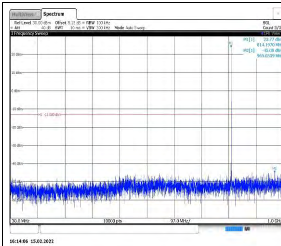
Band26-1.4MHz-QPSK-26697-1RB#0- Range1:30~1000MHz
