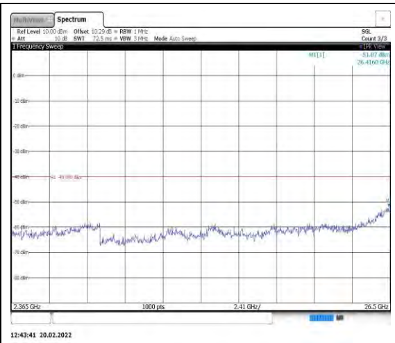
Band40-5MHz-QPSK-38750-1RB#0- Range13:2365~26500MHz
