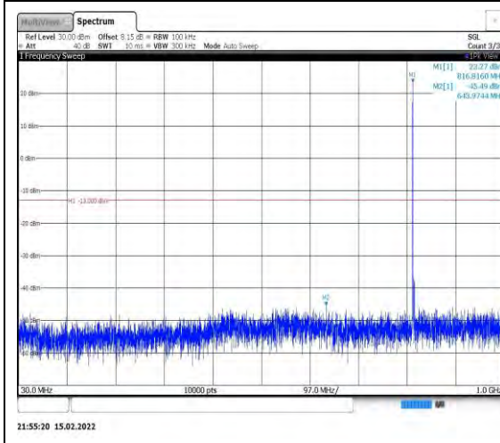
Band26-5MHz-QPSK-26740-1RB#0- Range1:30~1000MHz
