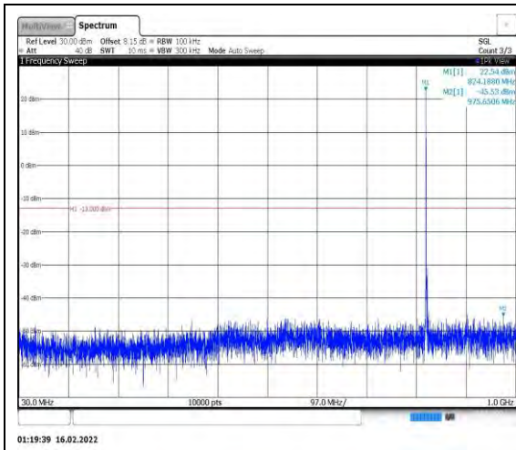
Band26-3MHz-16QAM-26805-1RB#0- Range1:30~1000MHz
