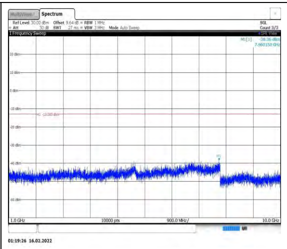
Band26-3MHz-QPSK-26805-1RB#0- Range2:1000~10000MHz
