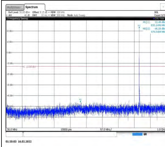
Band26-3MHz-QPSK-26915-1RB#0- Range1:30~1000MHz
