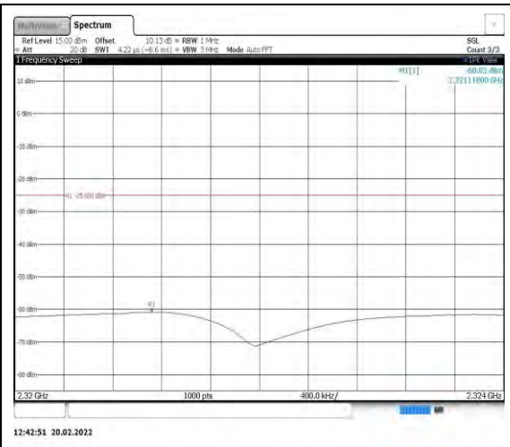
Band40-5MHz-QPSK-38750-1RB#0- Range7:2320~2324MHz
