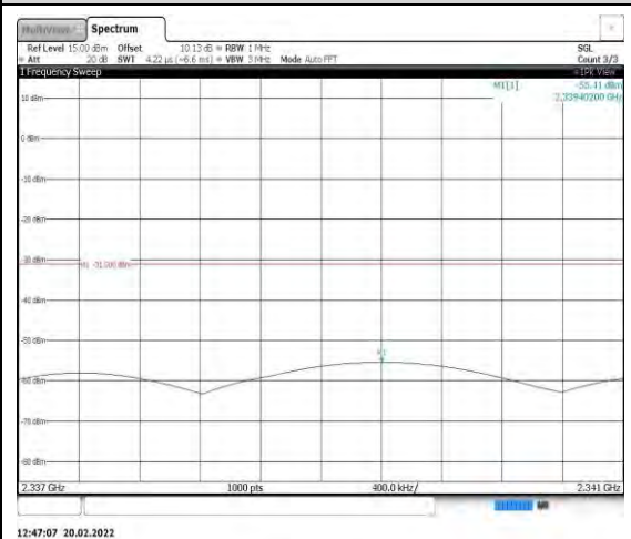
Band40-5MHz-QPSK-38775-1RB#0- Range10:2337~2341MHz
