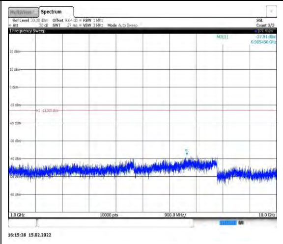
Band26-1.4MHz-16QAM-26740-1RB#0- Range2:1000~10000MHz
