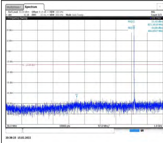
Band26-3MHz-QPSK-26775-1RB#0- Range1:30~1000MHz
