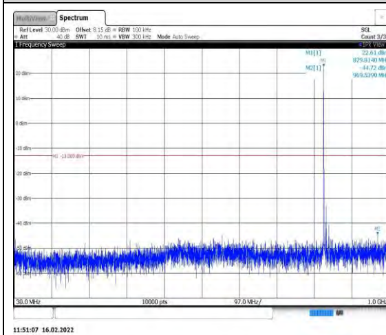
Band26-15MHz-16QAM-26915-1RB#0- Range1:30~1000MHz
