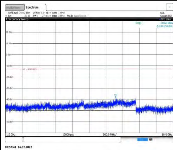
Band26-1.4MHz-QPSK-26915-1RB#0- Range2:1000~10000MHz
