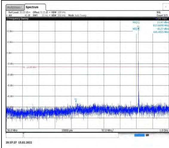
Band26-3MHz-QPSK-26740-1RB#0- Range1:30~1000MHz
