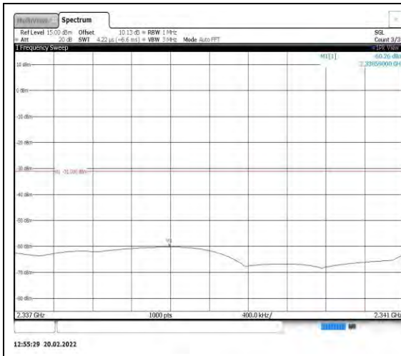
Band40-5MHz-QPSK-39175-1RB#0- Range10:2337~2341MHz
