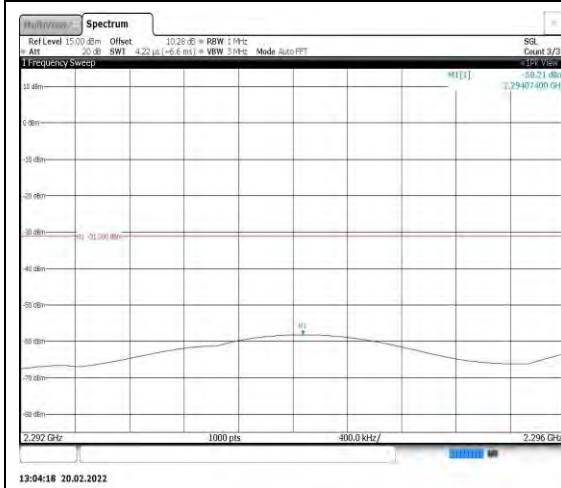
Band40-5MHz-16QAM-39225-1RB#0- Range4:2292~2296MHz
