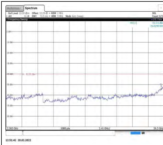
Band40-10MHz-QPSK-38750-1RB#0- Range13:2365~26500MHz
