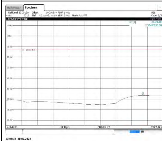
Band40-5MHz-16QAM-39225-1RB#0- Range12:2360~2365MHz
