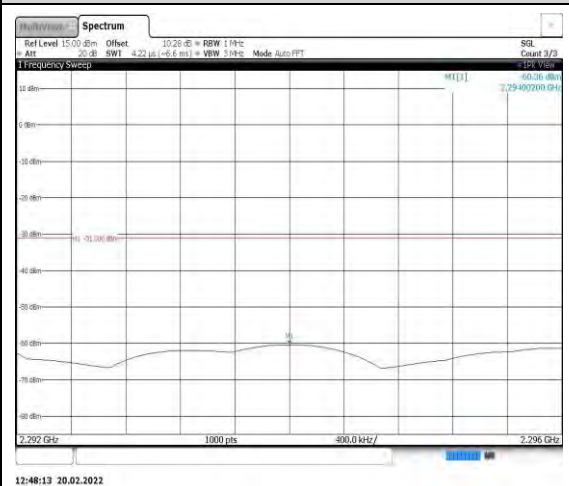
Band40-5MHz-16QAM-38775-1RB#0- Range4:2292~2296MHz
