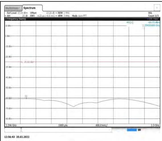
Band40-5MHz-16QAM-39175-1RB#0- Range5:2296~2300MHz
