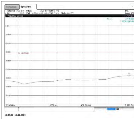
Band40-10MHz-16QAM-39200-1RB#0- Range4:2292~2296MHz
