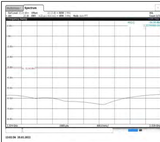
Band40-5MHz-QPSK-39225-1RB#0- Range8:2324~2328MHz
