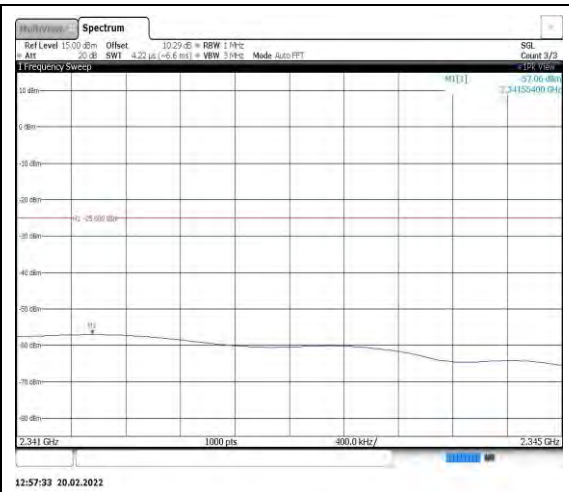
Band40-5MHz-16QAM-39175-1RB#0- Range11:2341~2345MHz
