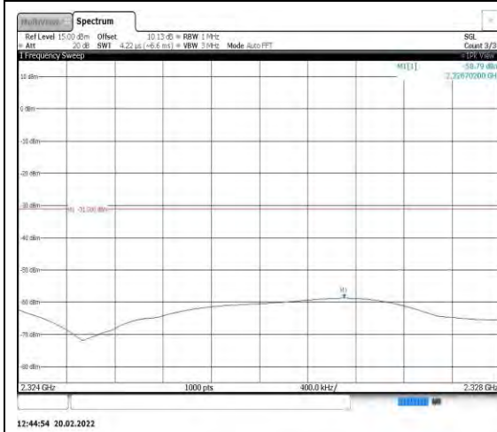
Band40-5MHz-16QAM-38750-1RB#0- Range8:2324~2328MHz
