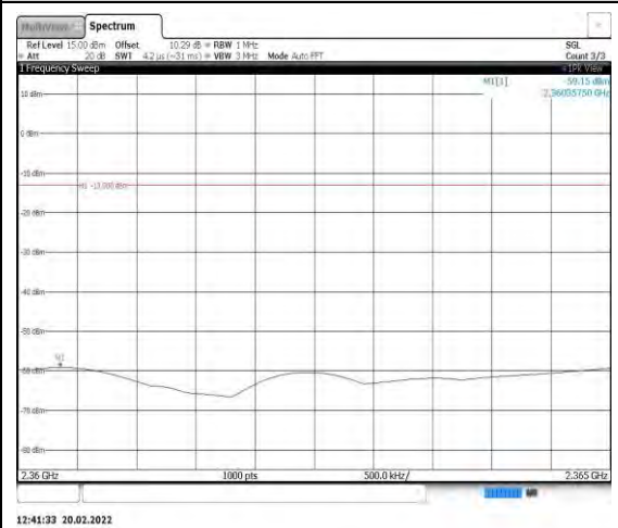
Band40-5MHz-16QAM-38725-1RB#0- Range12:2360~2365MHz
