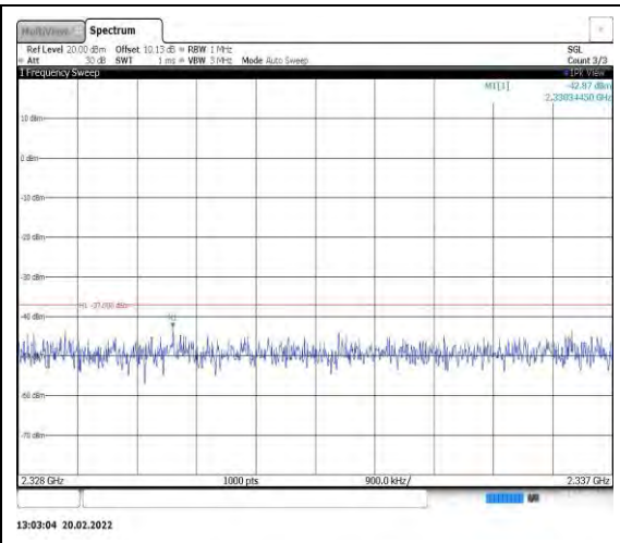
Band40-5MHz-QPSK-39225-1RB#0- Range9:2328~2337MHz
