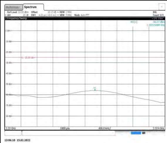
Band40-10MHz-16QAM-39200-1RB#0- Range7:2320~2324MHz
