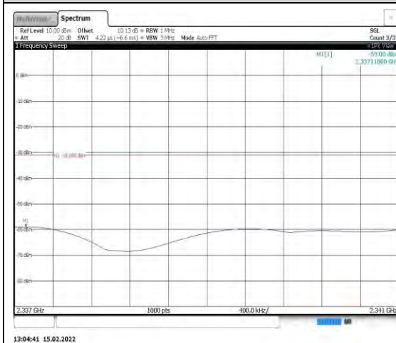
Band40-10MHz-QPSK-39200-1RB#0- Range10:2337~2341MHz
