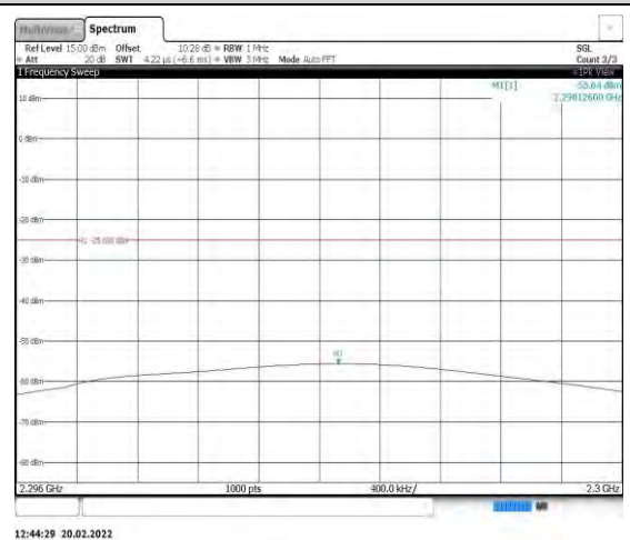
Band40-5MHz-16QAM-38750-1RB#0- Range5:2296~2300MHz
