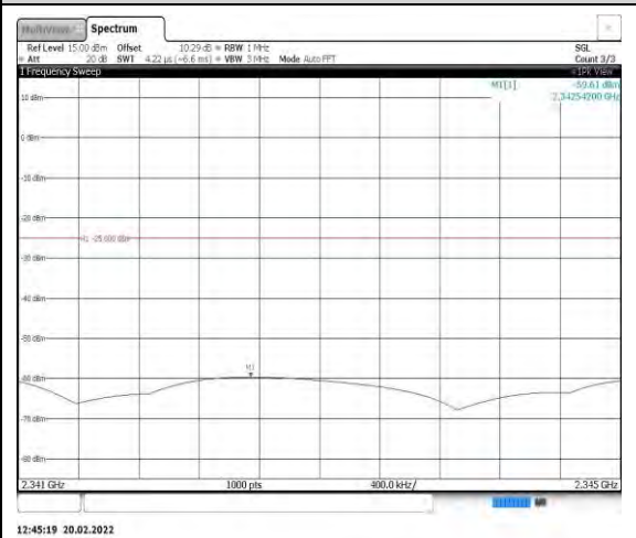
Band40-5MHz-16QAM-38750-1RB#0- Range11:2341~2345MHz
