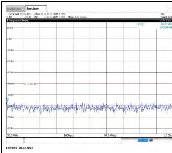
Band40-10MHz-QPSK-38750-1RB#0- Range1:30~1000MHz
