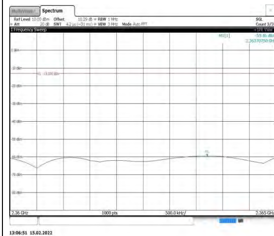
Band40-10MHz-16QAM-39200-1RB#0- Range12:2360~2365MHz
