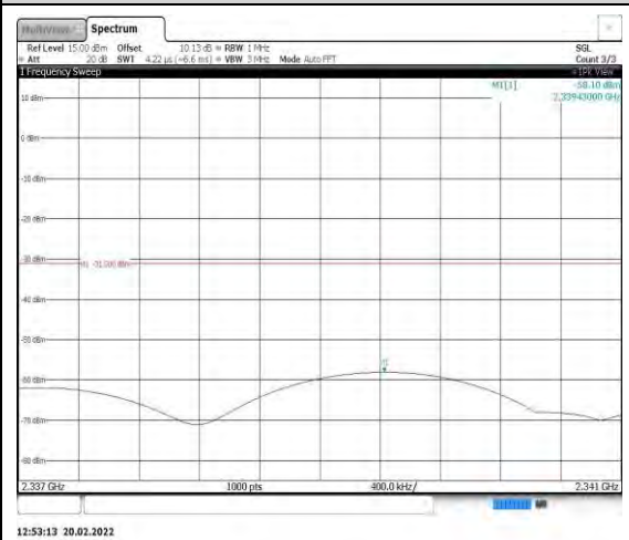
Band40-10MHz-16QAM-38750-1RB#0- Range10:2337~2341MHz
