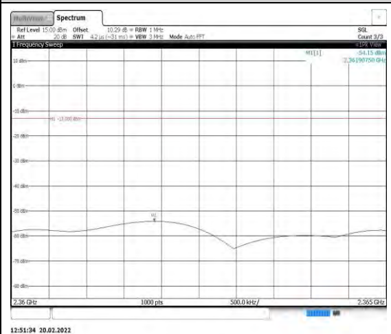
Band40-10MHz-QPSK-38750-1RB#0- Range12:2360~2365MHz
