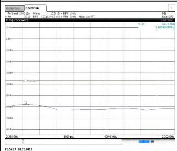
Band40-5MHz-16QAM-39175-1RB#0- Range3:2288~2292MHz
