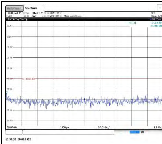
Band40-5MHz-16QAM-38725-1RB#0- Range1:30~1000MHz
