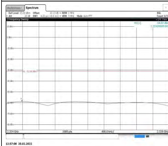
Band40-5MHz-16QAM-39175-1RB#0- Range8:2324~2328MHz
