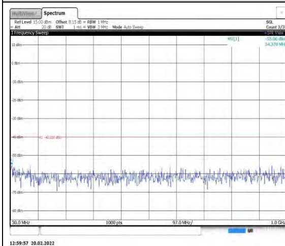
Band40-5MHz-16QAM-39200-1RB#0- Range1:30~1000MHz
