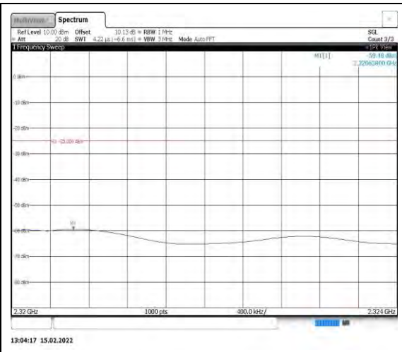
Band40-10MHz-QPSK-39200-1RB#0- Range7:2320~2324MHz
