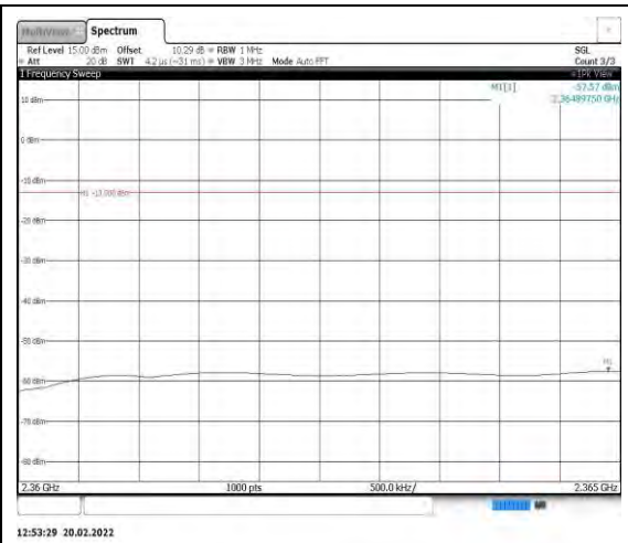
Band40-10MHz-16QAM-38750-1RB#0- Range12:2360~2365MHz
