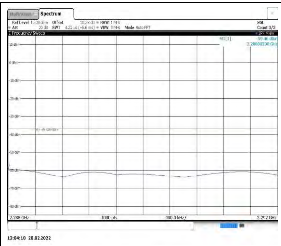
Band40-5MHz-16QAM-39225-1RB#0- Range3:2288~2292MHz
