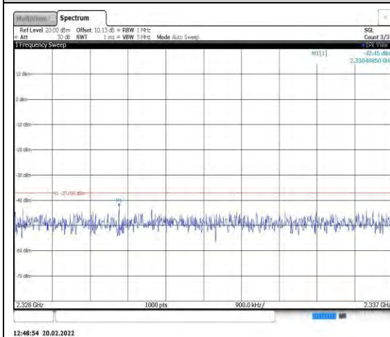
Band40-5MHz-16QAM-38775-1RB#0- Range9:2328~2337MHz
