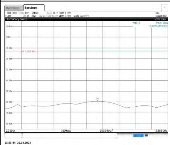
Band40-10MHz-QPSK-38750-1RB#0- Range6:2300~2305MHz
