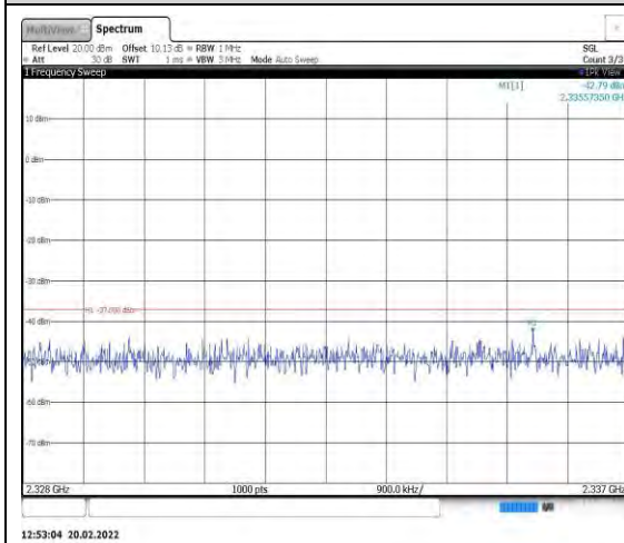
Band40-10MHz-16QAM-38750-1RB#0- Range9:2328~2337MHz
