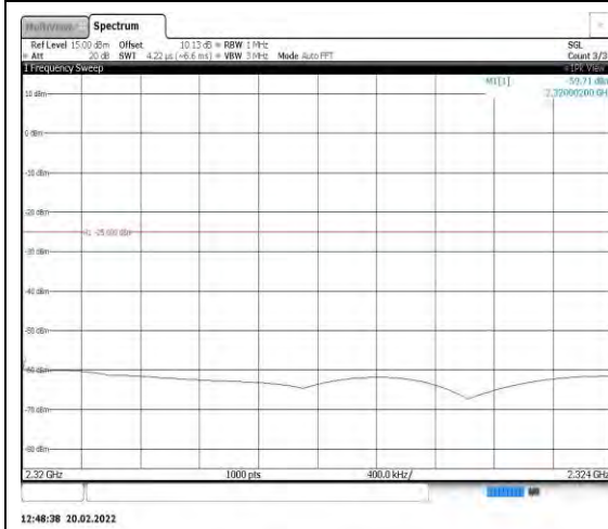
Band40-5MHz-16QAM-38775-1RB#0- Range7:2320~2324MHz
