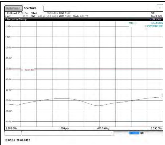
Band40-5MHz-16QAM-39200-1RB#0- Range4:2292~2296MHz
