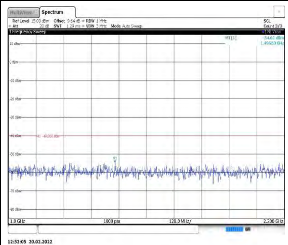
Band40-10MHz-16QAM-38750-1RB#0- Range2:1000~2288MHz
