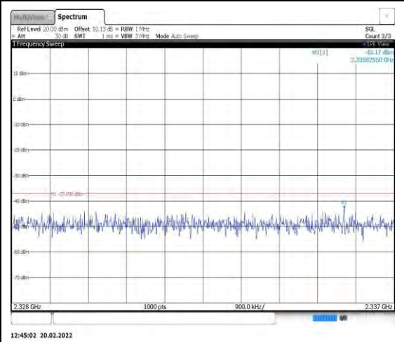
Band40-5MHz-16QAM-38750-1RB#0- Range9:2328~2337MHz
