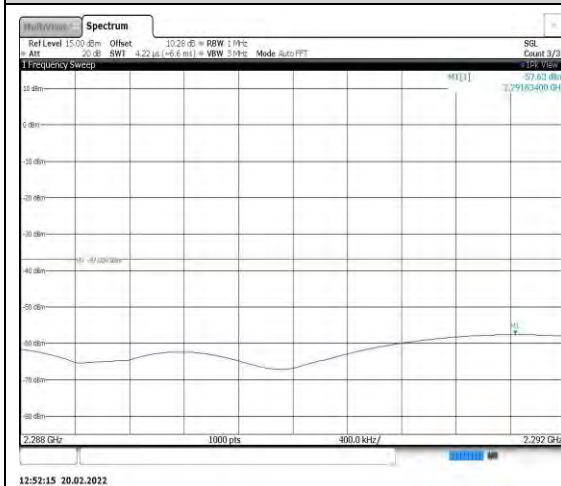
Band40-10MHz-16QAM-38750-1RB#0- Range3:2288~2292MHz
