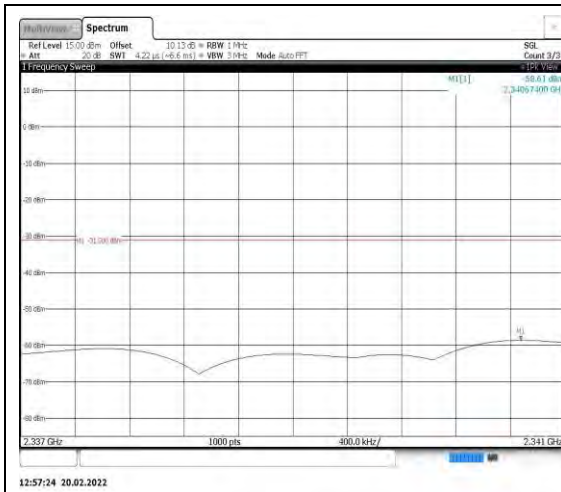
Band40-5MHz-16QAM-39175-1RB#0- Range10:2337~2341MHz
