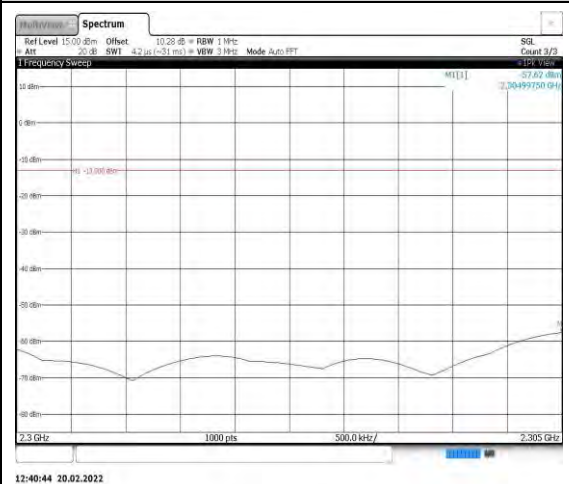
Band40-5MHz-16QAM-38725-1RB#0- Range6:2300~2305MHz
