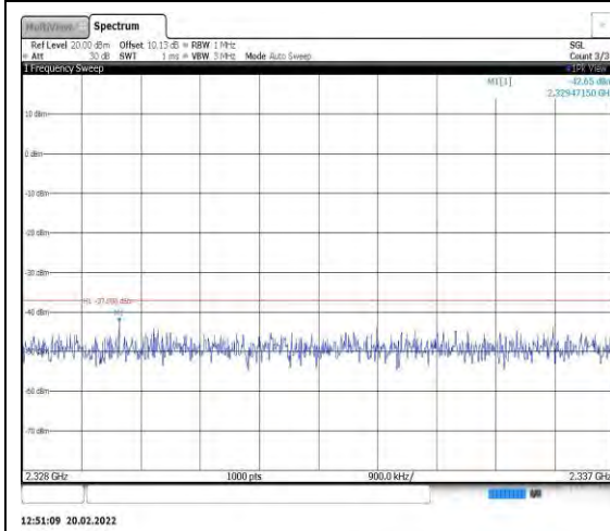
Band40-10MHz-QPSK-38750-1RB#0- Range9:2328~2337MHz
