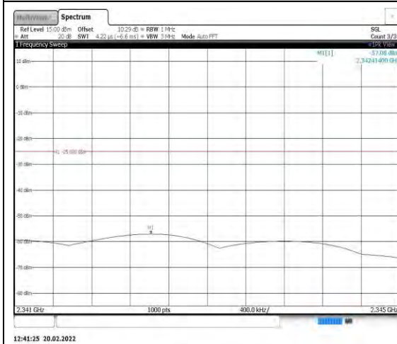
Band40-5MHz-16QAM-38725-1RB#0- Range11:2341~2345MHz
