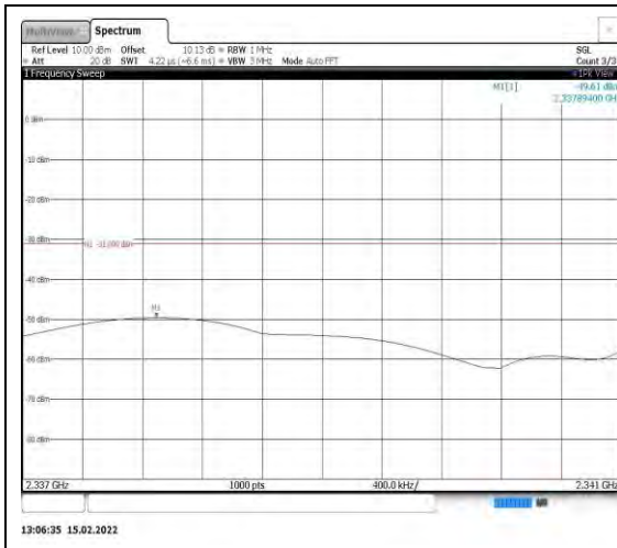
Band40-10MHz-16QAM-39200-1RB#0- Range10:2337~2341MHz
