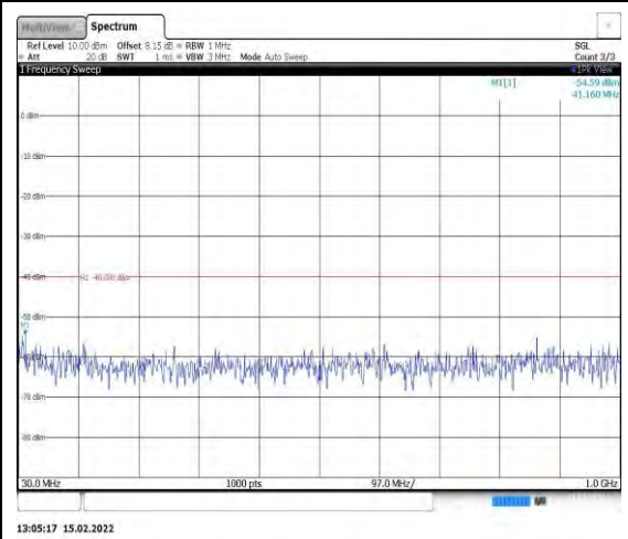
Band40-10MHz-16QAM-39200-1RB#0- Range1:30~1000MHz
