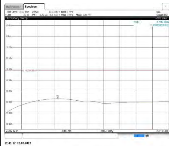
Band40-5MHz-16QAM-38725-1RB#0- Range10:2337~2341MHz
