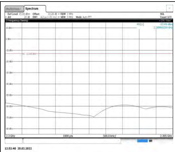
Band40-10MHz-16QAM-38750-1RB#0- Range6:2300~2305MHz
