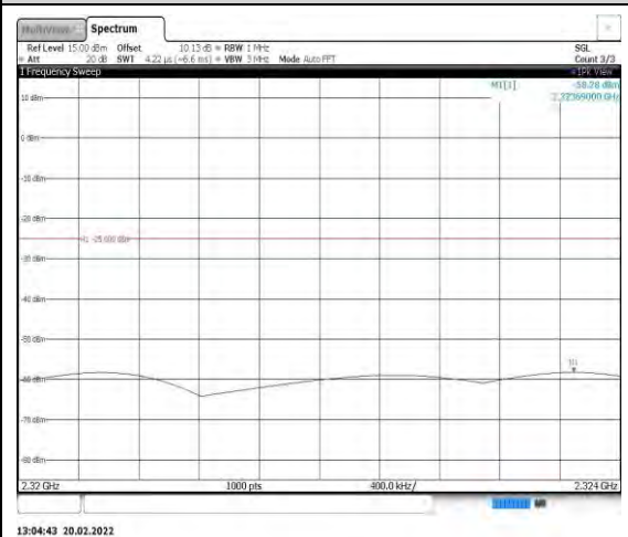
Band40-5MHz-16QAM-39225-1RB#0- Range7:2320~2324MHz
