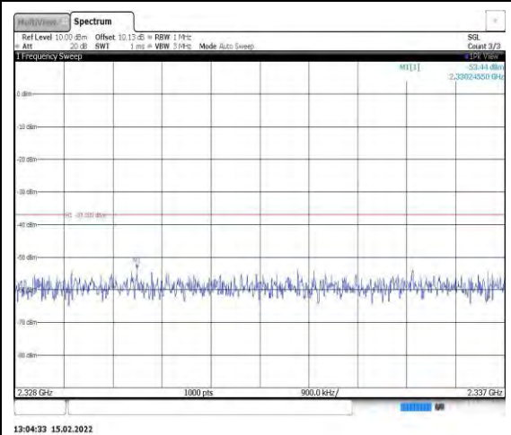
Band40-10MHz-QPSK-39200-1RB#0- Range9:2328~2337MHz
