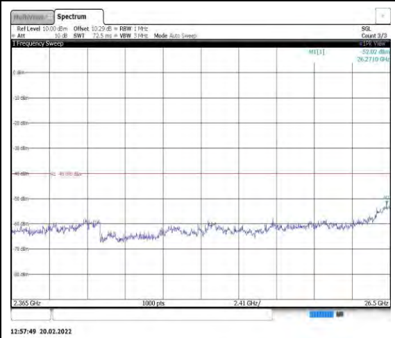
Band40-5MHz-16QAM-39175-1RB#0- Range13:2365~26500MHz
