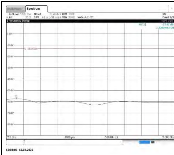
Band40-10MHz-QPSK-39200-1RB#0- Range6:2300~2305MHz
