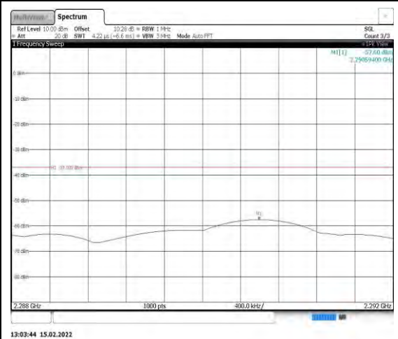
Band40-10MHz-QPSK-39200-1RB#0- Range3:2288~2292MHz
