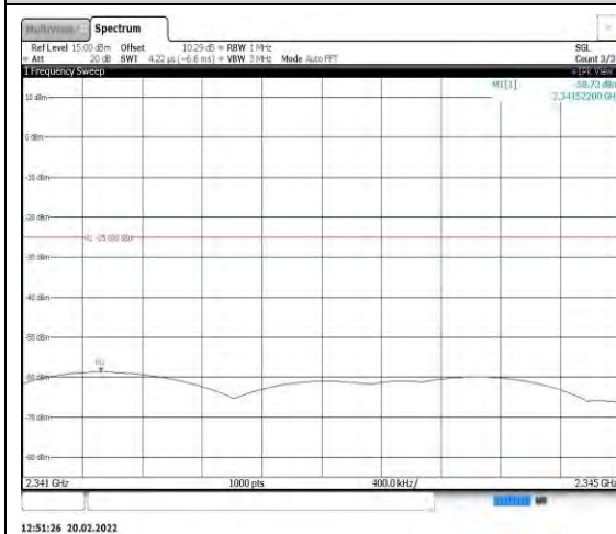
Band40-10MHz-QPSK-38750-1RB#0- Range11:2341~2345MHz
