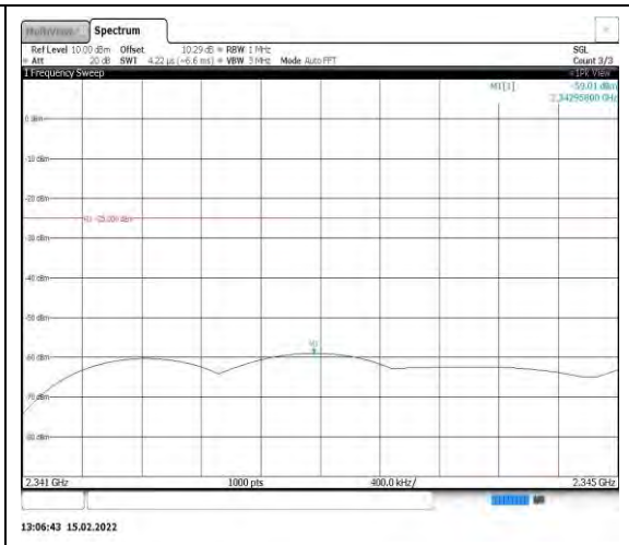
Band40-10MHz-16QAM-39200-1RB#0- Range11:2341~2345MHz
