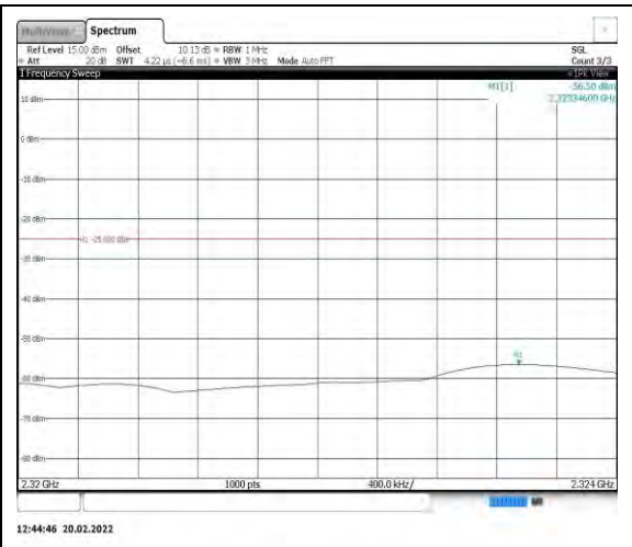
Band40-5MHz-16QAM-38750-1RB#0- Range7:2320~2324MHz
