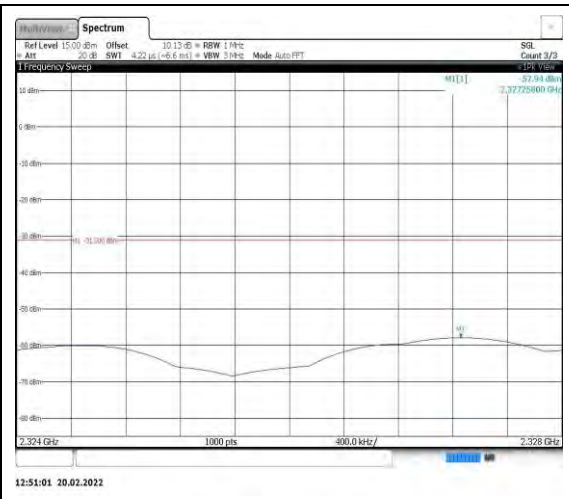
Band40-10MHz-QPSK-38750-1RB#0- Range8:2324~2328MHz
