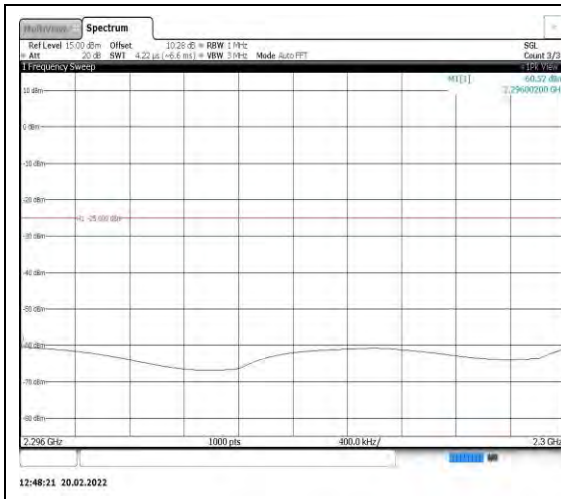
Band40-5MHz-16QAM-38775-1RB#0- Range5:2296~2300MHz
