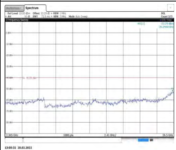
Band40-5MHz-16QAM-39225-1RB#0- Range13:2365~26500MHz
