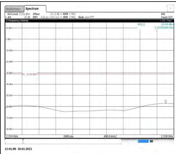
Band40-5MHz-16QAM-38725-1RB#0- Range8:2324~2328MHz
