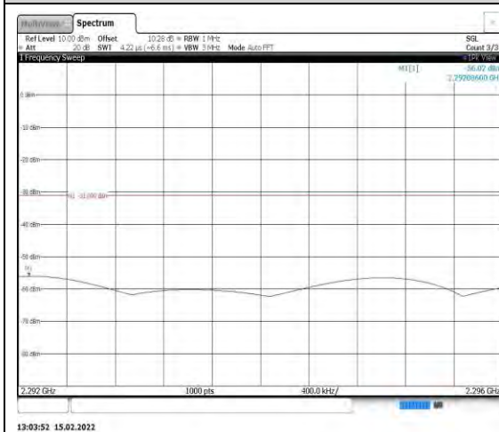
Band40-10MHz-QPSK-39200-1RB#0- Range4:2292~2296MHz
