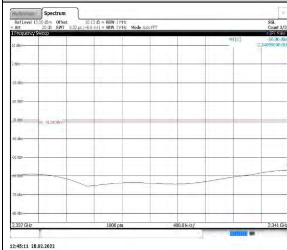
Band40-5MHz-16QAM-38750-1RB#0- Range10:2337~2341MHz
