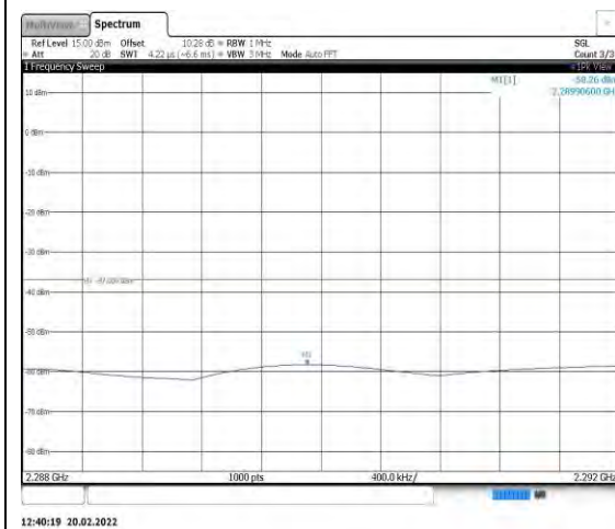
Band40-5MHz-16QAM-38725-1RB#0- Range3:2288~2292MHz
