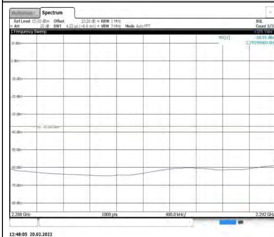
Band40-5MHz-16QAM-38775-1RB#0- Range3:2288~2292MHz
