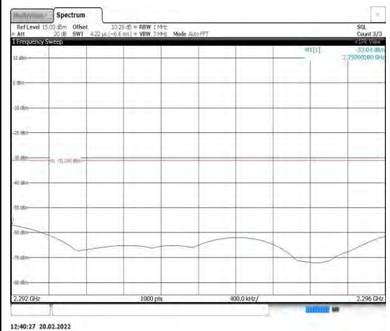
Band40-5MHz-16QAM-38725-1RB#0- Range4:2292~2296MHz
