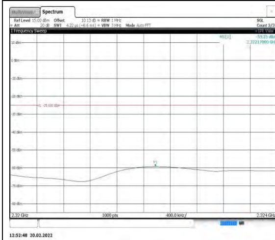
Band40-10MHz-16QAM-38750-1RB#0- Range7:2320~2324MHz
