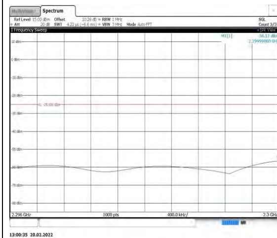
Band40-5MHz-16QAM-39200-1RB#0- Range5:2296~2300MHz
