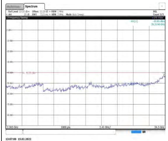
Band40-10MHz-16QAM-39200-1RB#0- Range13:2365~26500MHz
