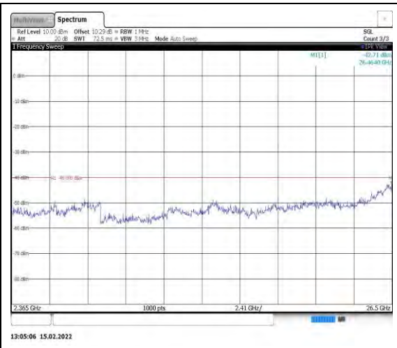
Band40-10MHz-QPSK-39200-1RB#0- Range13:2365~26500MHz
