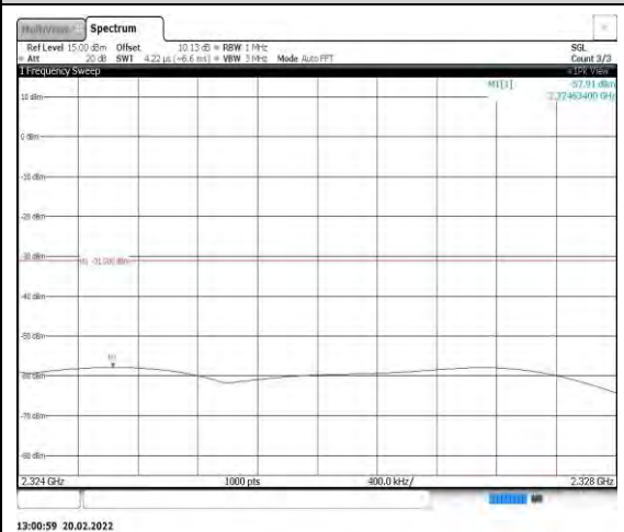
Band40-5MHz-16QAM-39200-1RB#0- Range8:2324~2328MHz
