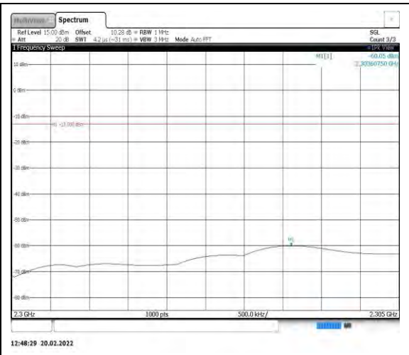
Band40-5MHz-16QAM-38775-1RB#0- Range6:2300~2305MHz
