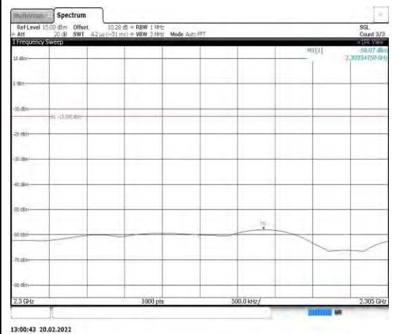
Band40-5MHz-16QAM-39200-1RB#0- Range6:2300~2305MHz
