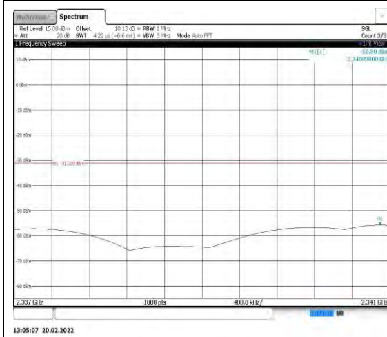
Band40-5MHz-16QAM-39225-1RB#0- Range10:2337~2341MHz
