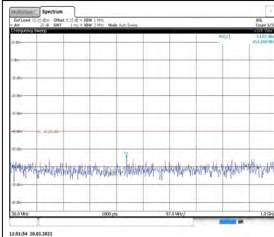
Band40-10MHz-16QAM-38750-1RB#0- Range1:30~1000MHz
