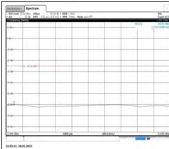
Band40-10MHz-16QAM-38750-1RB#0- Range11:2341~2345MHz
