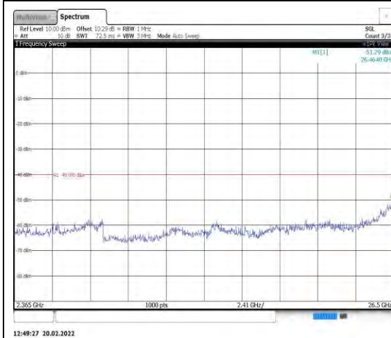
Band40-5MHz-16QAM-38775-1RB#0- Range13:2365~26500MHz
