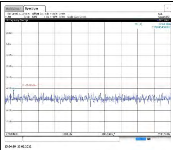
Band40-5MHz-16QAM-39225-1RB#0- Range9:2328~2337MHz
