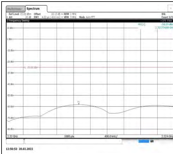
Band40-10MHz-QPSK-38750-1RB#0- Range7:2320~2324MHz
