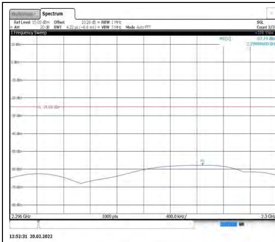
Band40-10MHz-16QAM-38750-1RB#0- Range5:2296~2300MHz
