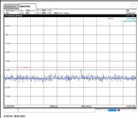
Band40-5MHz-16QAM-39175-1RB#0- Range9:2328~2337MHz
