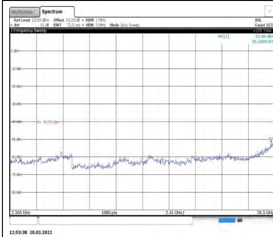
Band40-10MHz-16QAM-38750-1RB#0- Range13:2365~26500MHz
