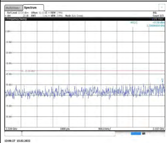
Band40-10MHz-16QAM-39200-1RB#0- Range9:2328~2337MHz
