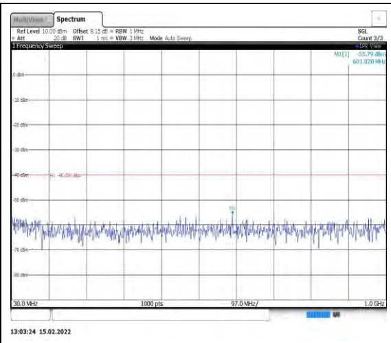
Band40-10MHz-QPSK-39200-1RB#0- Range1:30~1000MHz
