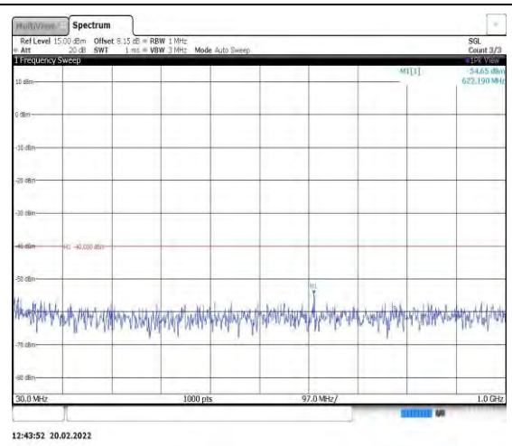
Band40-5MHz-16QAM-38750-1RB#0- Range1:30~1000MHz
