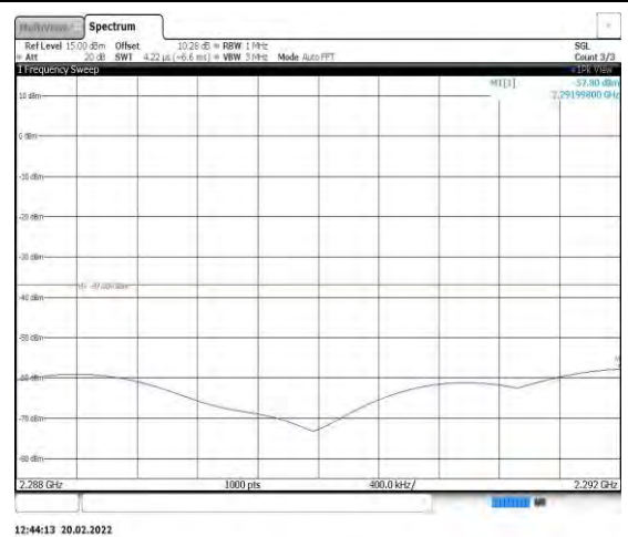
Band40-5MHz-16QAM-38750-1RB#0- Range3:2288~2292MHz
