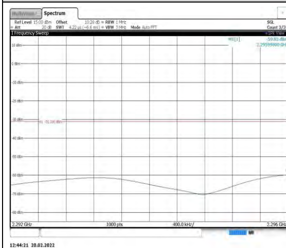
Band40-5MHz-16QAM-38750-1RB#0- Range4:2292~2296MHz
