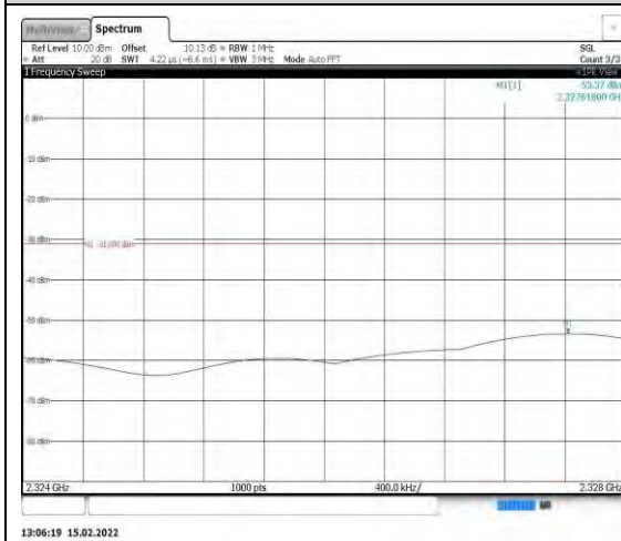
Band40-10MHz-16QAM-39200-1RB#0- Range8:2324~2328MHz
