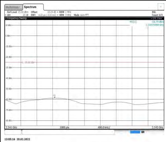
Band40-5MHz-16QAM-39225-1RB#0- Range11:2341~2345MHz
