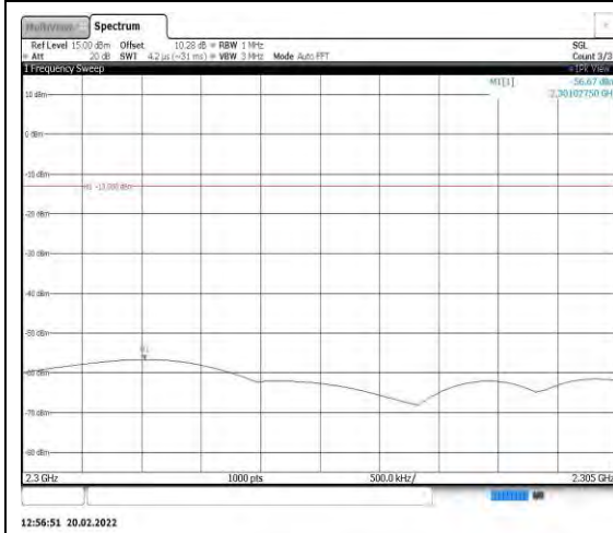
Band40-5MHz-16QAM-39175-1RB#0- Range6:2300~2305MHz
