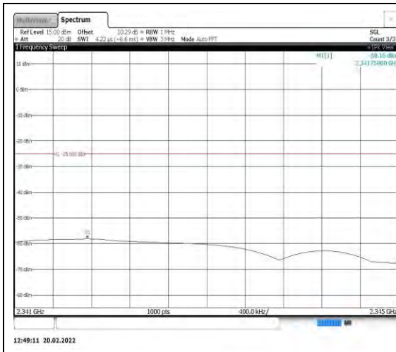
Band40-5MHz-16QAM-38775-1RB#0- Range11:2341~2345MHz
