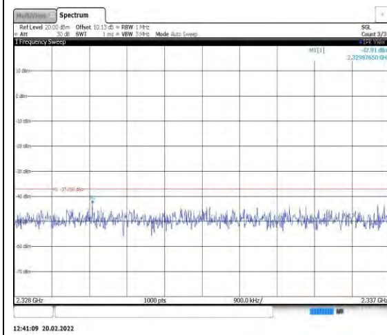
Band40-5MHz-16QAM-38725-1RB#0- Range9:2328~2337MHz
