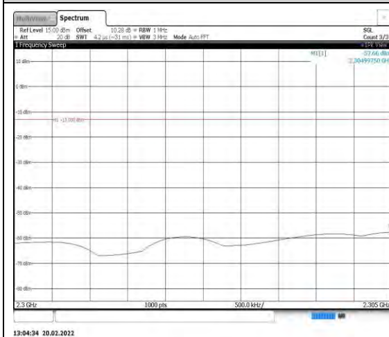
Band40-5MHz-16QAM-39225-1RB#0- Range6:2300~2305MHz
