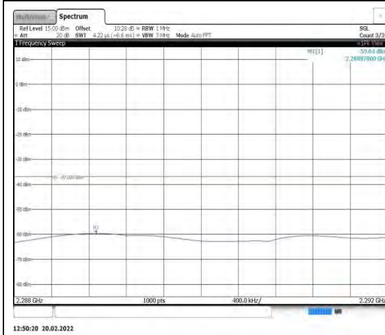
Band40-10MHz-QPSK-38750-1RB#0- Range3:2288~2292MHz
