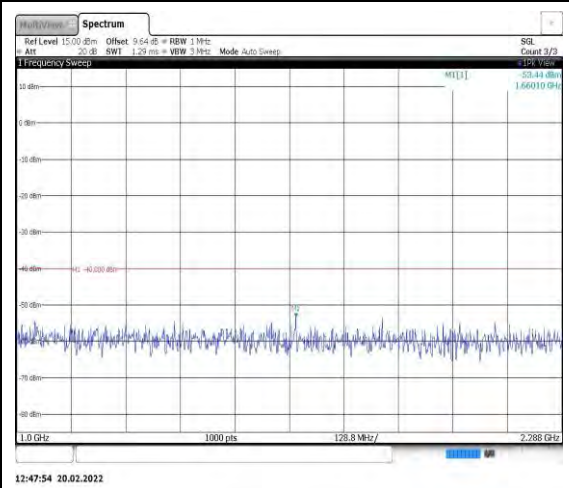
Band40-5MHz-16QAM-38775-1RB#0- Range2:1000~2288MHz
