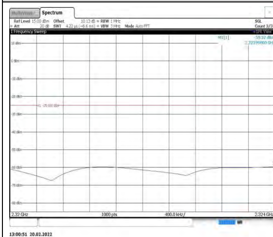
Band40-5MHz-16QAM-39200-1RB#0- Range7:2320~2324MHz
