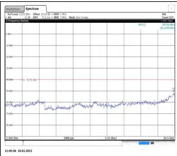
Band40-5MHz-16QAM-38750-1RB#0- Range13:2365~26500MHz
