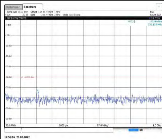
Band40-5MHz-16QAM-39175-1RB#0- Range1:30~1000MHz
