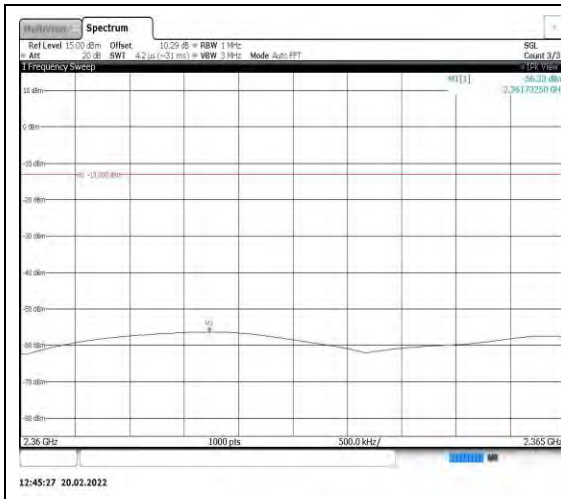
Band40-5MHz-16QAM-38750-1RB#0- Range12:2360~2365MHz
