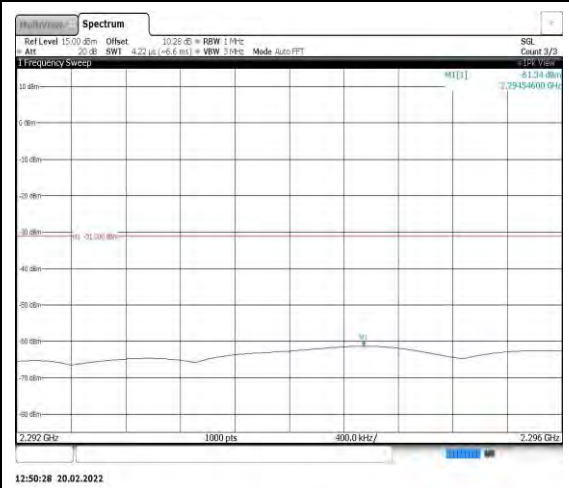
Band40-10MHz-QPSK-38750-1RB#0- Range4:2292~2296MHz
