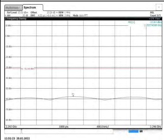
Band40-10MHz-16QAM-38750-1RB#0- Range4:2292~2296MHz
