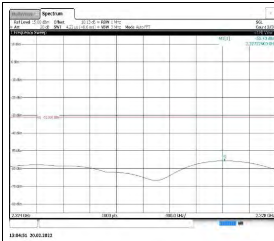
Band40-5MHz-16QAM-39225-1RB#0- Range8:2324~2328MHz
