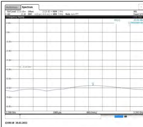
Band40-5MHz-16QAM-39200-1RB#0- Range3:2288~2292MHz
