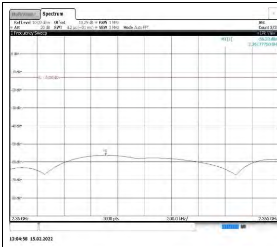
Band40-10MHz-QPSK-39200-1RB#0- Range12:2360~2365MHz
