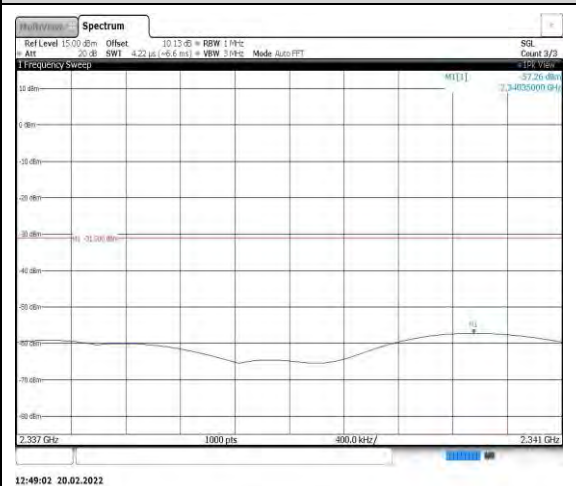
Band40-5MHz-16QAM-38775-1RB#0- Range10:2337~2341MHz
