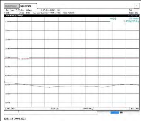
Band40-10MHz-QPSK-38750-1RB#0- Range10:2337~2341MHz
