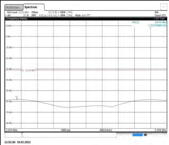
Band40-10MHz-16QAM-38750-1RB#0- Range8:2324~2328MHz
