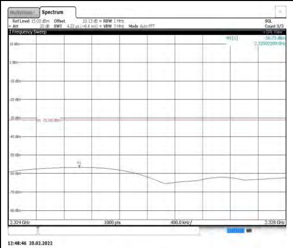
Band40-5MHz-16QAM-38775-1RB#0- Range8:2324~2328MHz
