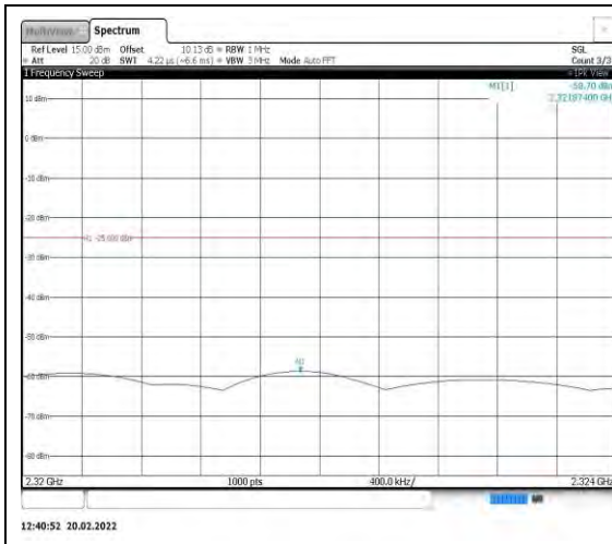
Band40-5MHz-16QAM-38725-1RB#0- Range7:2320~2324MHz
