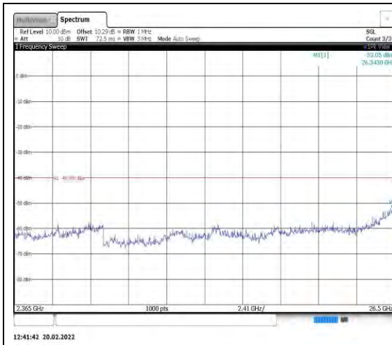
Band40-5MHz-16QAM-38725-1RB#0- Range13:2365~26500MHz
