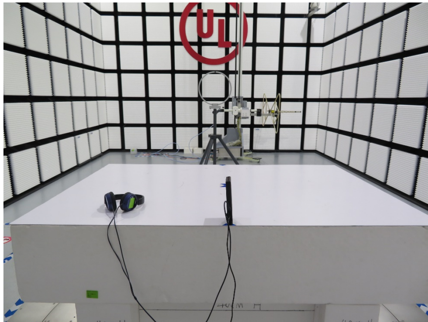
MEASUREMENT POSITION OF BT/WIFI/NFC
