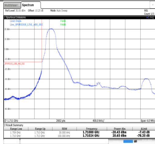
Band4-3MHz-16QAM-19965-1RB#0-PASS
