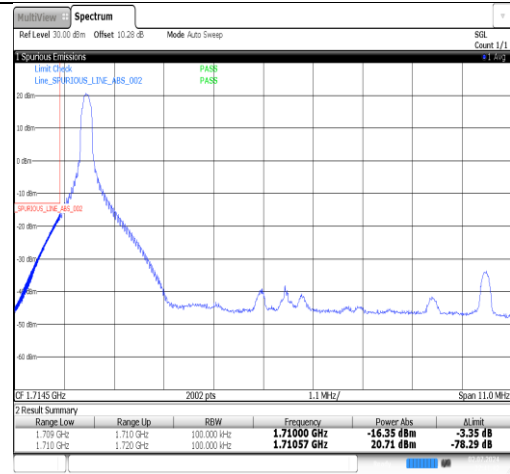
Band4-10MHz-16QAM-20000-1RB#49-PASS
