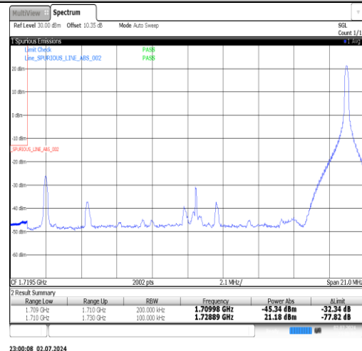
Band4-20MHz-QPSK-20300-100RB#0-PASS
