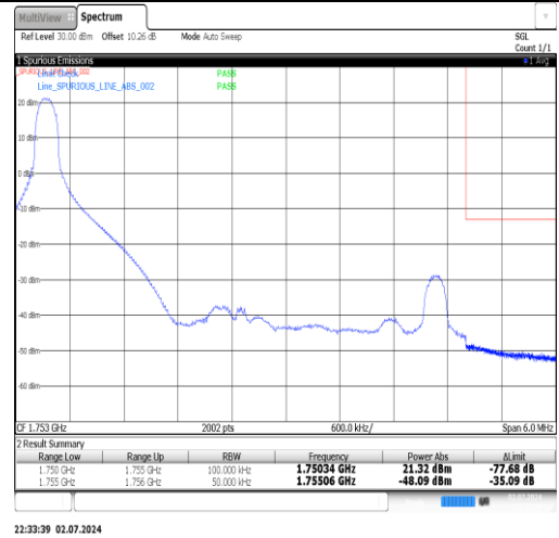
Band4-5MHz-QPSK-20375-1RB#24-PRELIMINARY
