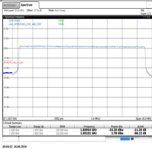
Band2-15MHz-QPSK-19125-1RB#0-PASS
