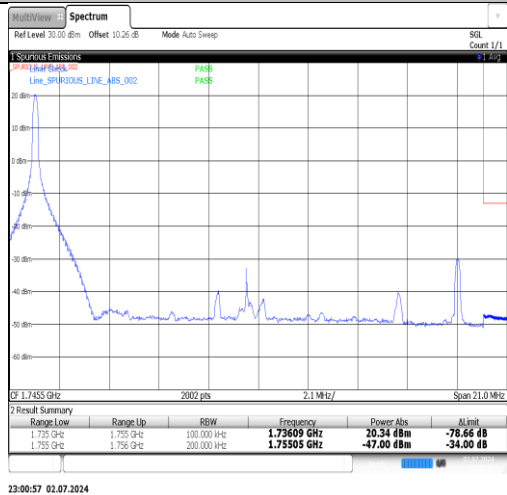
Band4-20MHz-16QAM-20300-1RB#99-PASS
