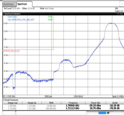
Band4-1.4MHz-16QAM-20393-6RB#0-PASS
