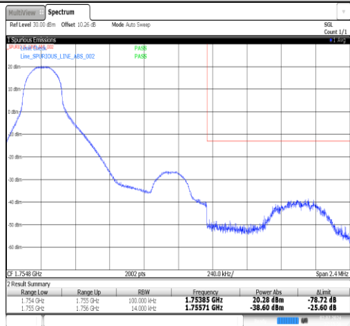
Band4-1.4MHz-16QAM-20393-1RB#5-PASS
