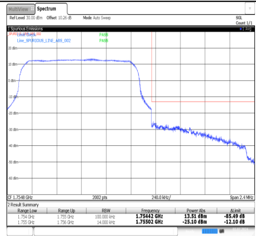
Band4-1.4MHz-QPSK-20393-6RB#5-PASS
