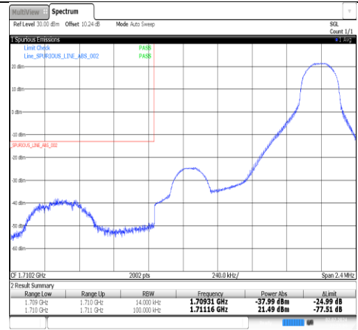
Band4-1.4MHz-QPSK-20393-6RB#0-PASS
