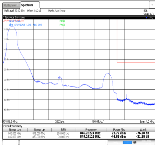
Band5-3MHz-QPSK-20635-1RB#14-PASS
