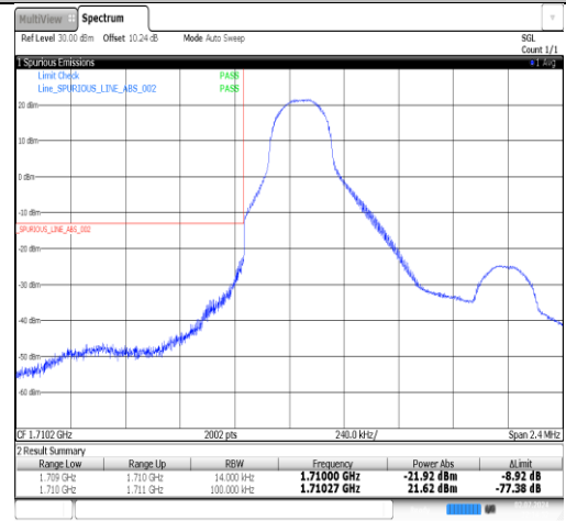
Band4-1.4MHz-QPSK-19957-1RB#0-PASS
