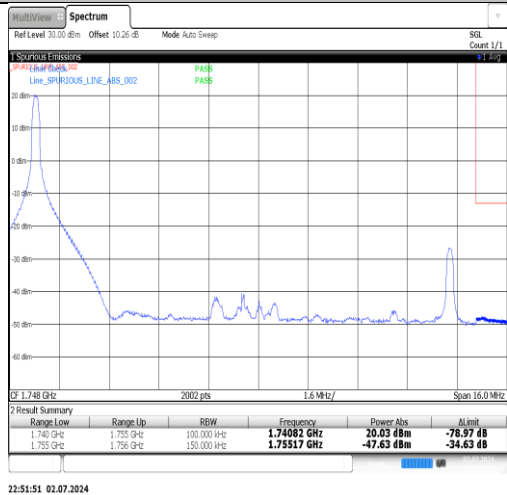
Band4-15MHz-16QAM-20325-1RB#74-PASS
