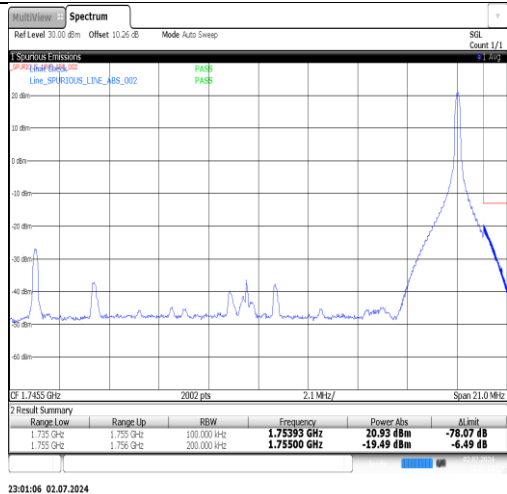
Band4-20MHz-16QAM-20050-100RB#0-PASS
