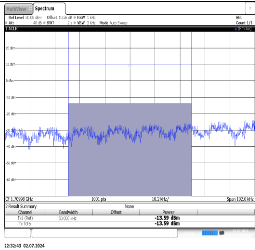
Band4-5MHz-QPSK-19975-1RB#24-PASS
