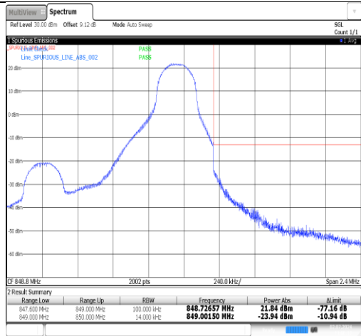
Band5-3MHz-QPSK-20415-15RB#0-PASS
