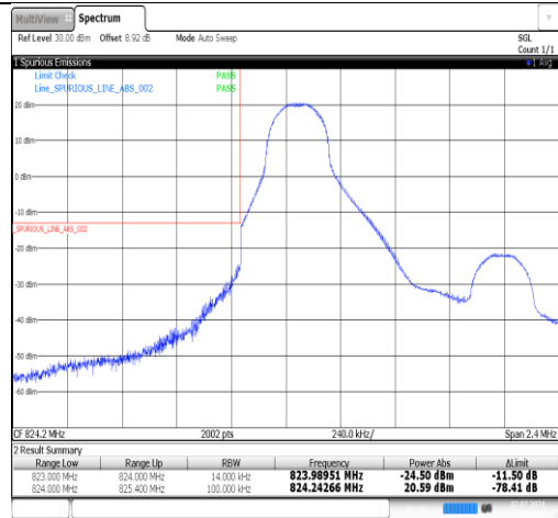
Band5-1.4MHz-16QAM-20407-1RB#5-PASS
