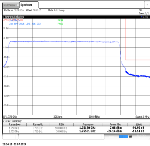
Band4-5MHz-QPSK-20375-1RB#24-Final_1 Integration method
