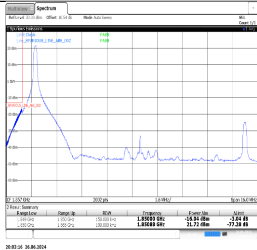
Band2-15MHz-QPSK-18675-1RB#74-PASS
