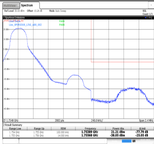
Band4-1.4MHz-QPSK-20393-1RB#5-PASS
