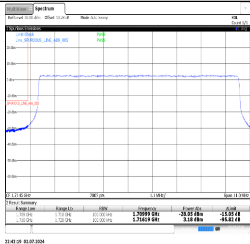
Band4-10MHz-16QAM-20350-1RB#0-PASS
