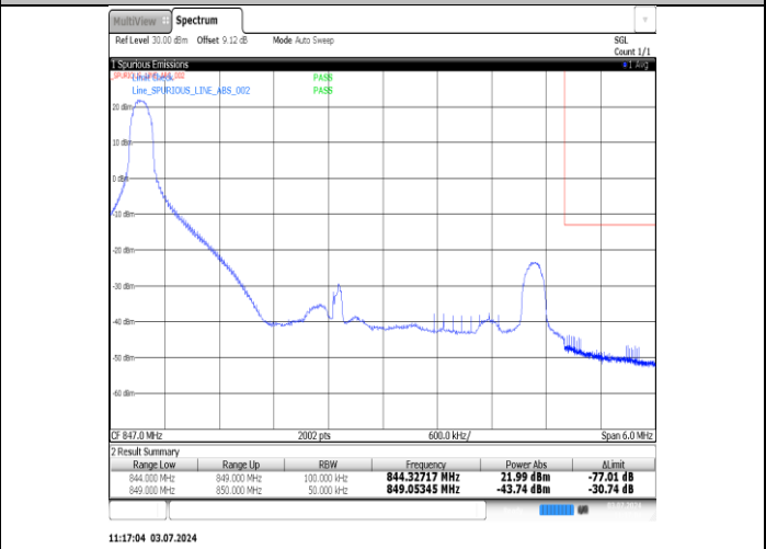
Band5-5MHz-16QAM-20625-1RB#24-PRELIMINARY
