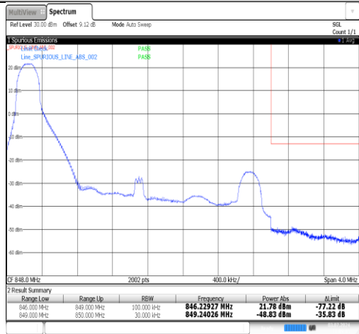
Band5-3MHz-16QAM-20635-1RB#14-PASS
