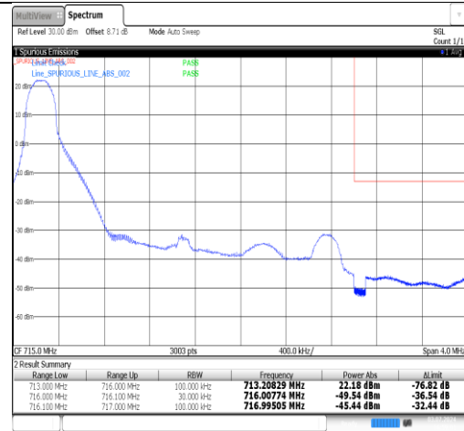
Band12-3MHz-QPSK-23165-1RB#14-PASS
