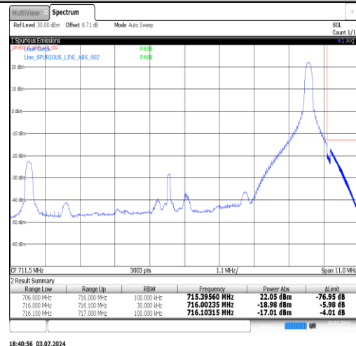
Band17-10MHz-16QAM-23780-50RB#0-PASS
