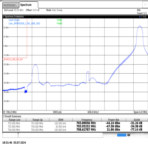
Band17-5MHz-QPSK-23825-25RB#0-PASS
