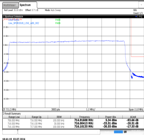
Band17-10MHz-16QAM-23780-1RB#0-PASS
