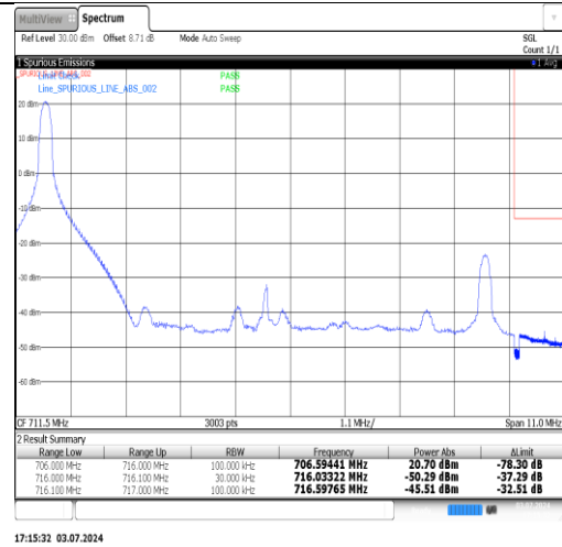
Band12-10MHz-16QAM-23130-1RB#49-PASS
