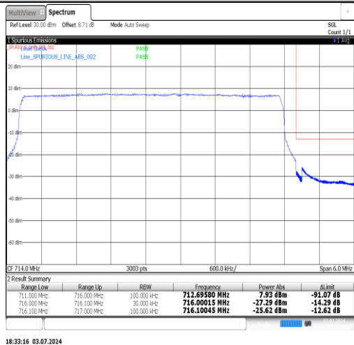
Band17-5MHz-16QAM-23755-1RB#0-PASS
