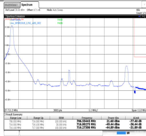
Band17-10MHz-QPSK-23800-1RB#49-PASS
