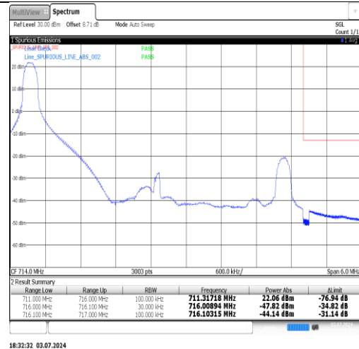
Band17-5MHz-QPSK-23825-1RB#24-PASS
