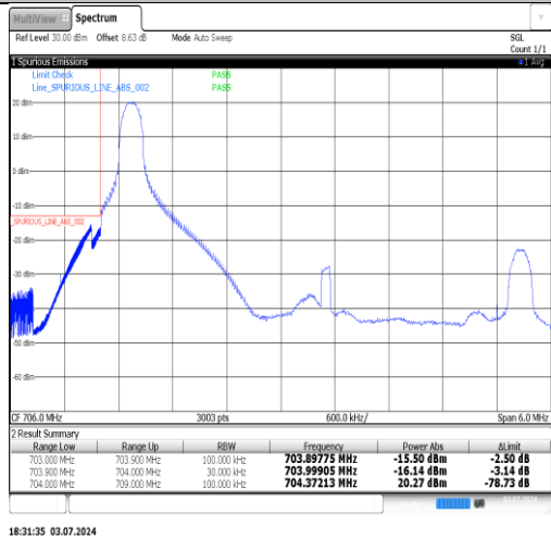
Band17-5MHz-16QAM-23755-1RB#24-PASS
