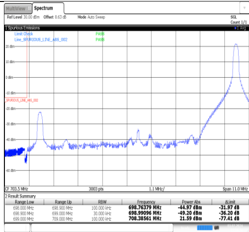
Band12-10MHz-QPSK-23130-50RB#0-PASS
