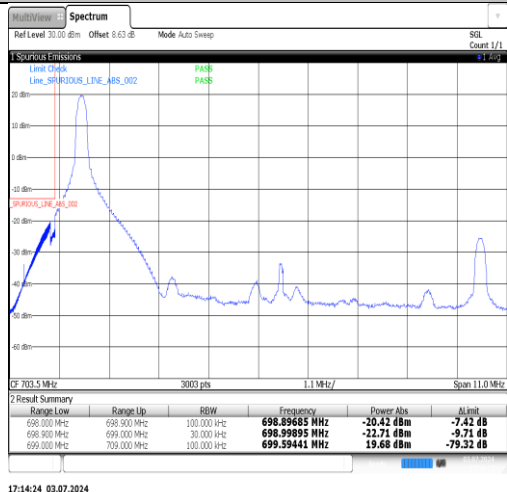
Band12-10MHz-16QAM-23060-1RB#49-PASS
