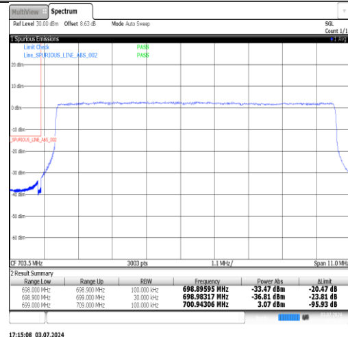
Band12-10MHz-16QAM-23130-1RB#0-PASS
