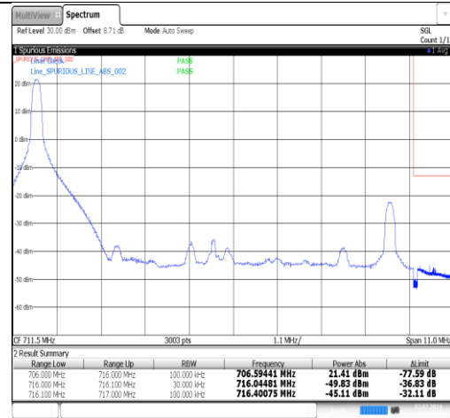
Band12-10MHz-QPSK-23130-1RB#49-PASS
