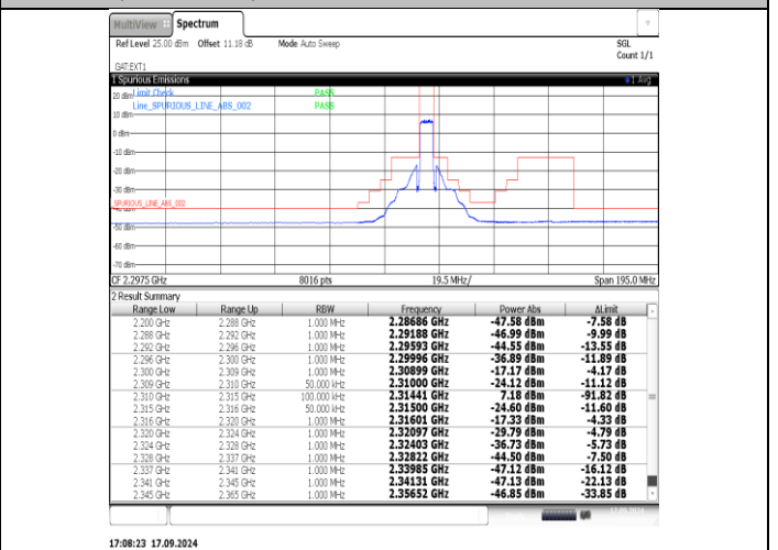
40(2305-2315)-5MHz-16QAM-38725-1RB#0-PASS
