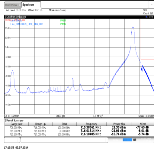
Band17-5MHz-QPSK-23755-25RB#0-PASS
