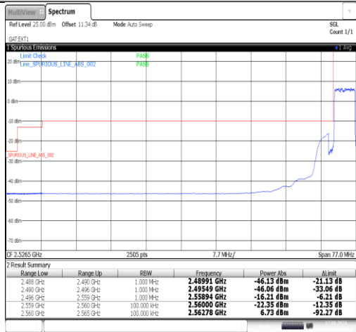
Band41-5MHz-QPSK-40315-25RB#0-PASS
