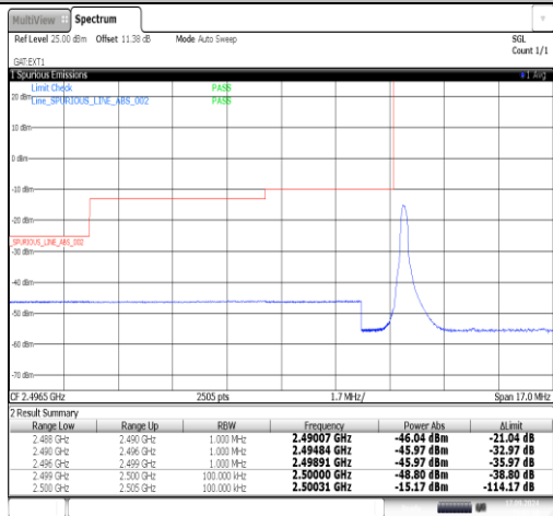
Band41-5MHz-QPSK-39715-1RB#0-PASS
