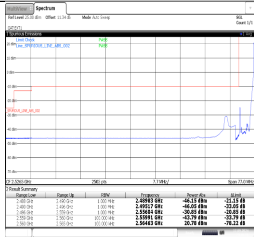
Band41-5MHz-QPSK-40315-1RB#24-PASS
