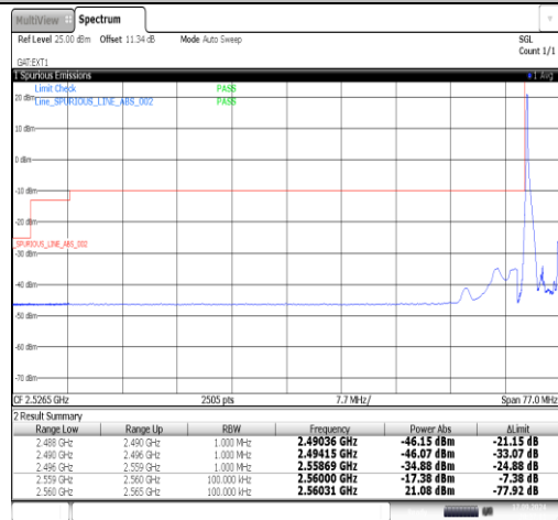
Band41-5MHz-QPSK-40315-1RB#0-PASS
