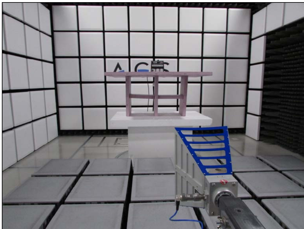
Figure 2: 48VDC Host - Front
