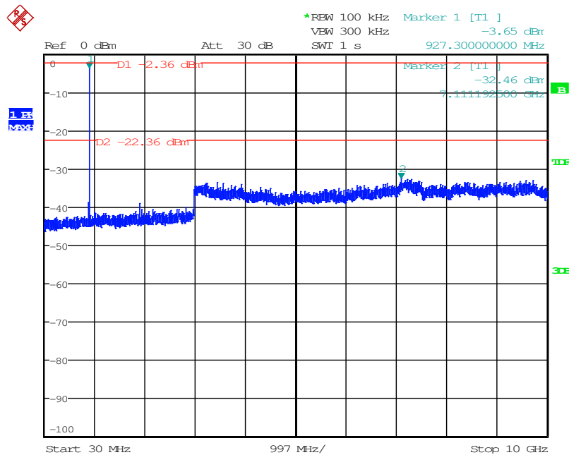
Figure 7.4.2.2-3: 30 MHz – 10 GHz –Middle Channel
