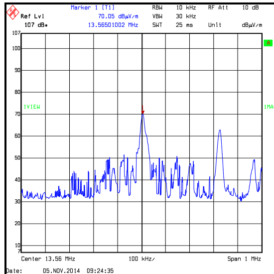
13.56 MHz reference unit signal at 3 metres on an open field test site on 05 November 2014
