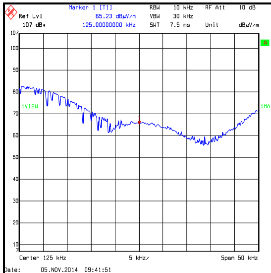
125 kHz reference unit signal at 3 metres on an open field test site on 05 November 2014
