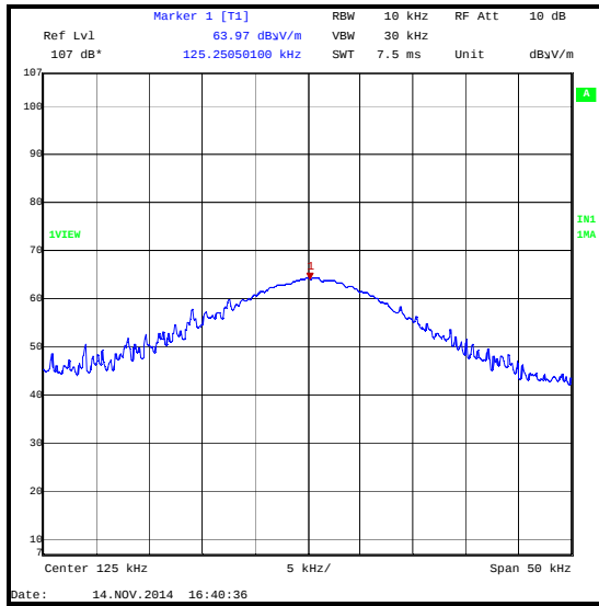
125 kHz reference unit signal at 3 metres in a semi-anechoic chamber on 14 November 2014
