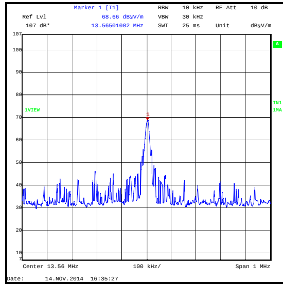
13.56 MHz reference unit signal at 3 metres in a semi-anechoic chamber on 14 November 2014
