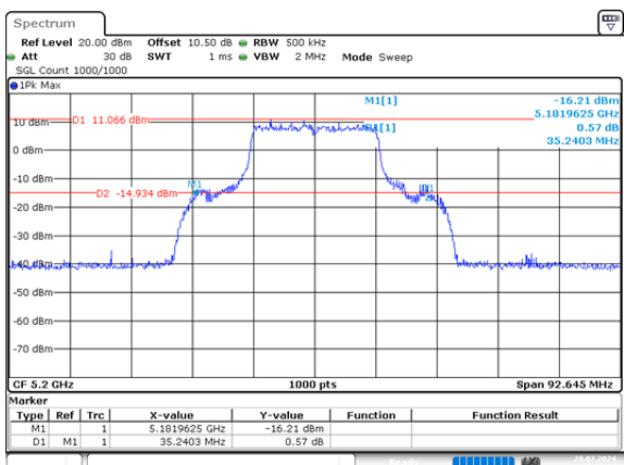
ax20_5200MHz_RU_Full_Chain 1 35.240MHz
