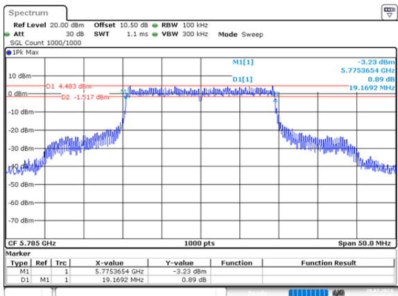
ax20_5785MHz_RU_Full_Chain 1 19.169MHz
