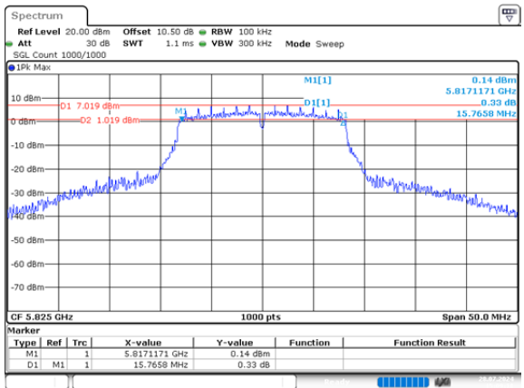
a_5825MHz_Chain 1 15.766MHz
