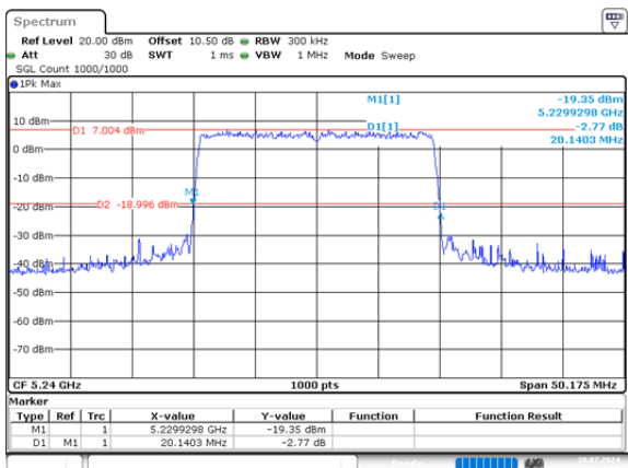
ax20_5240MHz_RU_Full_Chain 1 20.140MHz
