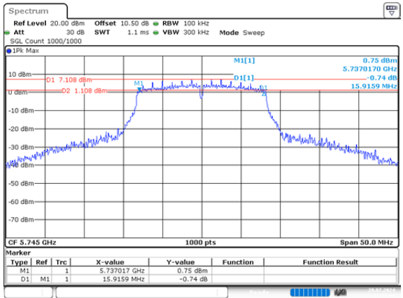
a_5745MHz_Chain 1 15.916MHz
