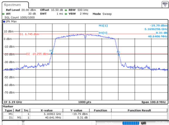
n40_5190MHz_Chain 0 40.641MHz
