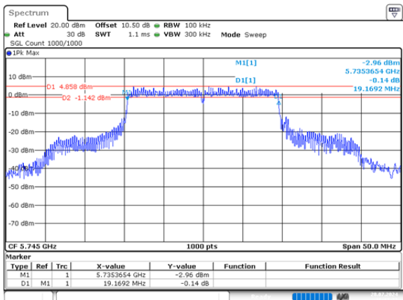
ax20_5745MHz_RU_Full_Chain 1 19.169MHz
