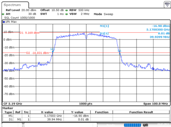
n40_5190MHz_Chain 1 39.940MHz
