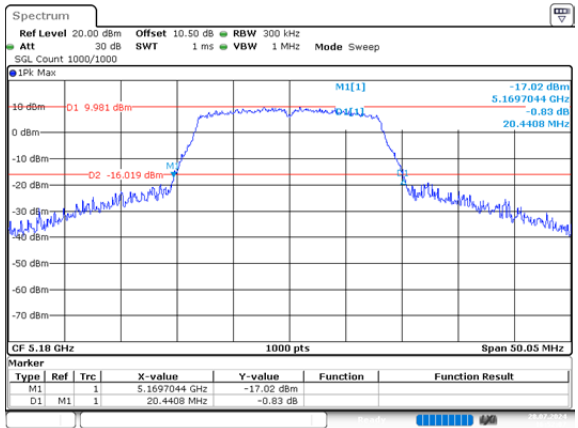
a_5180MHz_Chain 1 20.441MHz
