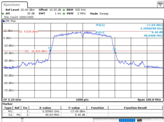
n40_5230MHz_Chain 1 40.040MHz
