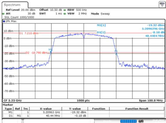
n40_5230MHz_Chain 0 40.440MHz
