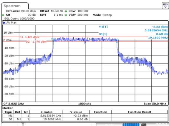
ax20_5825MHz_RU_Full_Chain 1 19.169MHz
