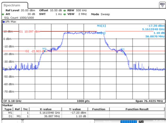
ax20_5180MHz_RU_Full_Chain 1 36.887MHz
