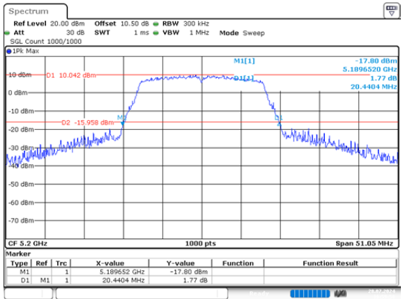
a_5200MHz_Chain 1 20.440MHz
