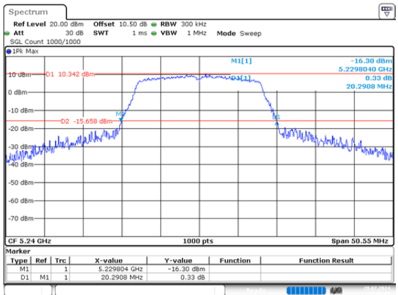
a_5240MHz_Chain 1 20.291MHz
