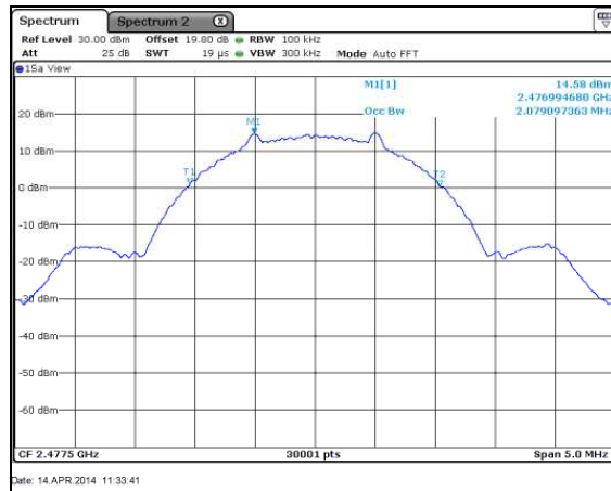
Figure 7.3.2-12: 99% Bandwidth Plot – 2477.5 MHz
