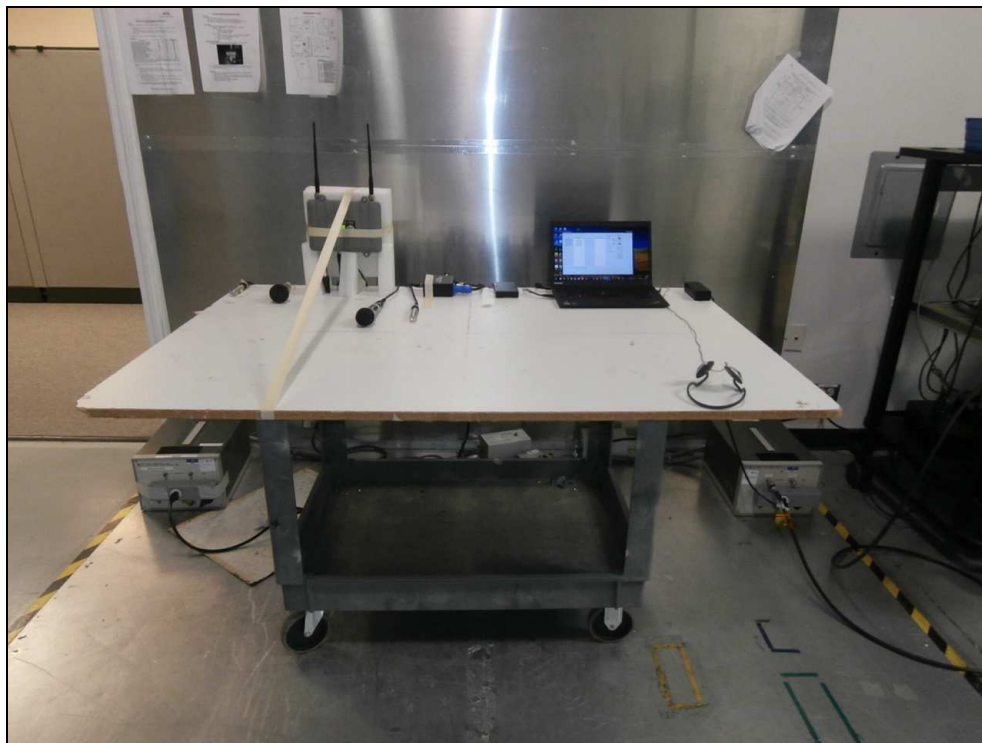
Figure 7: Test Setup Photo – Conducted Emissions – Breakout Box Computer Configuration
