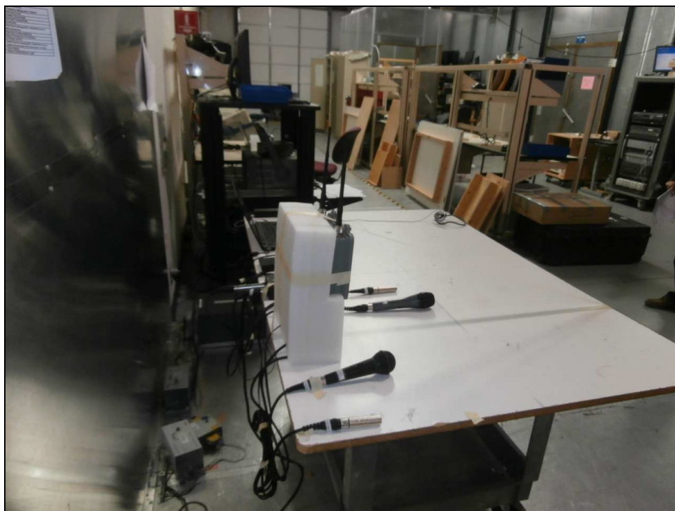
Figure 8: Test Setup Photo – Conducted Emissions – Breakout Box Computer Configuration
