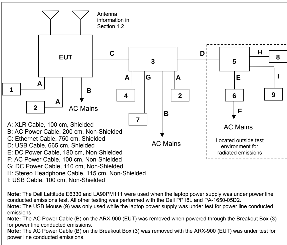
Figure 6-1: EUT Test Setup – Radiated and Conducted Emissions
