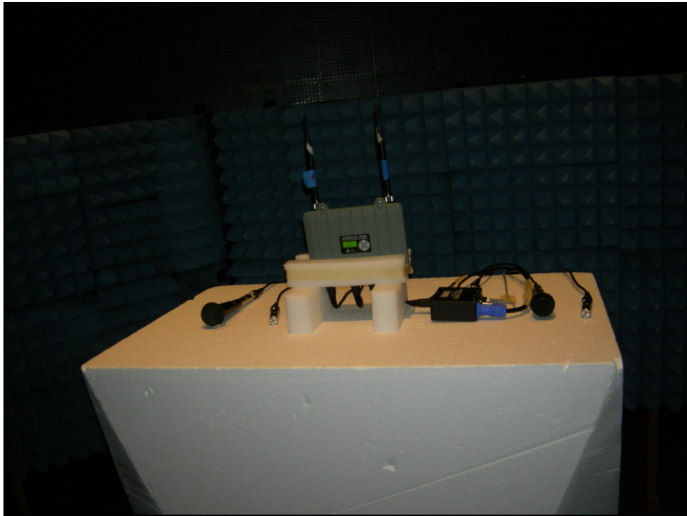
Figure 1: Radiated Emissions – Dipole Antennas
