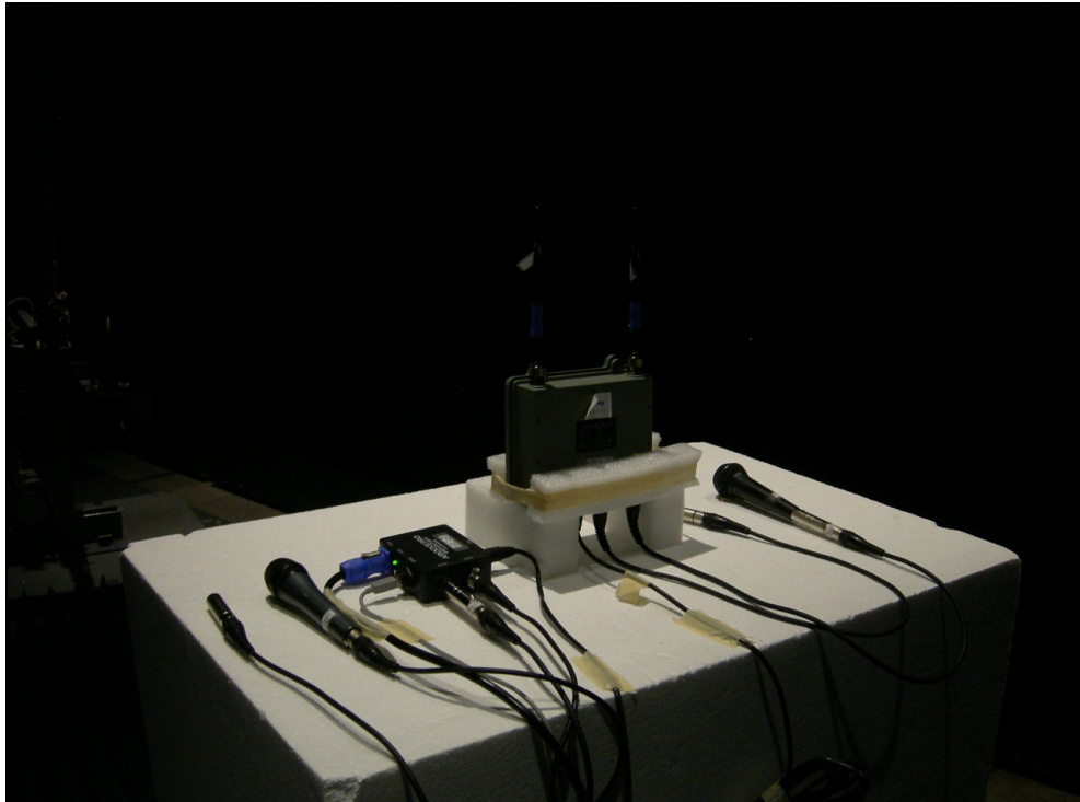
Figure 2: Radiated Emissions – Dipole Antennas
