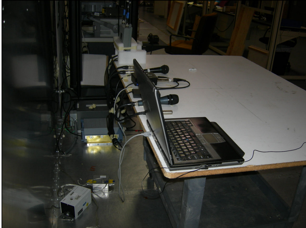
Figure 6: Conducted Emissions – AiRocks Configuration
