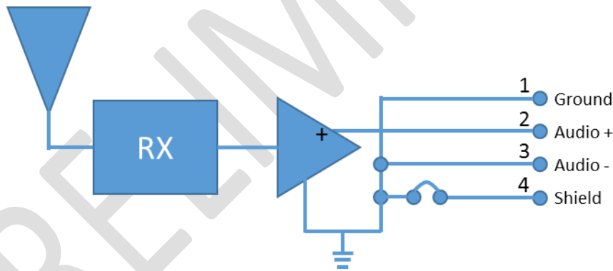
Figure 9 Unbalanced Mono Audio Output Connector Configuration
