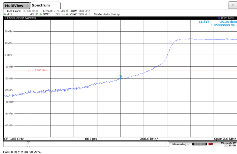
Band2-10MHz-QPSK-18650-Full RB#
