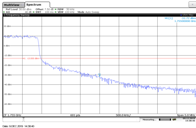
Band4-3MHz-16QAM-20385-Full RB#
