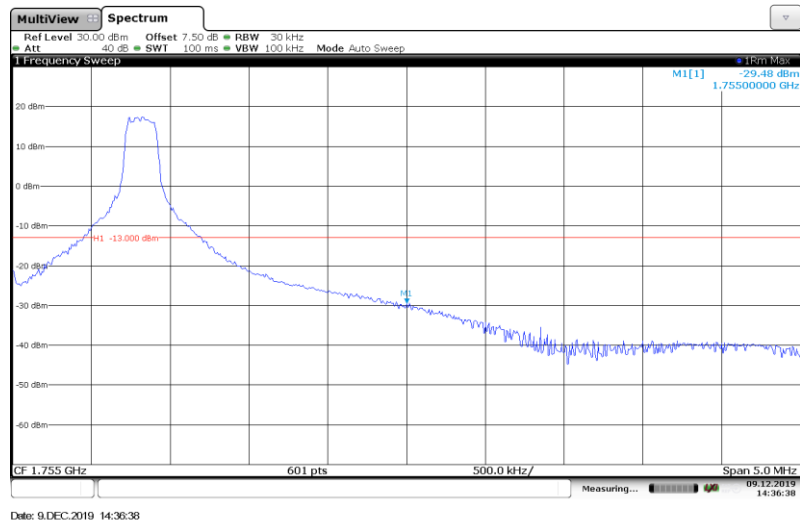
Band4-3MHz-QPSK-20385-1RB#
