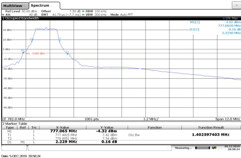
Band13-10MHz-16QAM-23230
