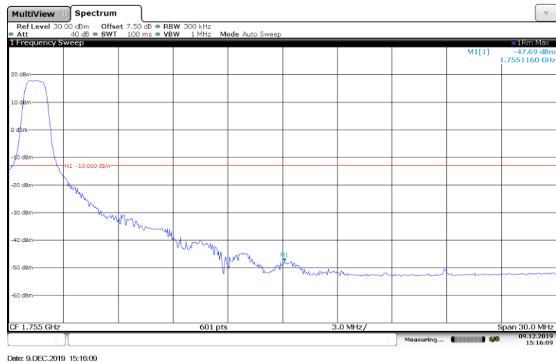
Band4-15MHz-QPSK-20325-Full RB#
