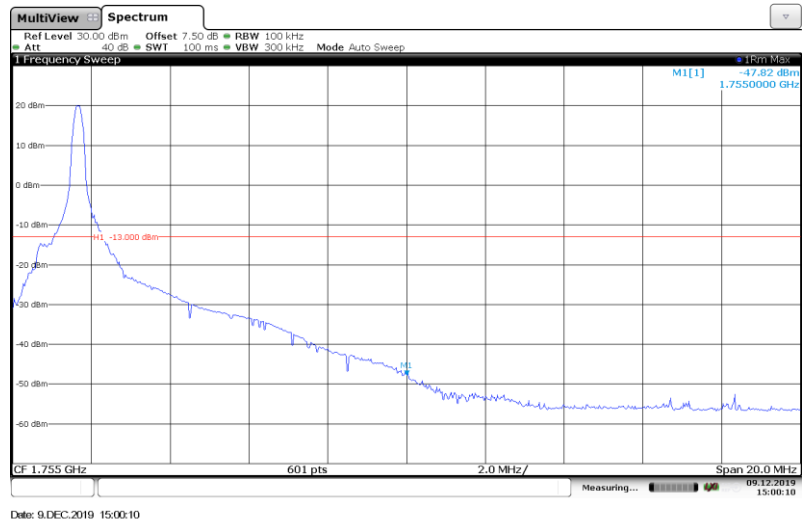
Band4-10MHz-16QAM-20350-1RB#
