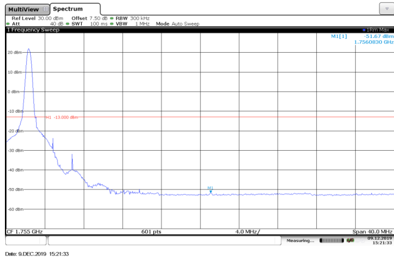
Band4-20MHz-16QAM-20300-1RB#
