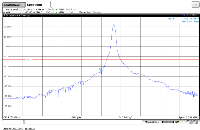
Band4-15MHz-QPSK-20025-1RB#
