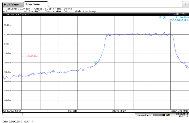
Band12-1.4MHz-QPSK-23017-Full RB#
