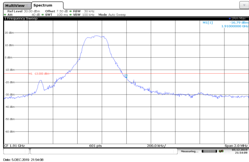
Band2-1.4MHz-16QAM-19193-1RB#
