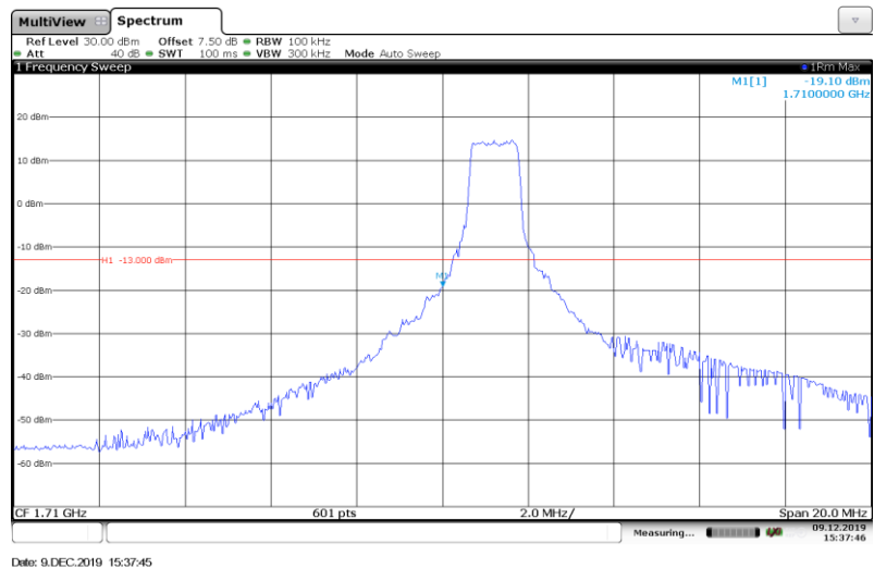
Band4-10MHz-16QAM-20000-Full RB#
