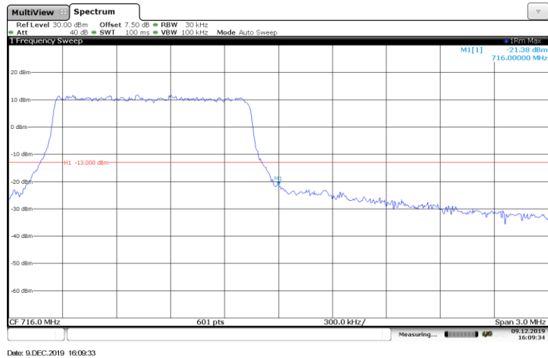
Band12-1.4MHz-QPSK-23173-Full RB#
