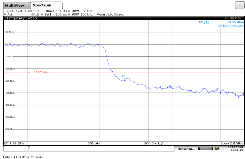
Band2-1.4MHz-QPSK-19193-Full RB#
