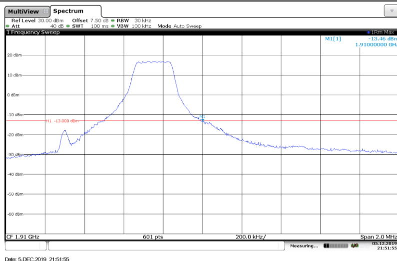
Band2-1.4MHz-QPSK-19193-1RB#
