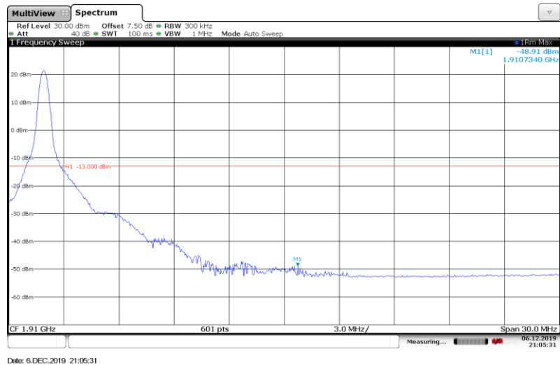
Band2-15MHz-QPSK-19125-1RB#
