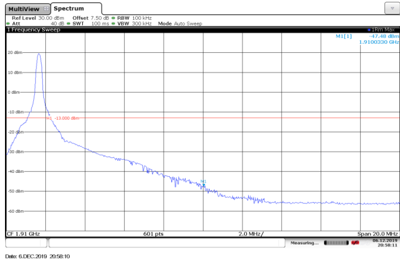
Band2-10MHz-16QAM-19150-1RB#
