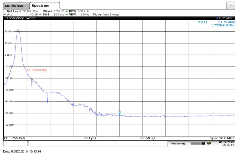
Band4-15MHz-16QAM-20325-1RB#
