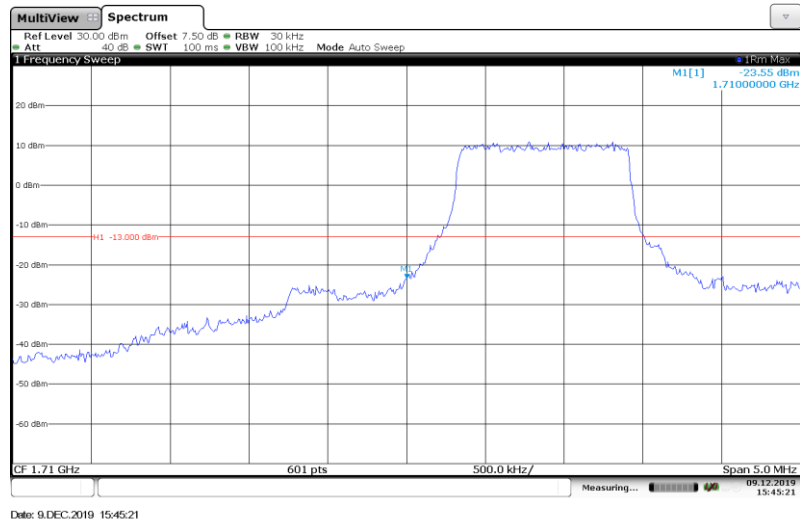
Band4-3MHz-QPSK-19965-Full RB#
