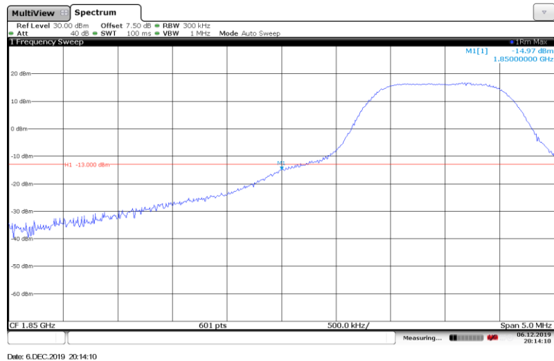
Band2-15MHz-16QAM-18675-Full RB#0
