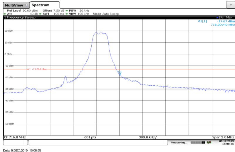
Band12-1.4MHz-QPSK-23173-1RB#
