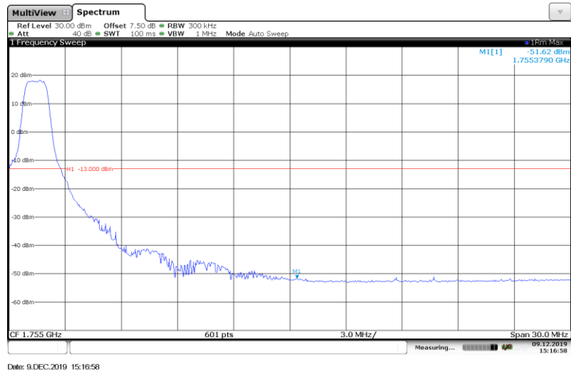
Band4-15MHz-16QAM-20325-Full RB#
