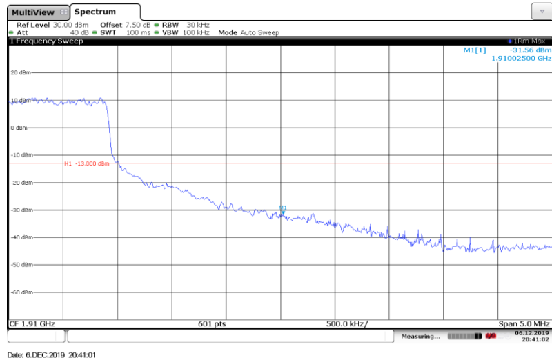
Band2-3MHz-16QAM-19185-Full RB#
