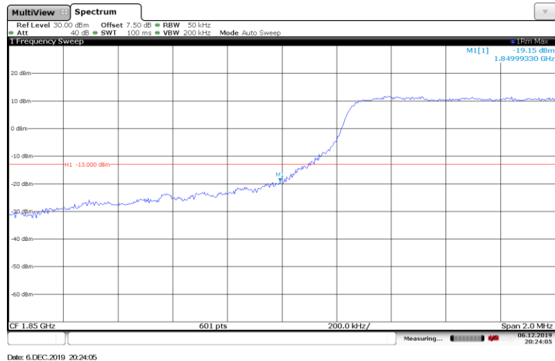
Band2-5MHz-QPSK-18625-Full RB#
