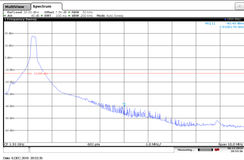
Band2-5MHz-16QAM-19175-1RB#
