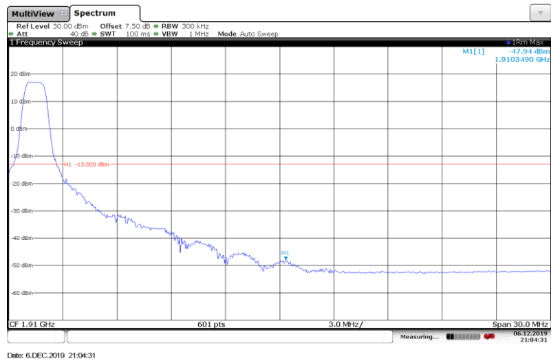
Band2-15MHz-QPSK-19125-Full RB#
