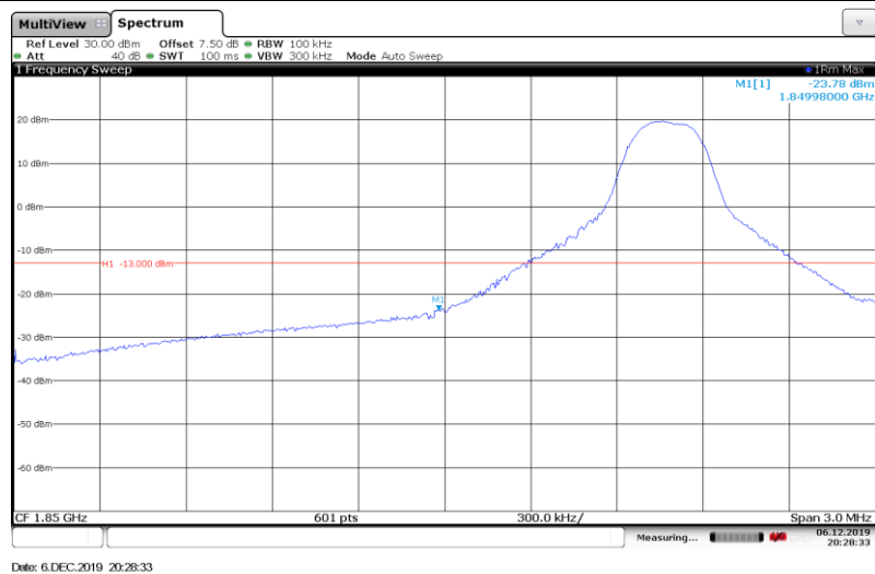
Band2-10MHz-16QAM-18650-1RB#
