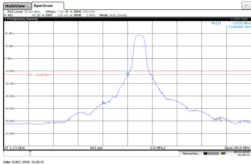
Band4-15MHz-16QAM-20025-Full RB#
