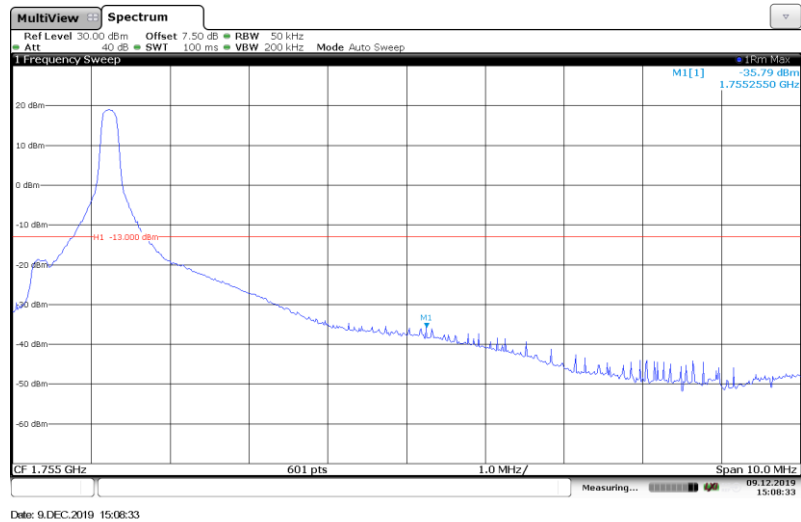
Band4-5MHz-QPSK-20375-1RB#
