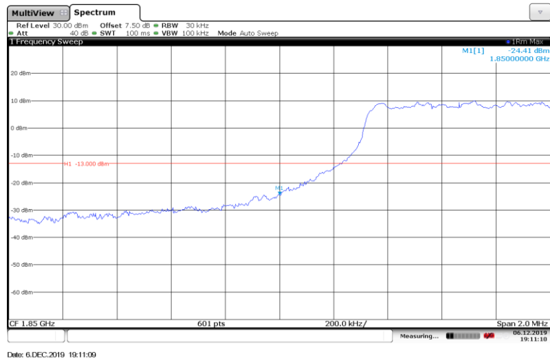
Band2-3MHz-16QAM-18615-Full RB#
