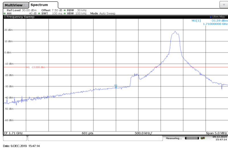
Band4-3MHz-16QAM-19965-1RB#
