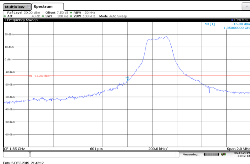
Band2-1.4MHz-QPSK-18607-1RB#
