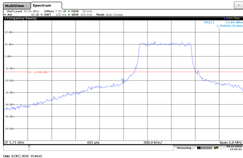
Band4-3MHz-16QAM-19965-Full RB#
