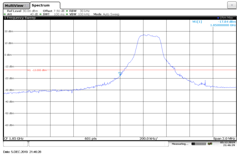
Band2-1.4MHz-16QAM-18607-1RB#
