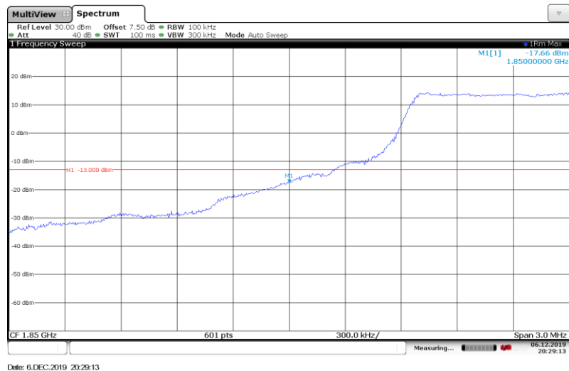
Band2-10MHz-16QAM-18650-Full RB#
