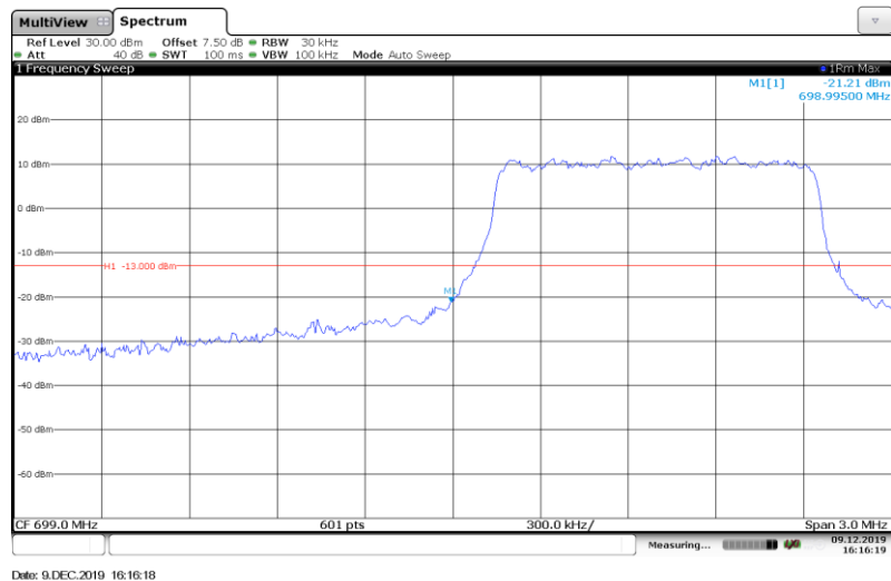
Band12-1.4MHz-16QAM-23017-Full RB#
