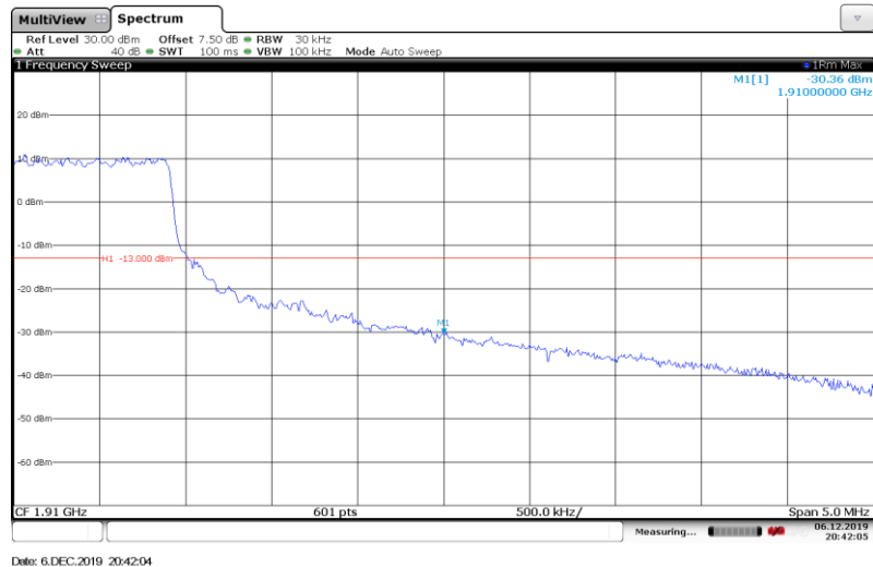
Band2-3MHz-QPSK-19185-Full RB#
