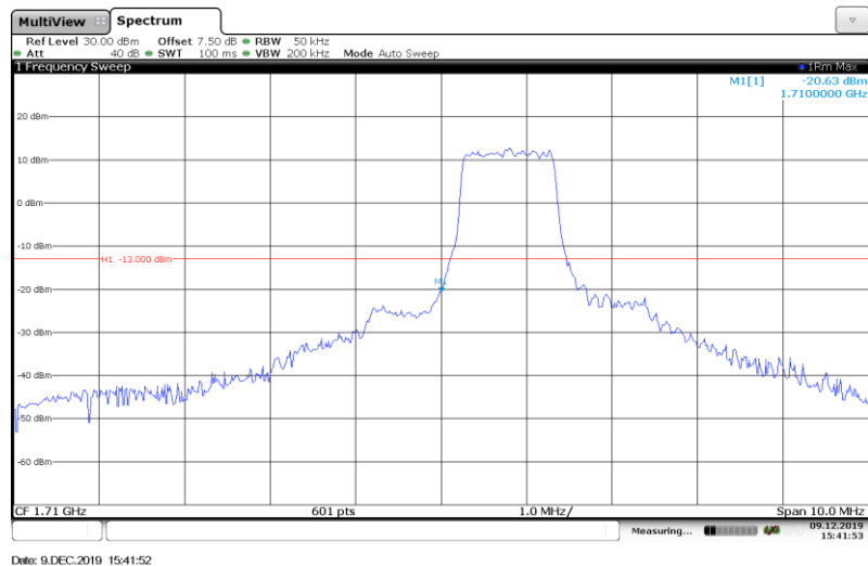
Band4-5MHz-QPSK-19975-Full RB#
