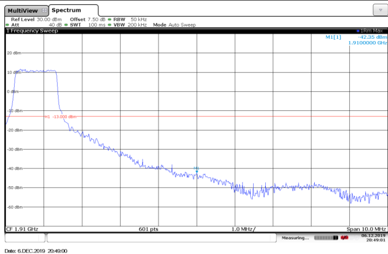
Band2-5MHz-QPSK-19175-Full RB#
