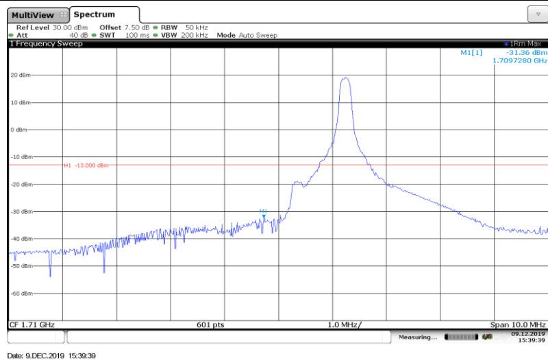
Band4-5MHz-QPSK-19975-1RB#
