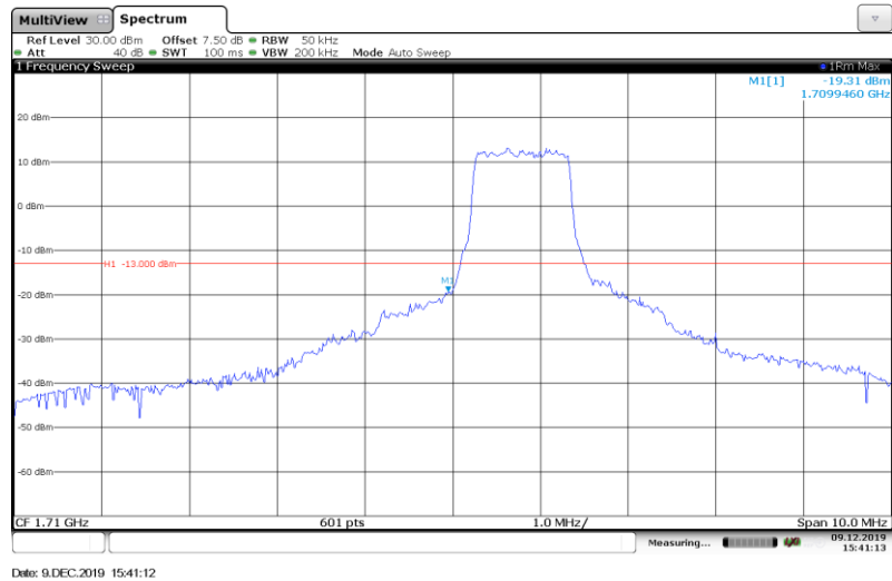
Band4-5MHz-16QAM-19975-Full RB#
