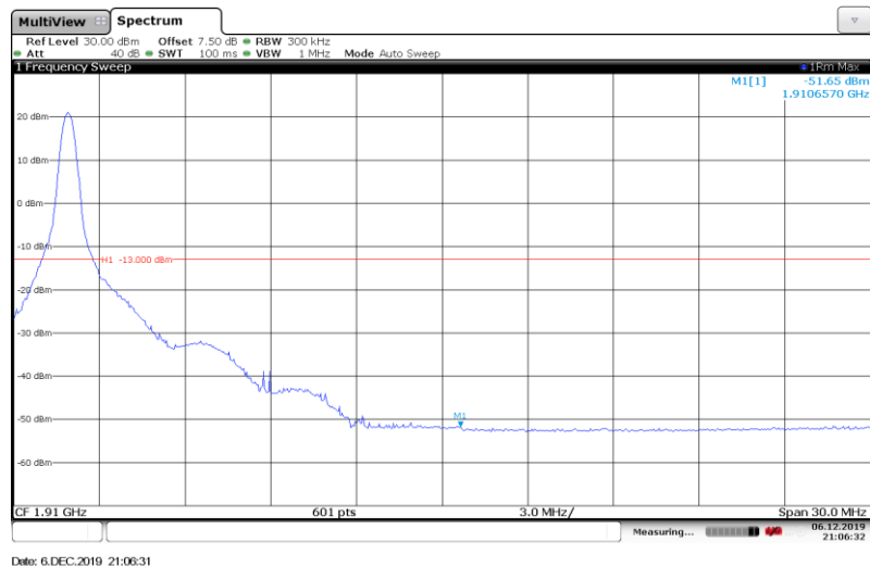
Band2-15MHz-16QAM-19125-1RB#
