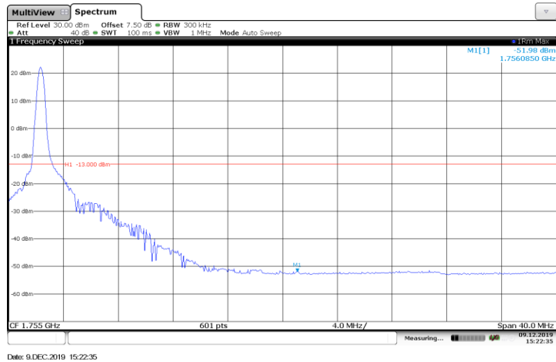
Band4-20MHz-QPSK-20300-1RB#
