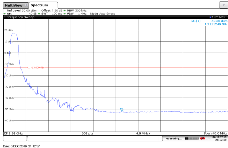
Band2-20MHz-QPSK-19100-Full RB#
