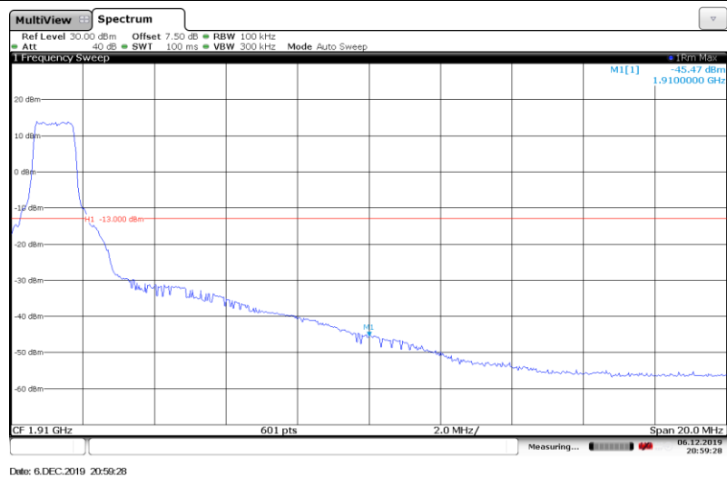
Band2-10MHz-16QAM-19150-Full RB#
