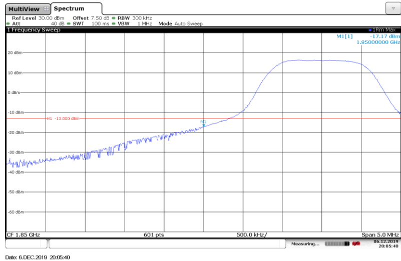
Band2-15MHz-QPSK-18675-Full RB#
