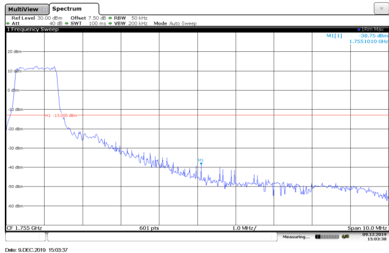
Band4-5MHz-QPSK-20375-Full RB#
