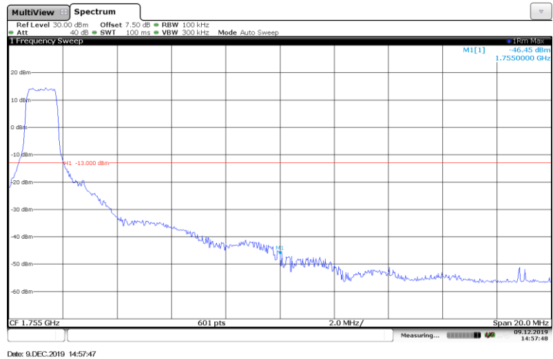
Band4-10MHz-QPSK-20350-Full RB#
