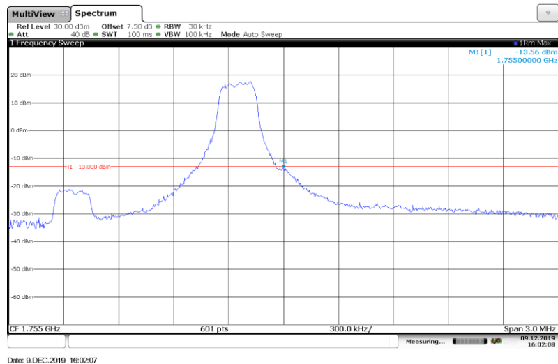
Band4-1.4MHz-QPSK-20393-1RB#
