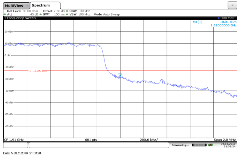
Band2-1.4MHz-16QAM-19193-Full RB#
