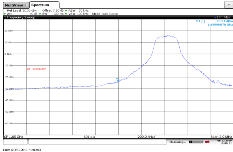
Band2-3MHz-16QAM-18615-1RB#
