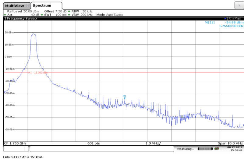
Band4-5MHz-16QAM-20375-1RB#
