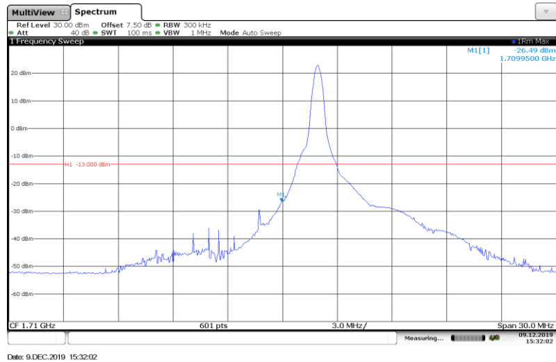
Band4-15MHz-16QAM-20025-1RB#
