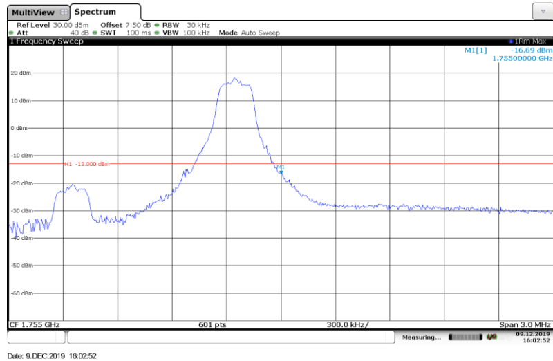
Band4-1.4MHz-16QAM-20393-1RB#
