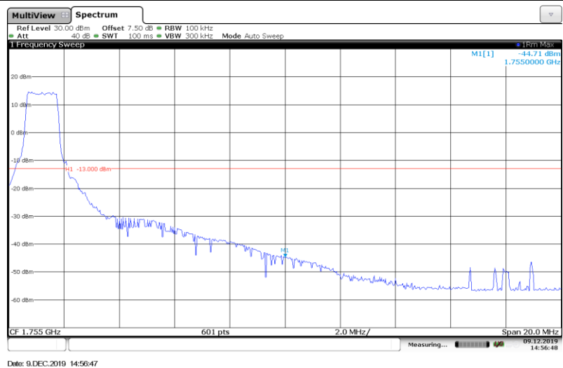
Band4-10MHz-16QAM-20350-Full RB#
