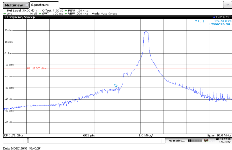
Band4-5MHz-16QAM-19975-1RB#0
