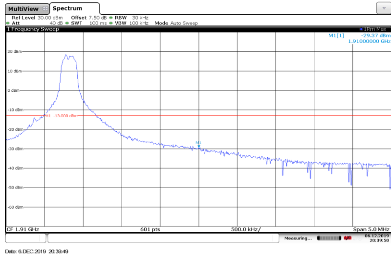
Band2-3MHz-16QAM-19185-1RB#
