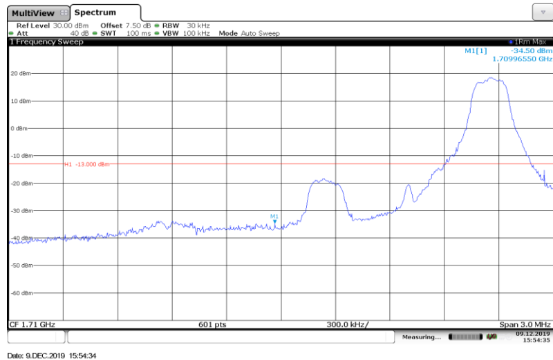
Band4-1.4MHz-16QAM-19957-1RB#
