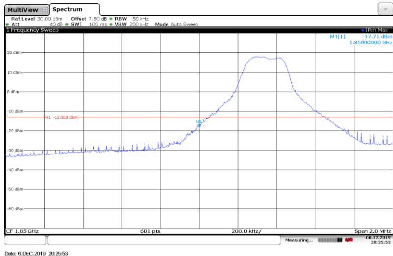
Band2-5MHz-16QAM-18625-1RB#
