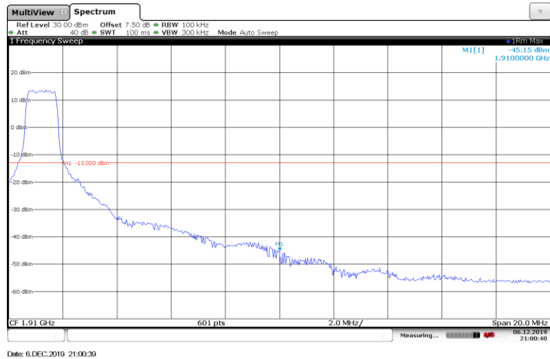
Band2-10MHz-QPSK-19150-Full RB#
