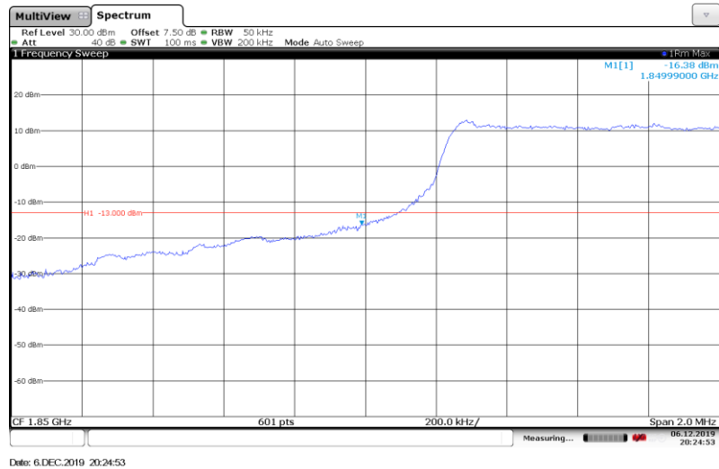
Band2-5MHz-16QAM-18625-Full RB#
