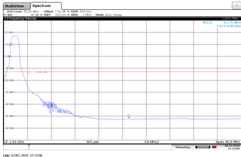
Band2-20MHz-16QAM-19100-Full RB#
