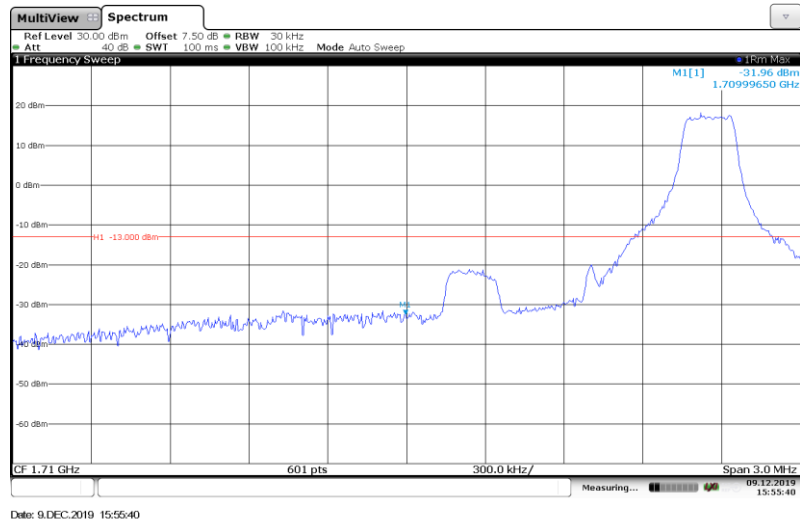
Band4-1.4MHz-QPSK-19957-1RB#
