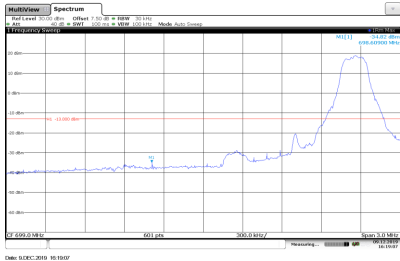
Band12-1.4MHz-16QAM-23017-1RB#
