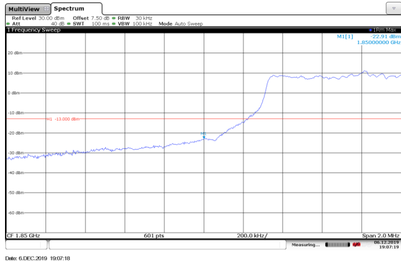
Band2-3MHz-QPSK-18615-Full RB#
