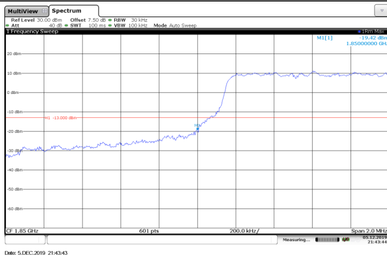
Band2-1.4MHz-QPSK-18607-Full RB#
