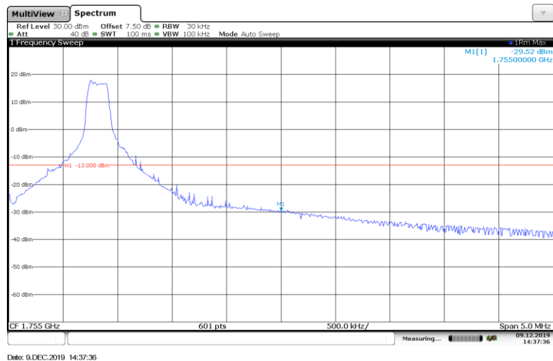
Band4-3MHz-16QAM-20385-1RB#
