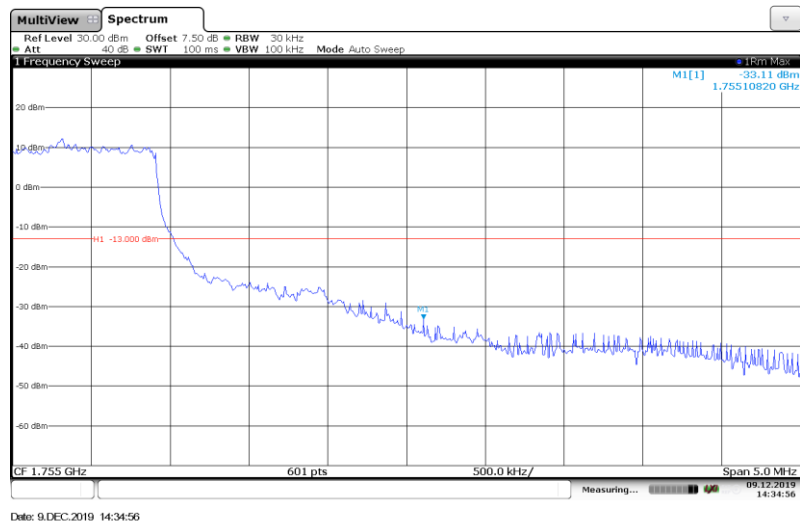
Band4-3MHz-QPSK-20385-Full RB#
