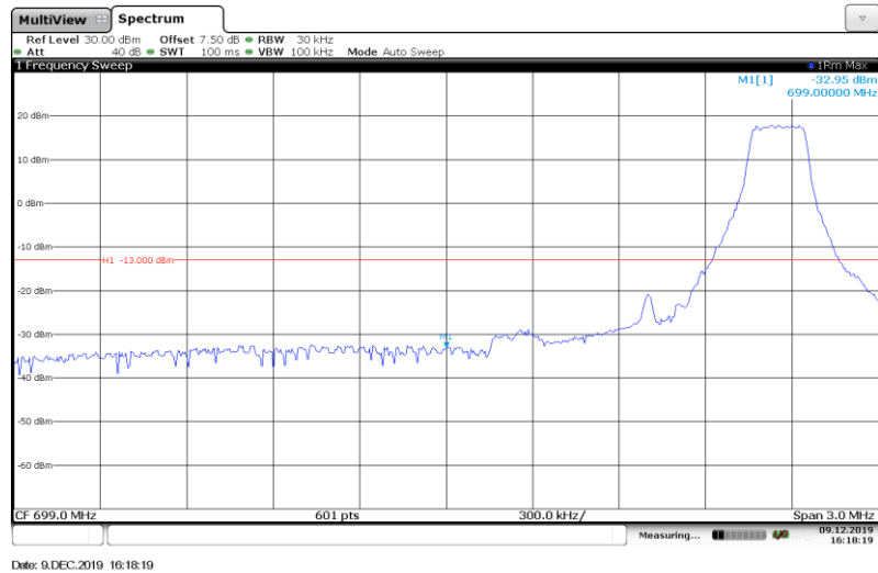
Band12-1.4MHz-QPSK-23017-1RB#
