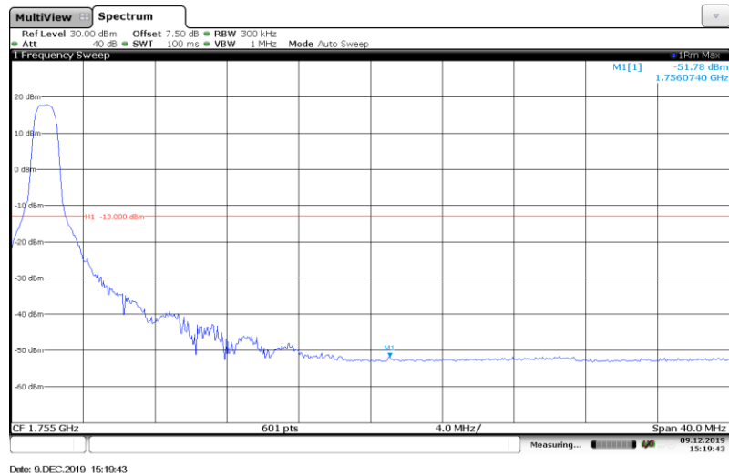
Band4-20MHz-QPSK-20300-Full RB#
