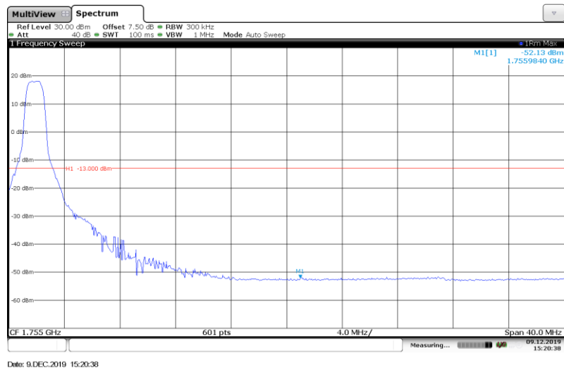
Band4-20MHz-16QAM-20300-Full RB#
