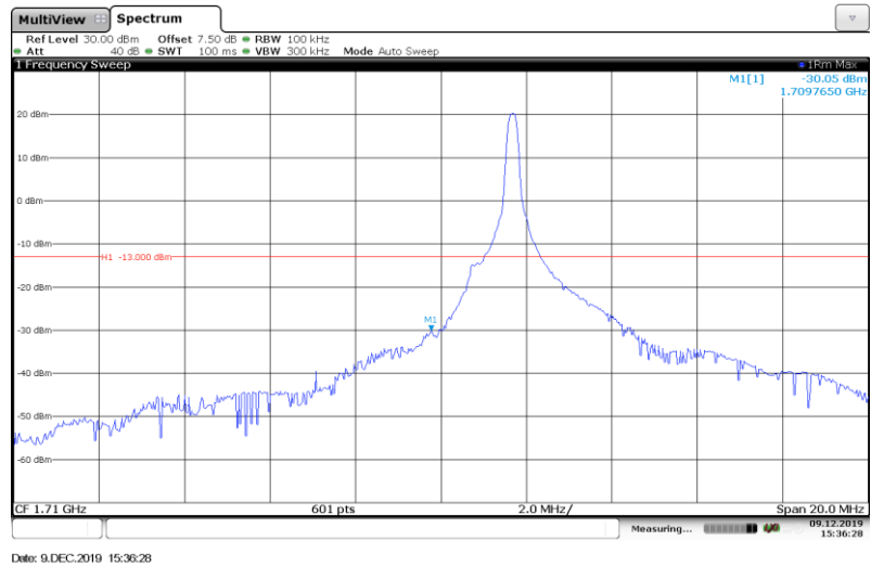
Band4-10MHz-QPSK-20000-1RB#
