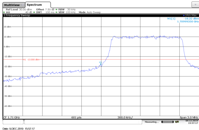
Band4-1.4MHz-16QAM-19957-Full RB#
