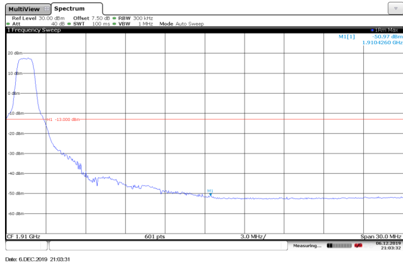
Band2-15MHz-16QAM-19125-Full RB#
