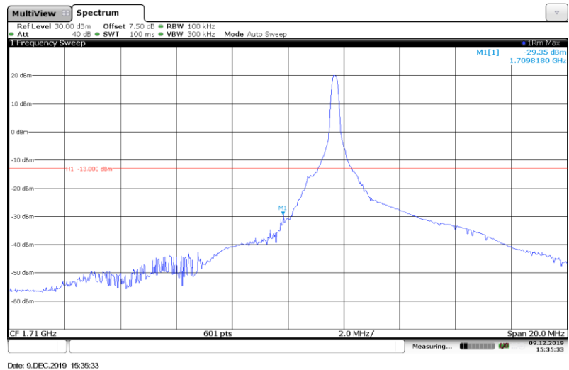
Band4-10MHz-16QAM-20000-1RB#
