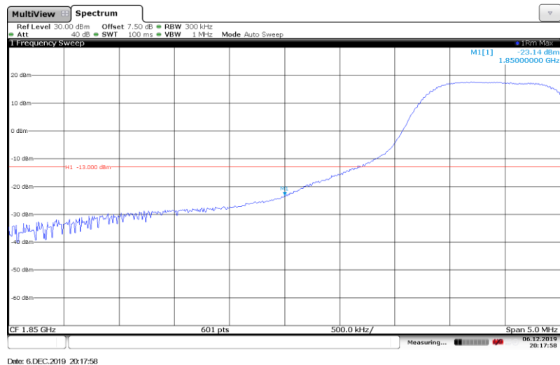
Band2-20MHz-QPSK-18700-Full RB#
