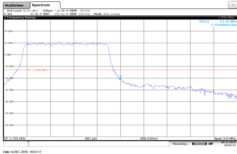
Band4-1.4MHz-QPSK-20393-Full RB#
