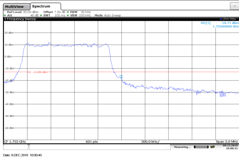
Band4-1.4MHz-16QAM-20393-Full RB#
