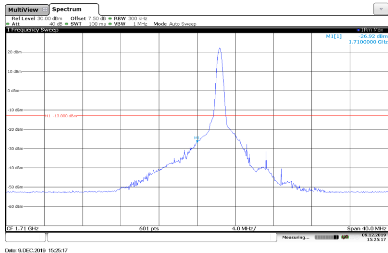
Band4-20MHz-16QAM-20050-1RB#
