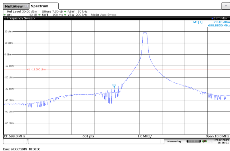
Band12-5MHz-QPSK-23035-1RB#
