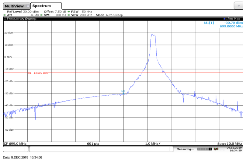
Band12-5MHz-16QAM-23035-1RB#
