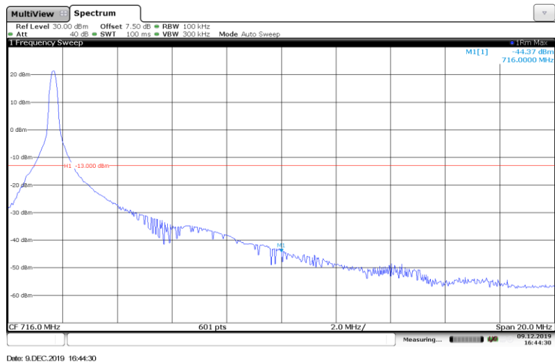
Band12-10MHz-QPSK-23130-1RB#
