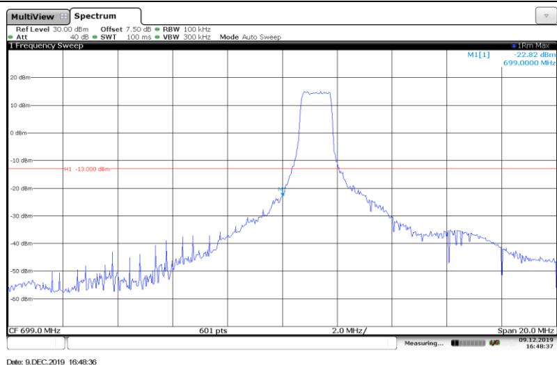
Band12-10MHz-QPSK-23060-Full RB#
