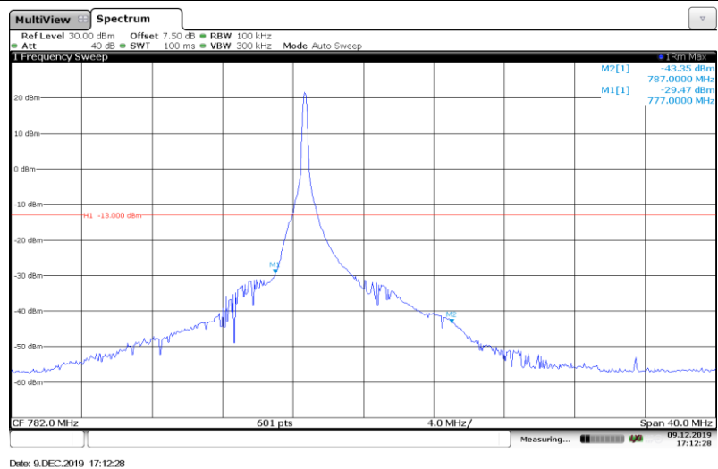
Band13-10MHz-QPSK-23230-1RB#
