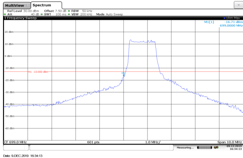
Band12-5MHz-16QAM-23035-Full RB#
