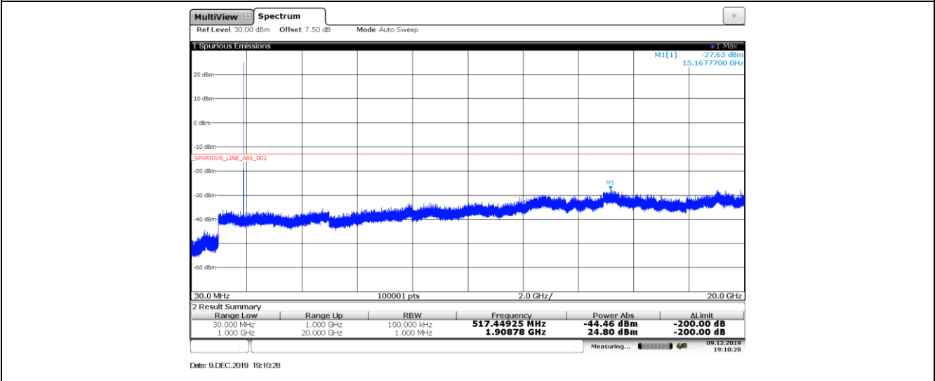
Band2-1.4MHz-QPSK-19193-1RB#
