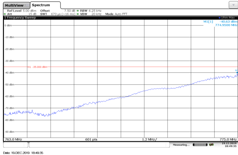
Band13-10MHz-QPSK-(763-775MHz)-Full RB#
