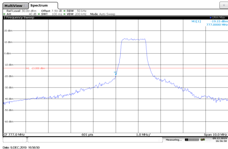
Band13-5MHz-QPSK-23205-Full RB#
