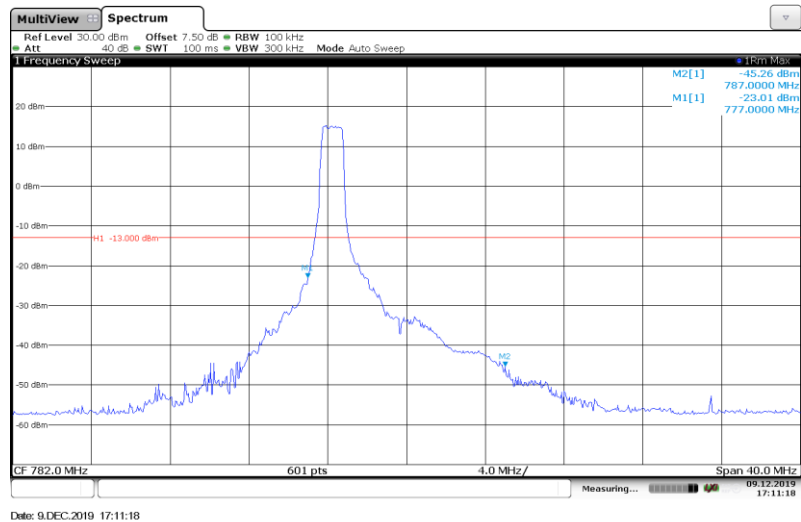
Band13-10MHz-QPSK-23230-Full RB#
