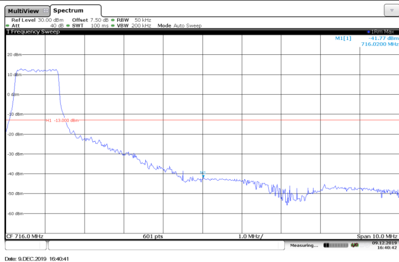
Band12-5MHz-QPSK-23155-Full RB#
