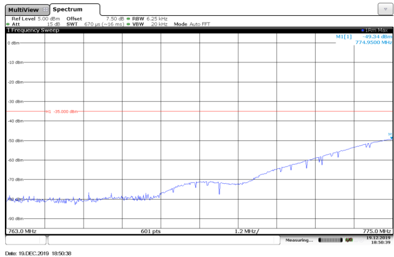
Band13-10MHz-QPSK-(763-775MHz)-1RB#
