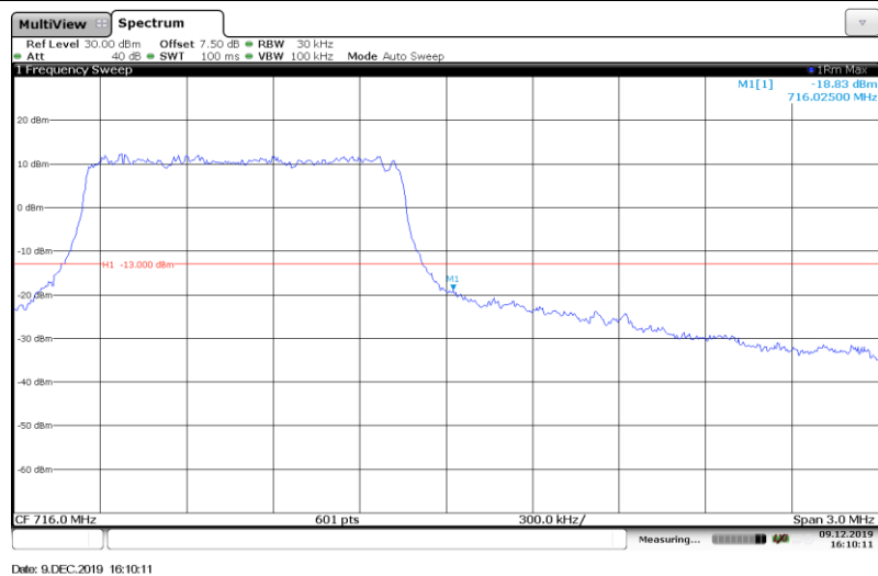
Band12-1.4MHz-16QAM-23173-Full RB#
