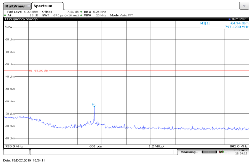
Band13-10MHz-16QAM-(793-805MHz)-Full RB#
