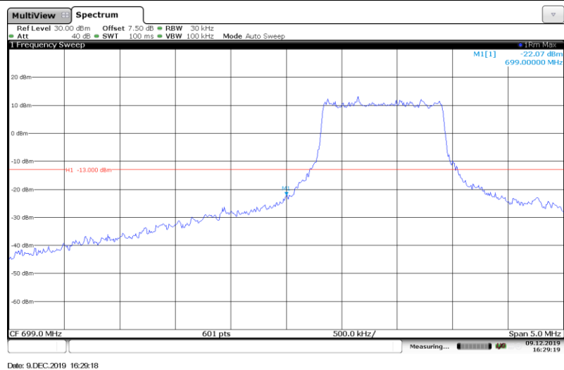
Band12-3MHz-16QAM-23025-Full RB#
