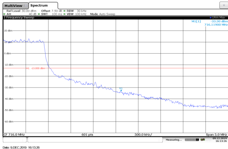
Band12-3MHz-QPSK-23165-Full RB#
