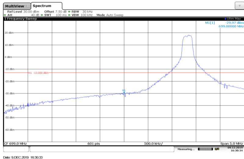
Band12-3MHz-QPSK-23025-1RB#
