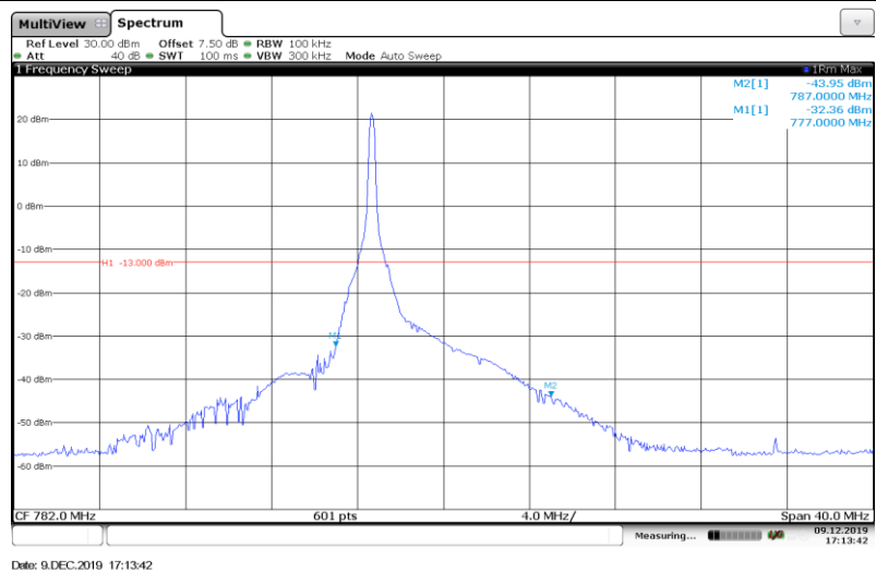
Band13-10MHz-16QAM-23230-1RB#
