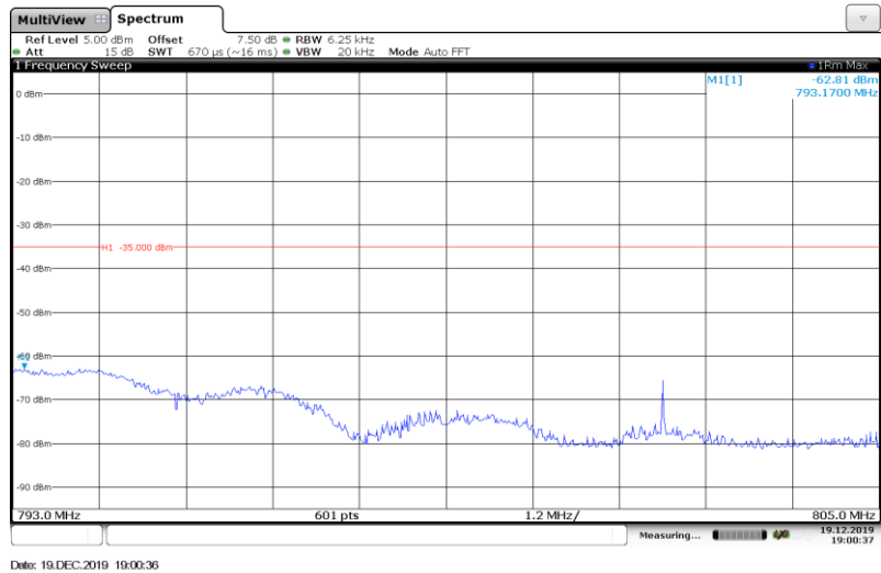
Band13-5MHz-QPSK-(793-805MHz)-Full RB#
