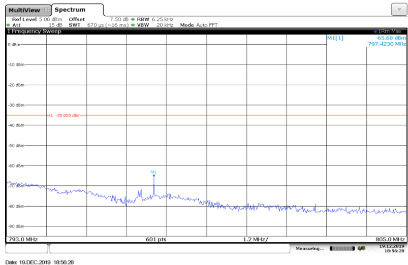
Band13-10MHz-QPSK-(793-805MHz)-1RB#
