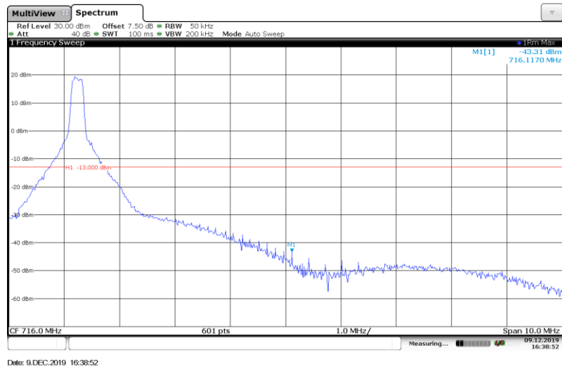
Band12-5MHz-16QAM-23155-1RB#
