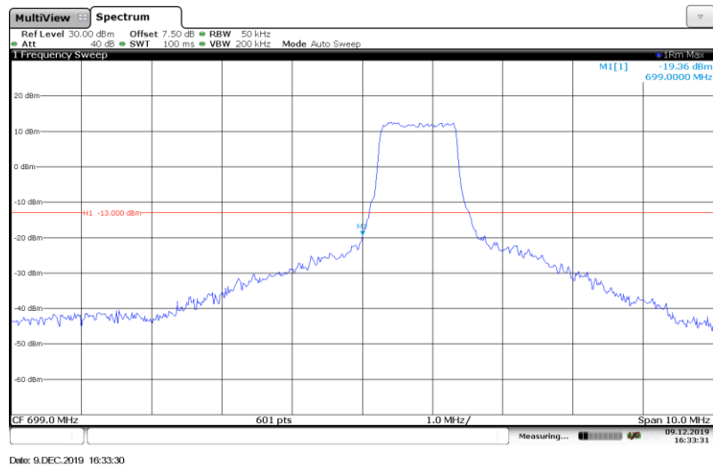
Band12-5MHz-QPSK-23035-Full RB#
