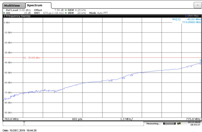
Band13-5MHz-16QAM-(763-775MHz)-1RB#
