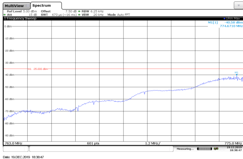
Band13-5MHz-QPSK-(763-775MHz)-Full RB#
