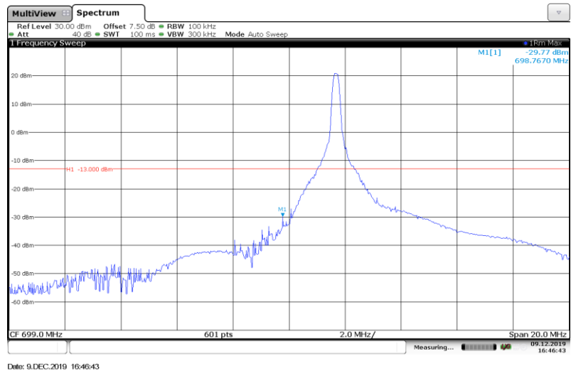
Band12-10MHz-16QAM-23060-1RB#
