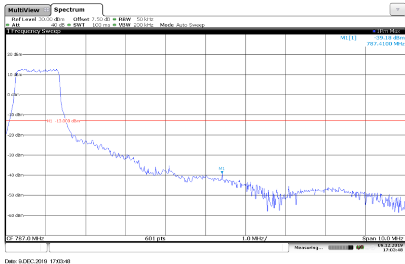
Band13-5MHz-QPSK-23255-Full RB#
