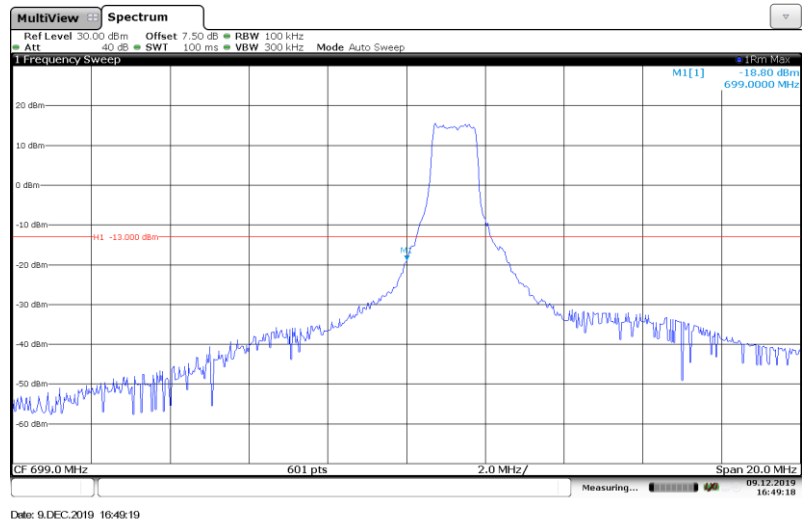
Band12-10MHz-16QAM-23060-Full RB#
