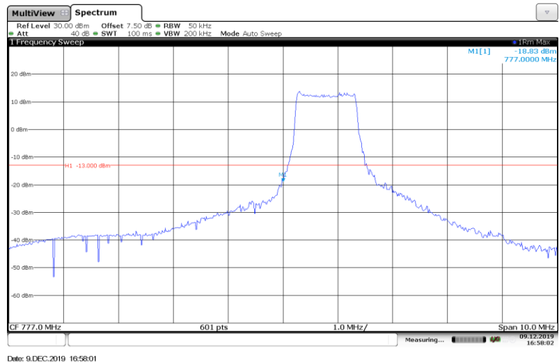
Band13-5MHz-16QAM-23205-Full RB#
