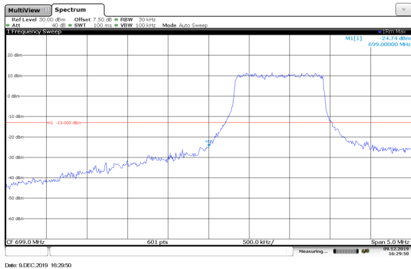
Band12-3MHz-QPSK-23025-Full RB#
