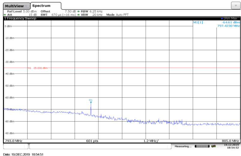
Band13-10MHz-16QAM-(793-805MHz)-1RB#
