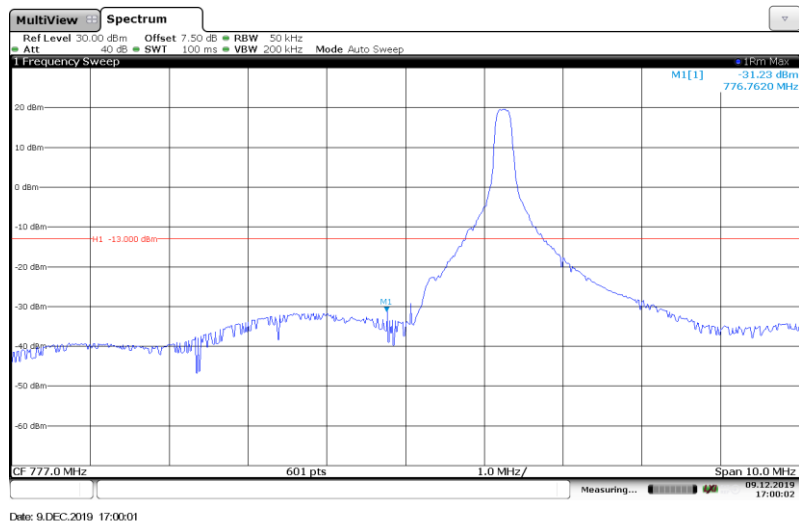
Band13-5MHz-QPSK-23205-1RB#
