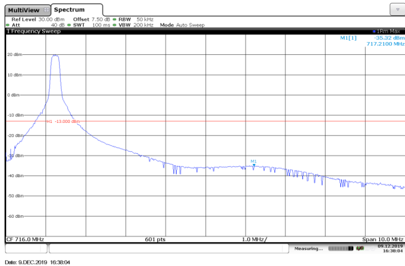
Band12-5MHz-QPSK-23155-1RB#
