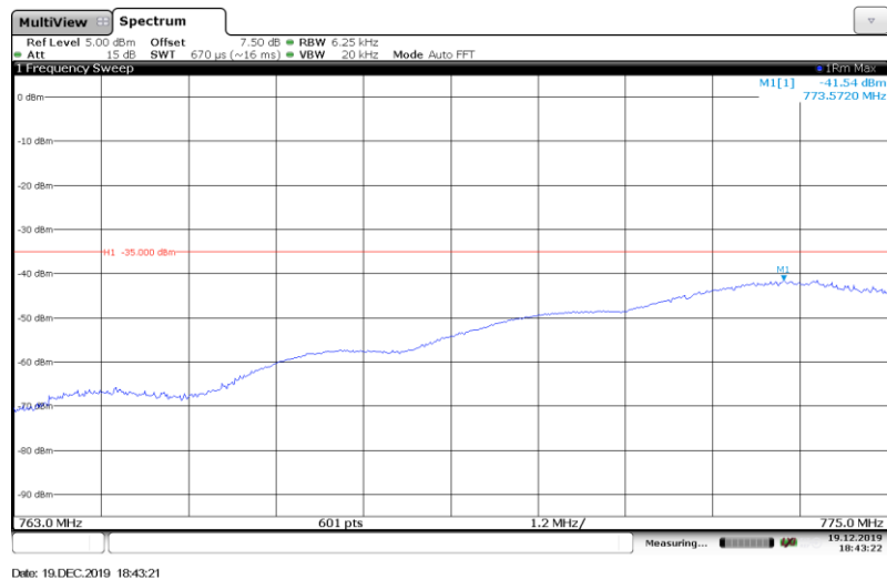
Band13-5MHz-QPSK-(763-775MHz)-1RB#
