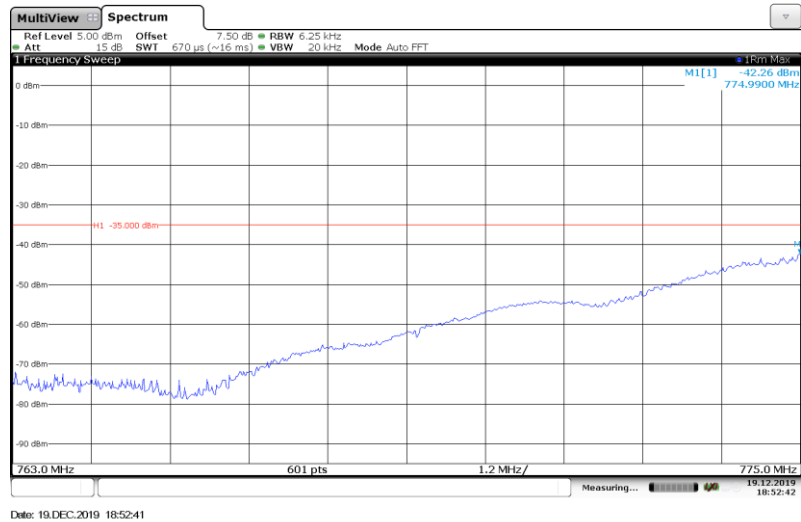
Band13-10MHz-16QAM-(763-775MHz)-Full RB#
