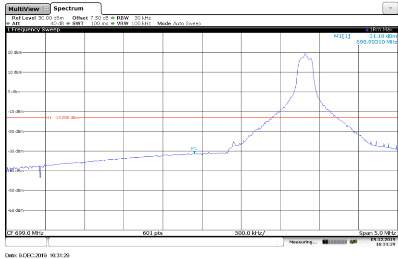
Band12-3MHz-16QAM-23025-1RB#
