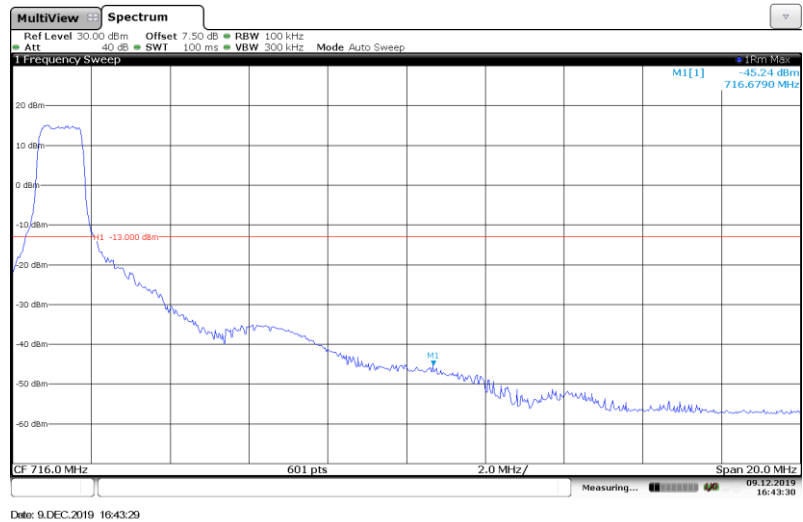
Band12-10MHz-QPSK-23130-Full RB#
