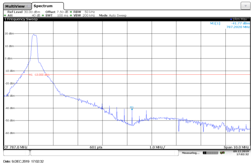
Band13-5MHz-16QAM-23255-1RB#
