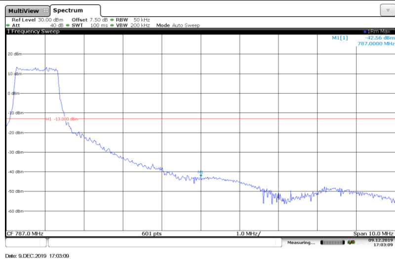
Band13-5MHz-16QAM-23255-Full RB#
