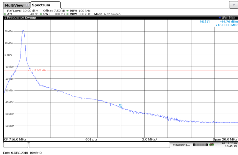
Band12-10MHz-16QAM-23130-1RB#
