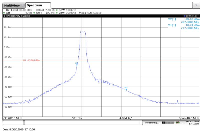
Band13-10MHz-16QAM-23230-Full RB#
