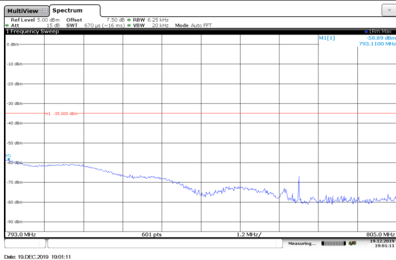
Band13-5MHz-QPSK-(793-805MHz)-1RB#
