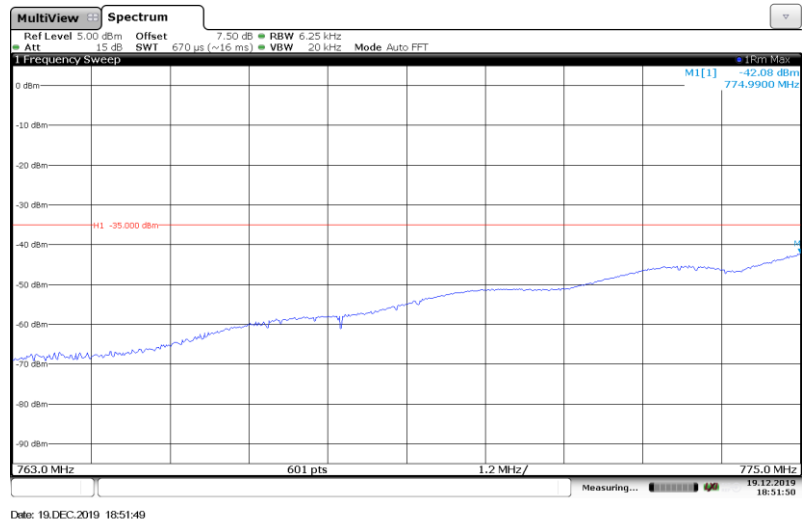
Band13-10MHz-16QAM-(763-775MHz)-1RB#
