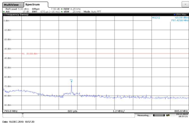
Band13-10MHz-QPSK-(793-805MHz)-Full RB#
