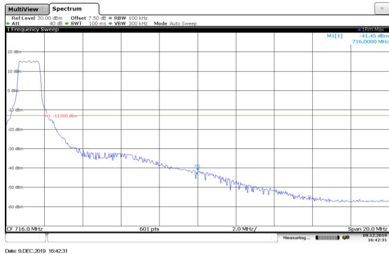
Band12-10MHz-16QAM-23130-Full RB#
