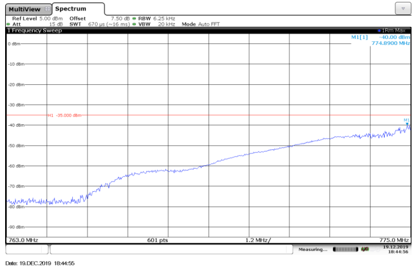
Band13-5MHz-16QAM-(763-775MHz)-Full RB#
