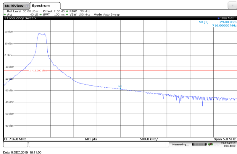
Band12-3MHz-16QAM-23165-1RB#
