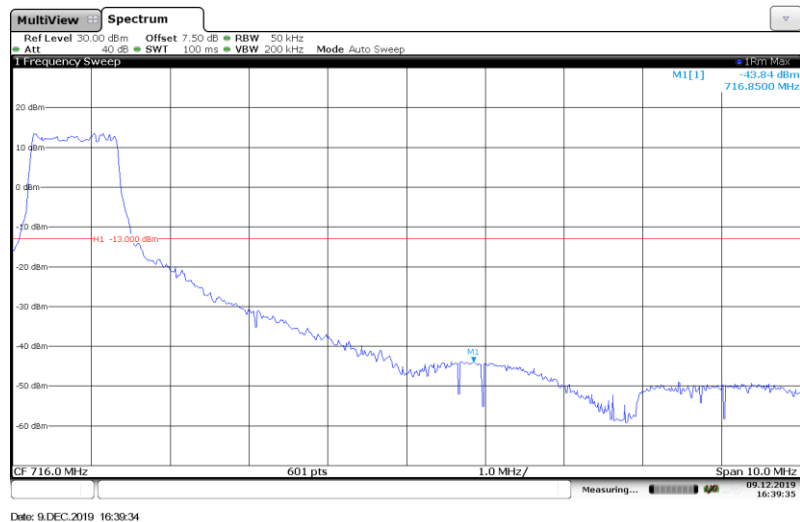
Band12-5MHz-16QAM-23155-Full RB#
