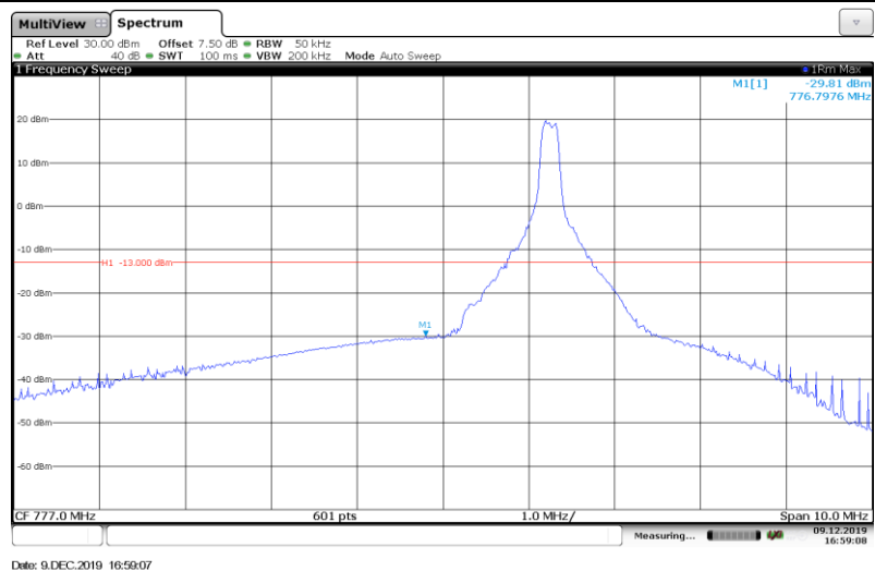
Band13-5MHz-16QAM-23205-1RB#
