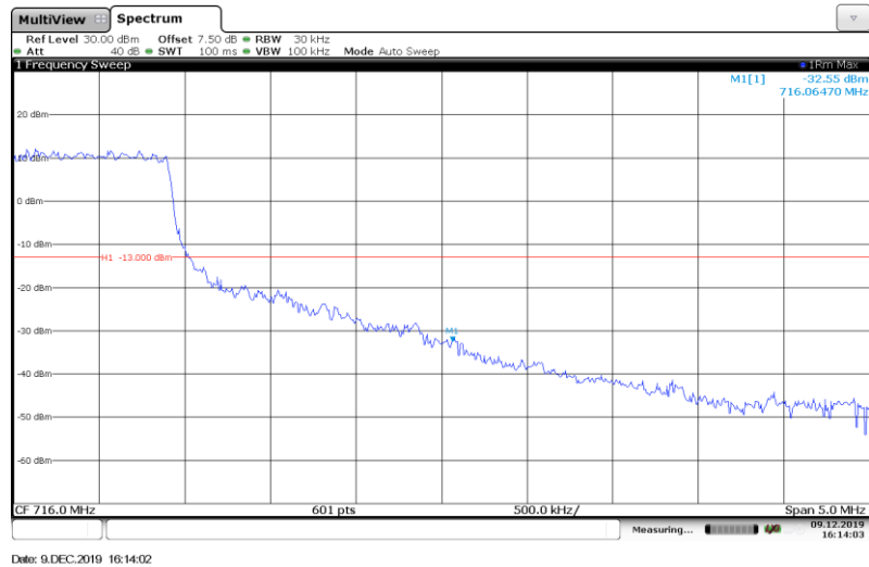
Band12-3MHz-16QAM-23165-Full RB#
