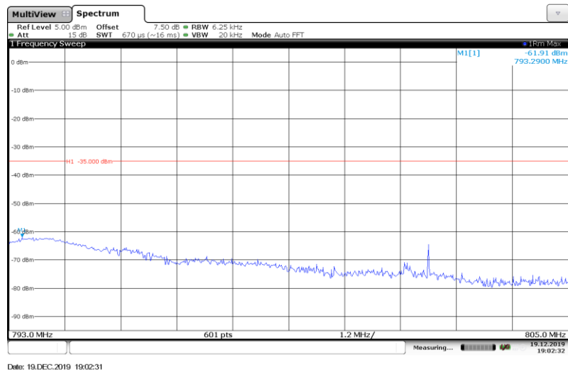
Band13-5MHz-16QAM-(793-805MHz)-1RB#
