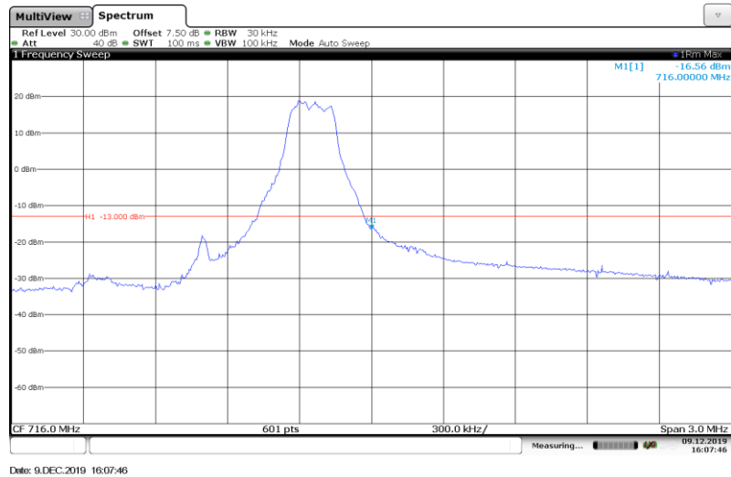
Band12-1.4MHz-16QAM-23173-1RB#
