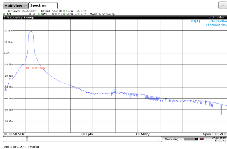
Band13-5MHz-QPSK-23255-1RB#
