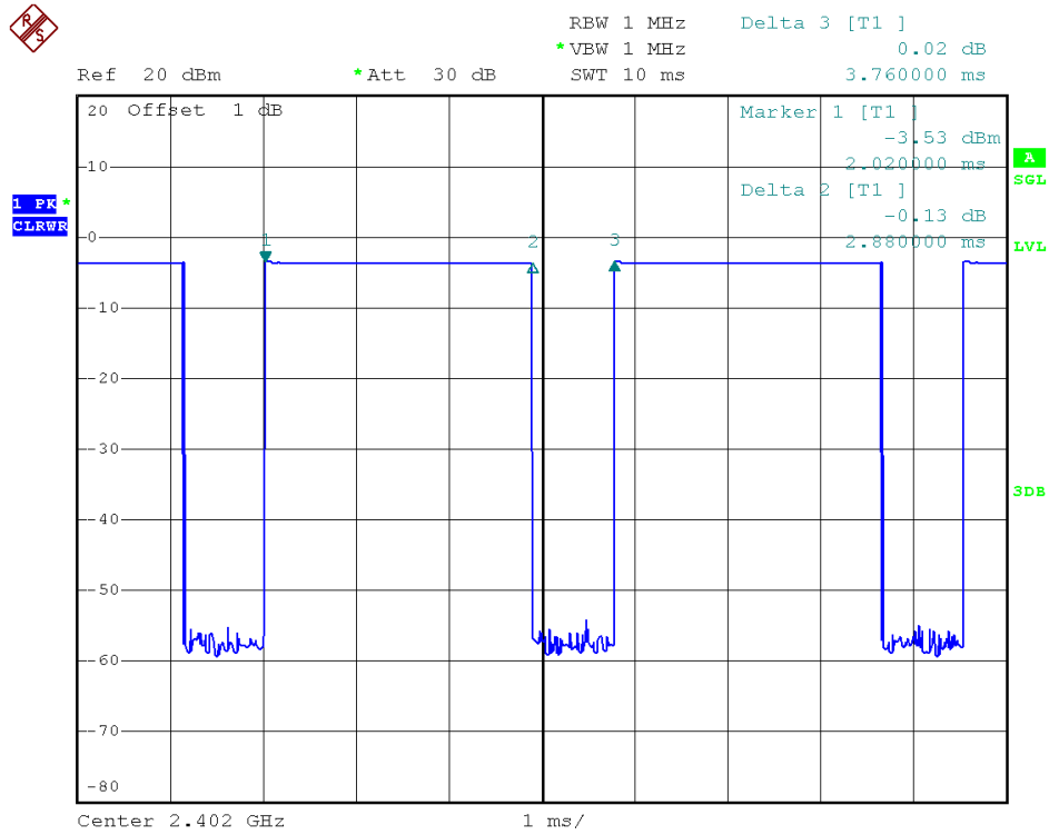
0 Channel @ DH5
