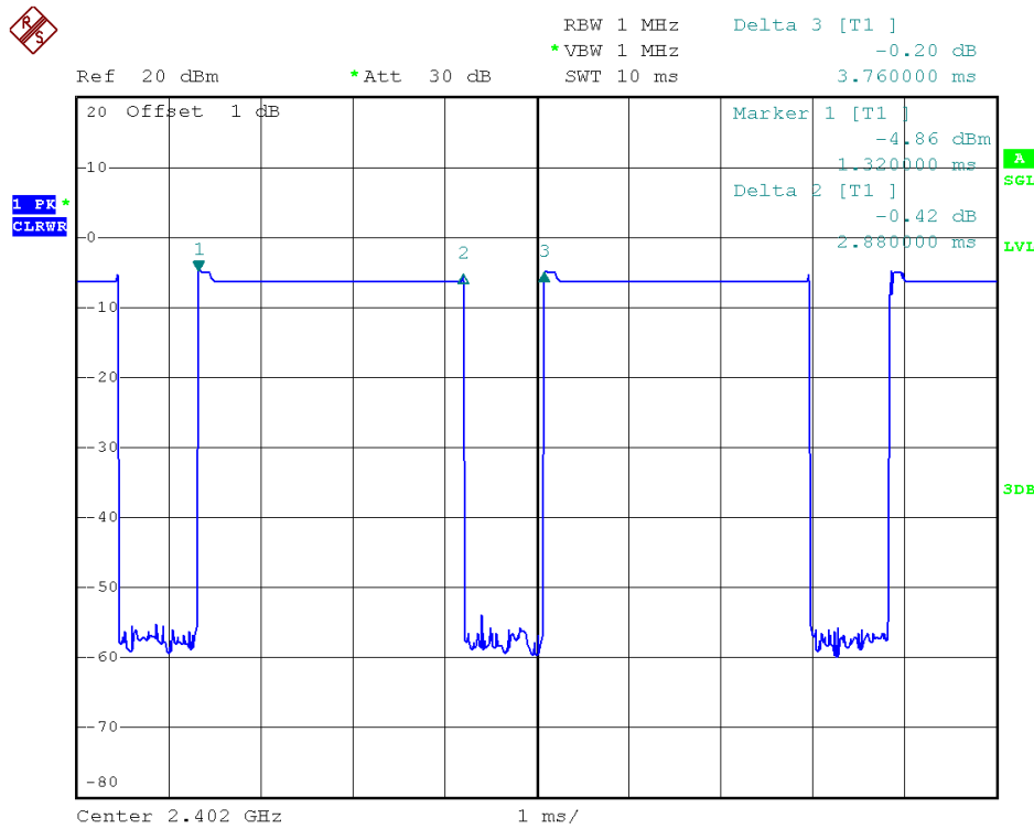
0 Channel @ 3DH5
