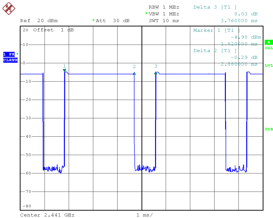
39 Channel @ 3DH5
