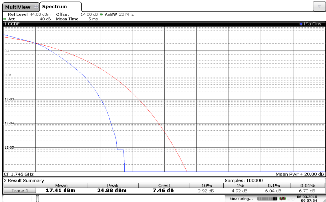
(Plot A6: Band 4/20MHz/16QAM in Ch.20300 100RB Size)
