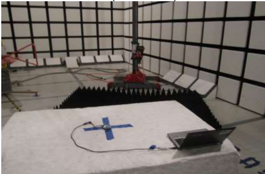
RADIATED BACK PHOTO (ABOVE 1 GHz)
