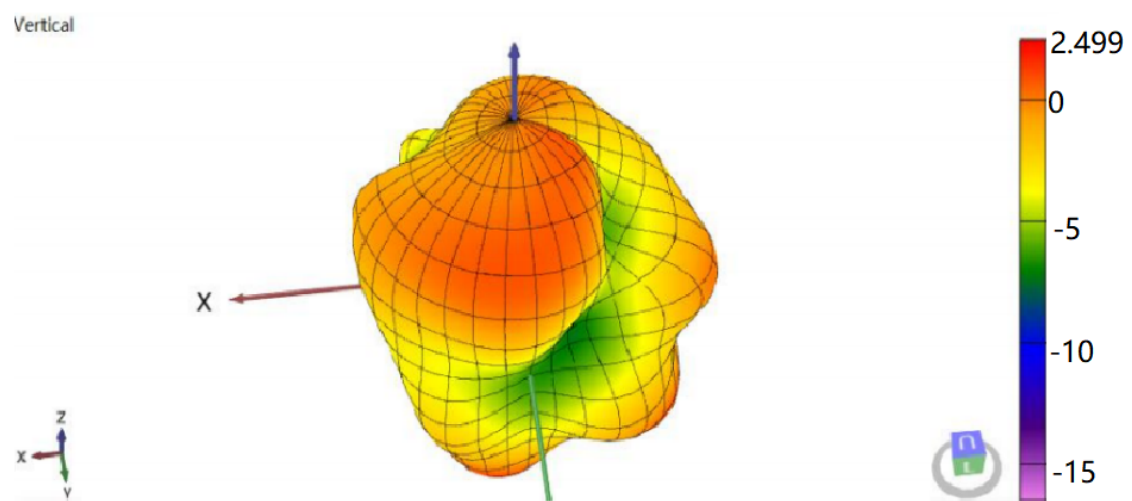
antenna 2480MHz 3D-Vertical Pattern
