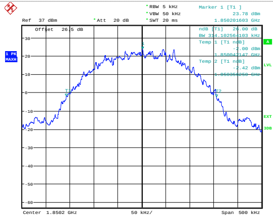
-26dB bandwidth
