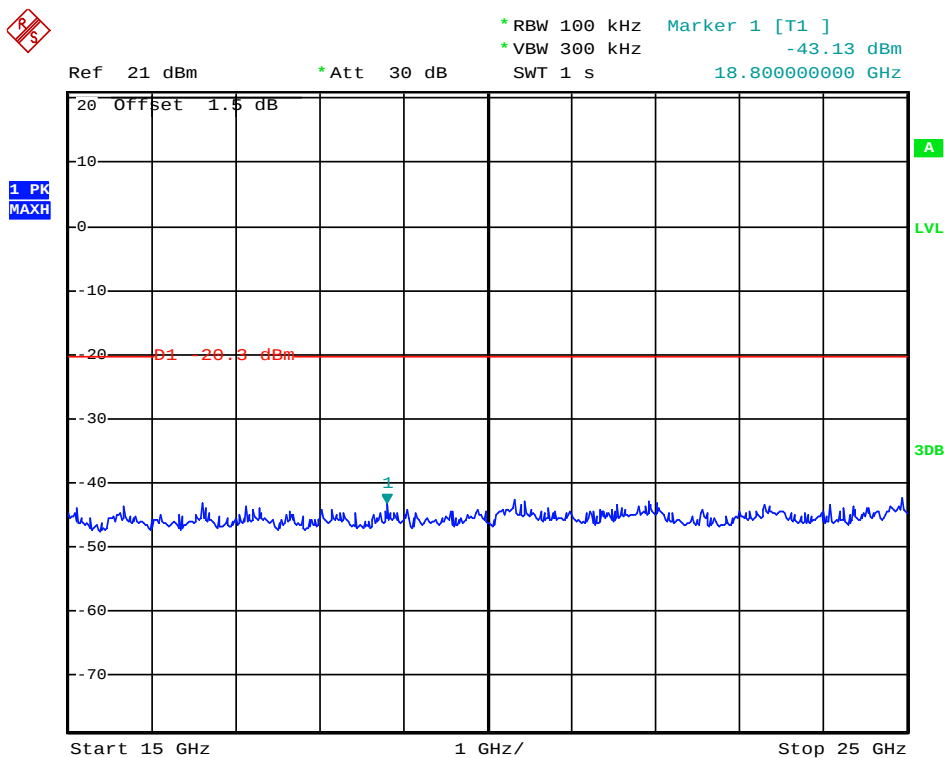
(Plot 4.9.2.C2: Channel 78: 2480MHz @ 8DPSK)
