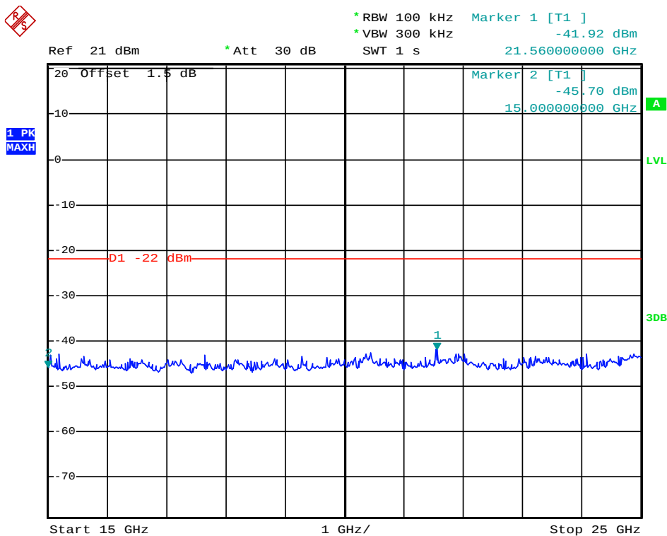
(Plot 4.9.3.A2: Channel 00: 2402MHz @ \pi/4 DQPSK)
