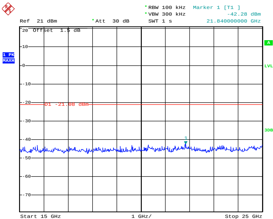
(Plot 4.9.2.A2: Channel 00: 2402MHz @ 8DPSK)
