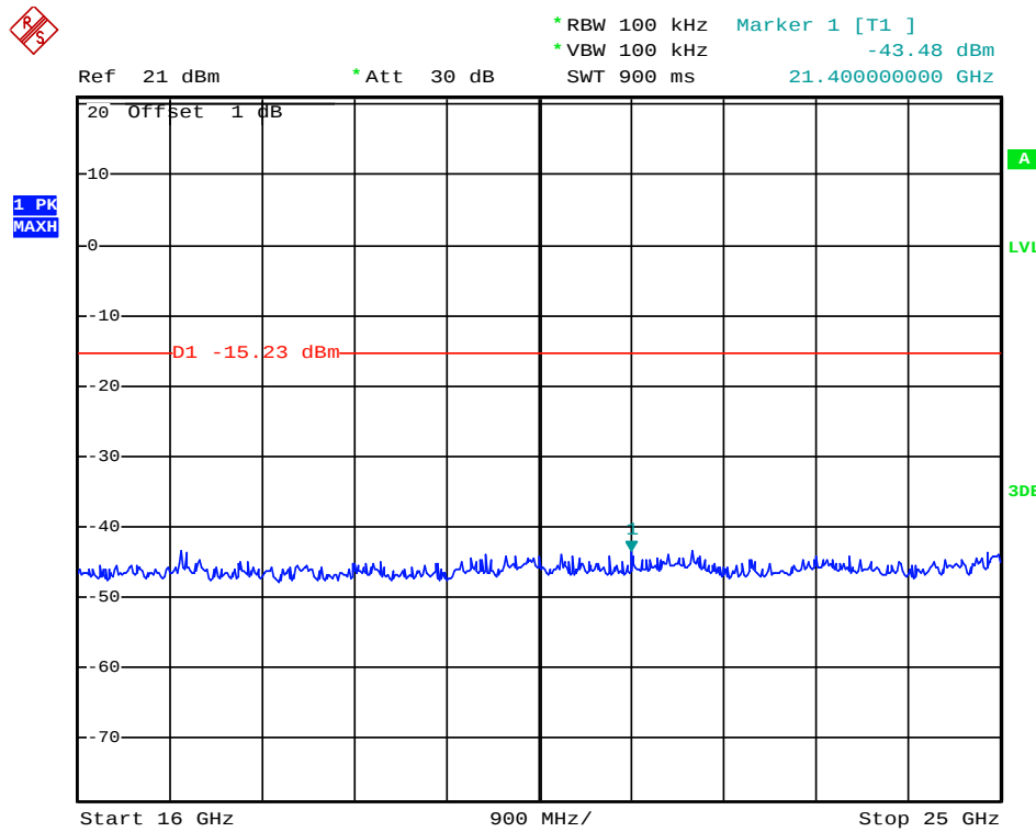
(Plot 4.9.3.B3: Channel 39: 2441MHz @ \pi/4 DQPSK)
