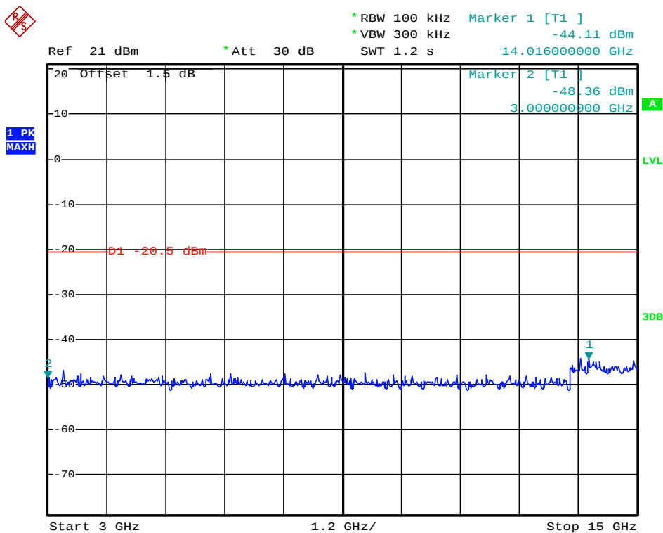
(Plot 4.9.3.B1: Channel 39: 2441MHz @ \pi/4 DQPSK)
