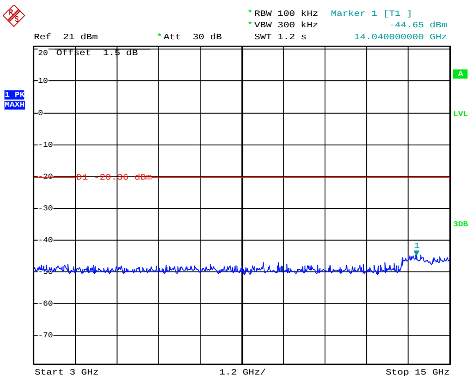
(Plot 4.9.2.B1: Channel 39: 2441MHz @ 8DPSK)
