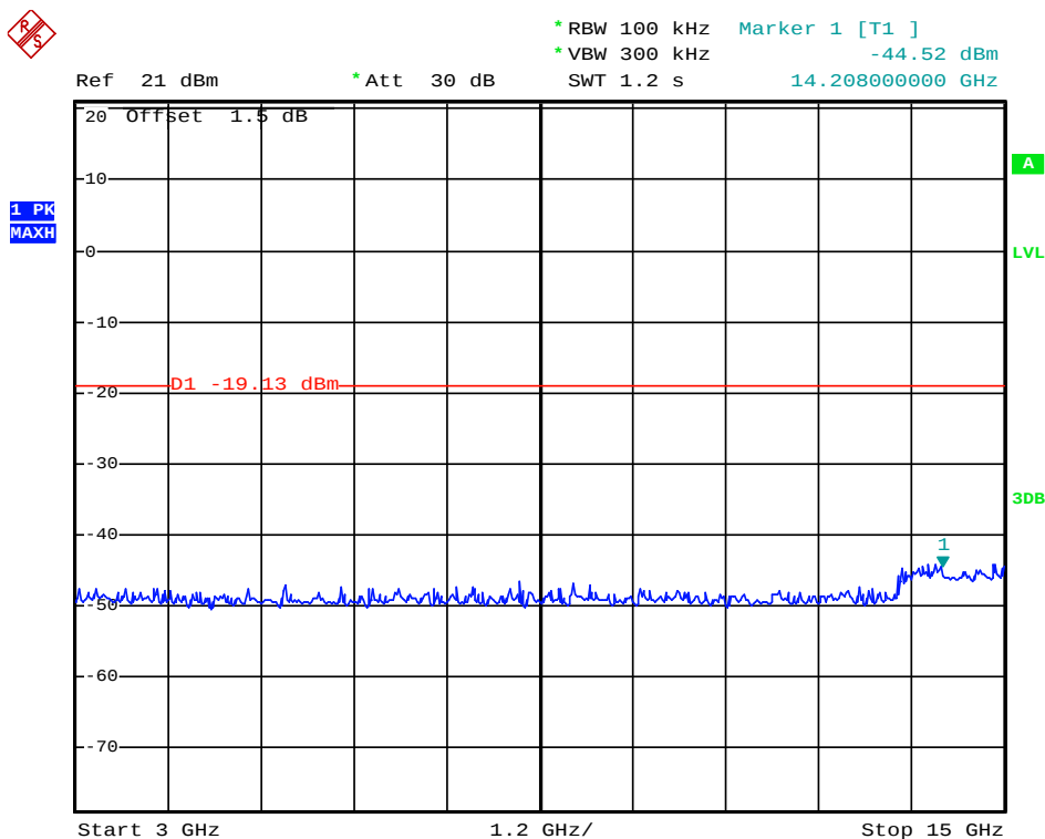
(Plot 4.9.3.C1: Channel 78: 2480MHz @ \pi/4 DQPSK)
