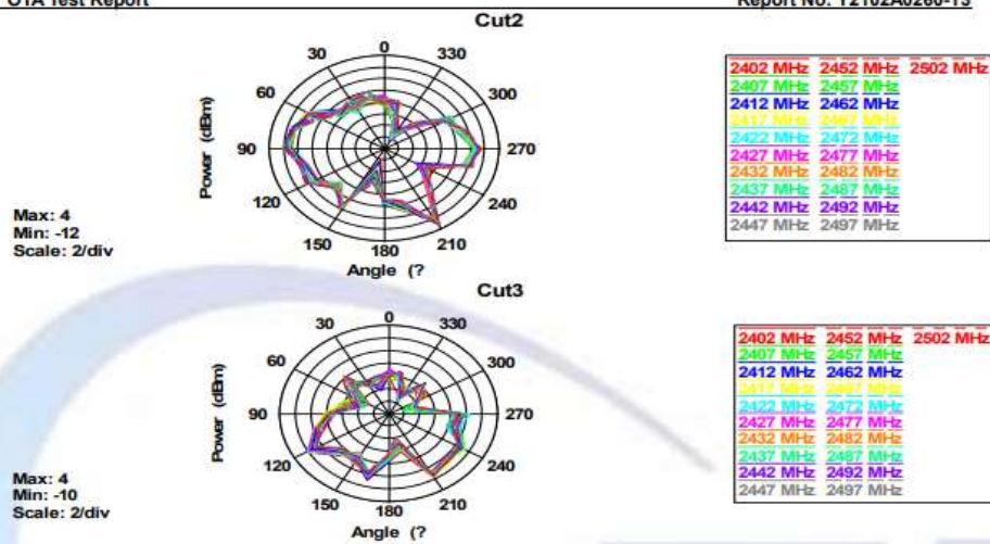
2402MHz ~2502 MHz Wi-Fi 2.4G 3D Gain
