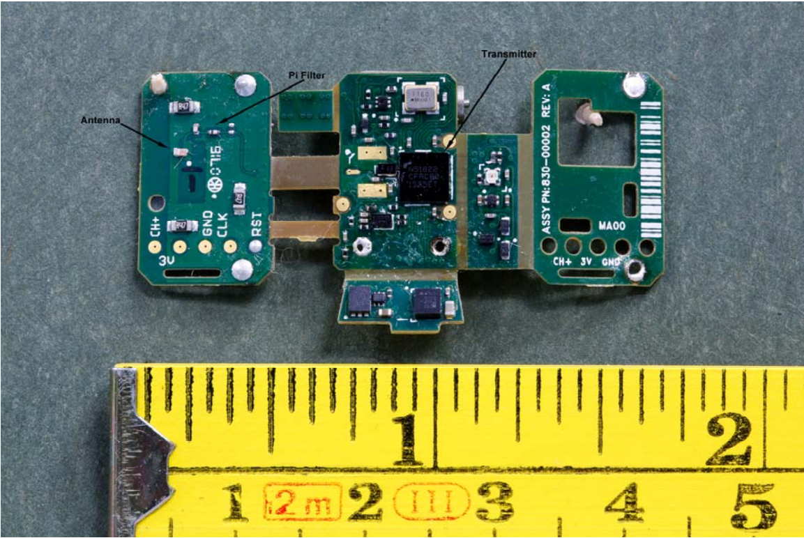
PCB Front
